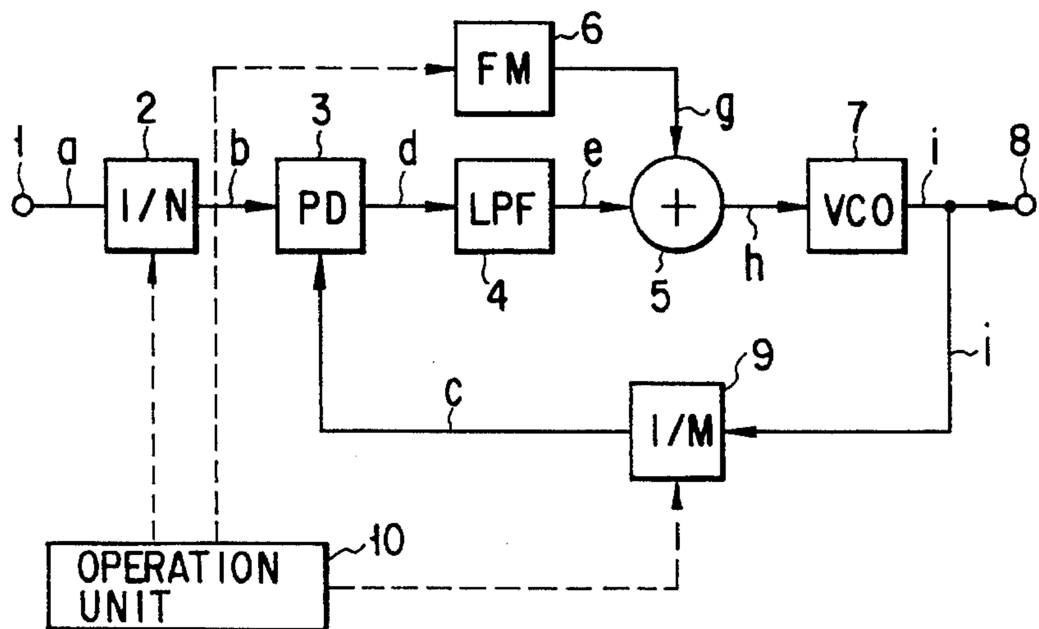
FIG. 5 (PRIOR ART)
