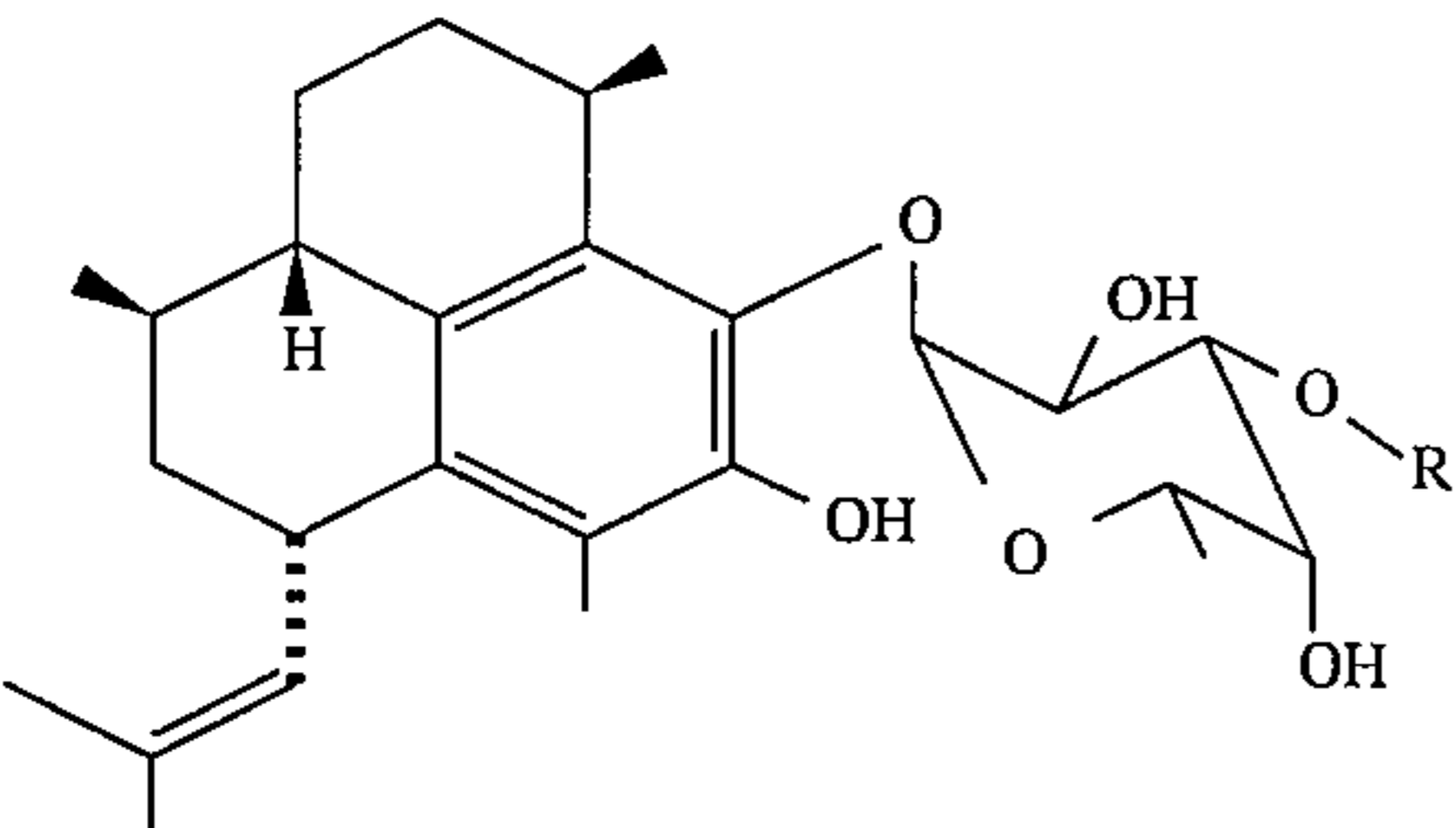
(13) R = H (Pseudopterisin K)
