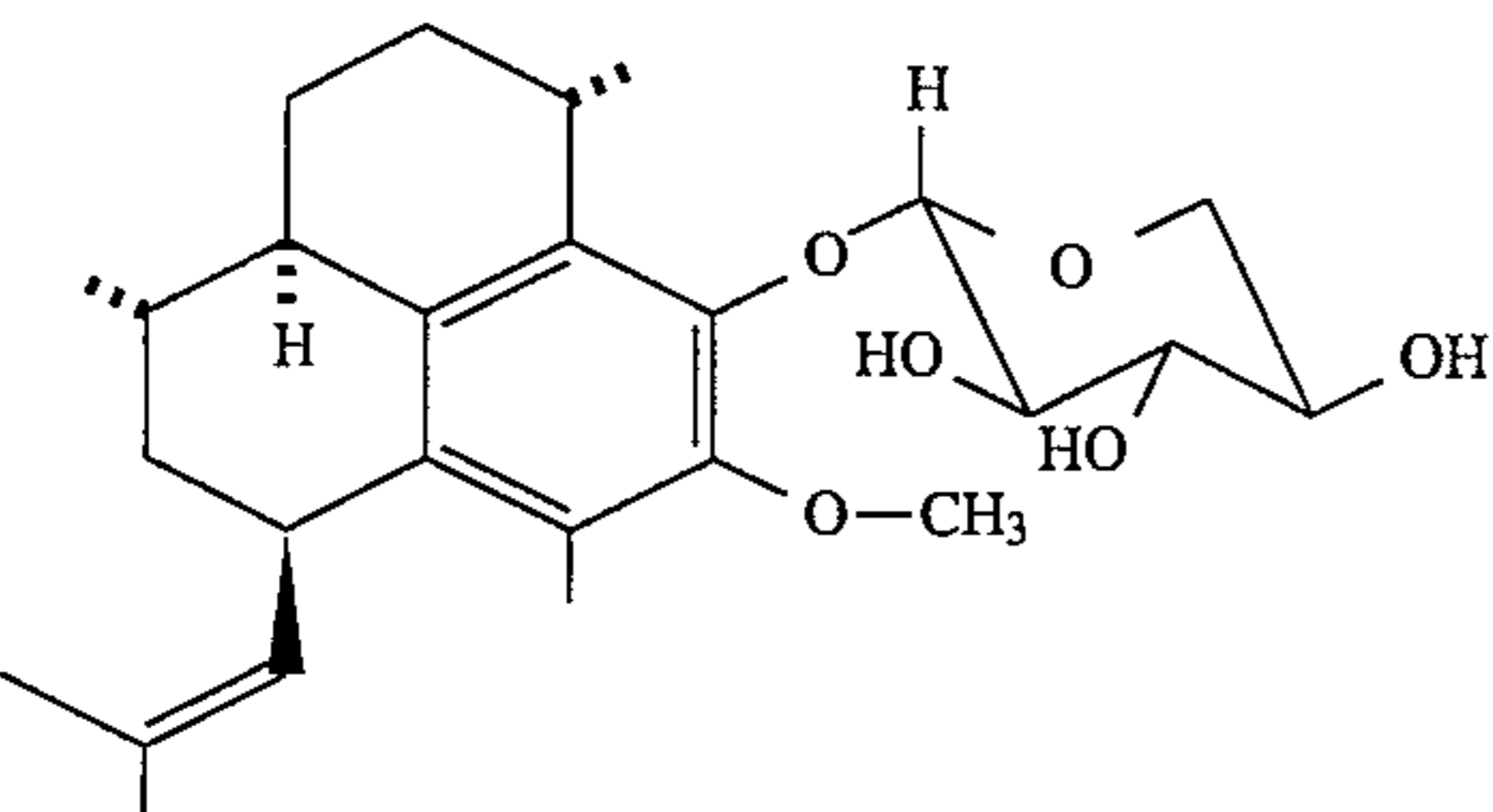
(15) Pseudopterisin A Methyl Ether
