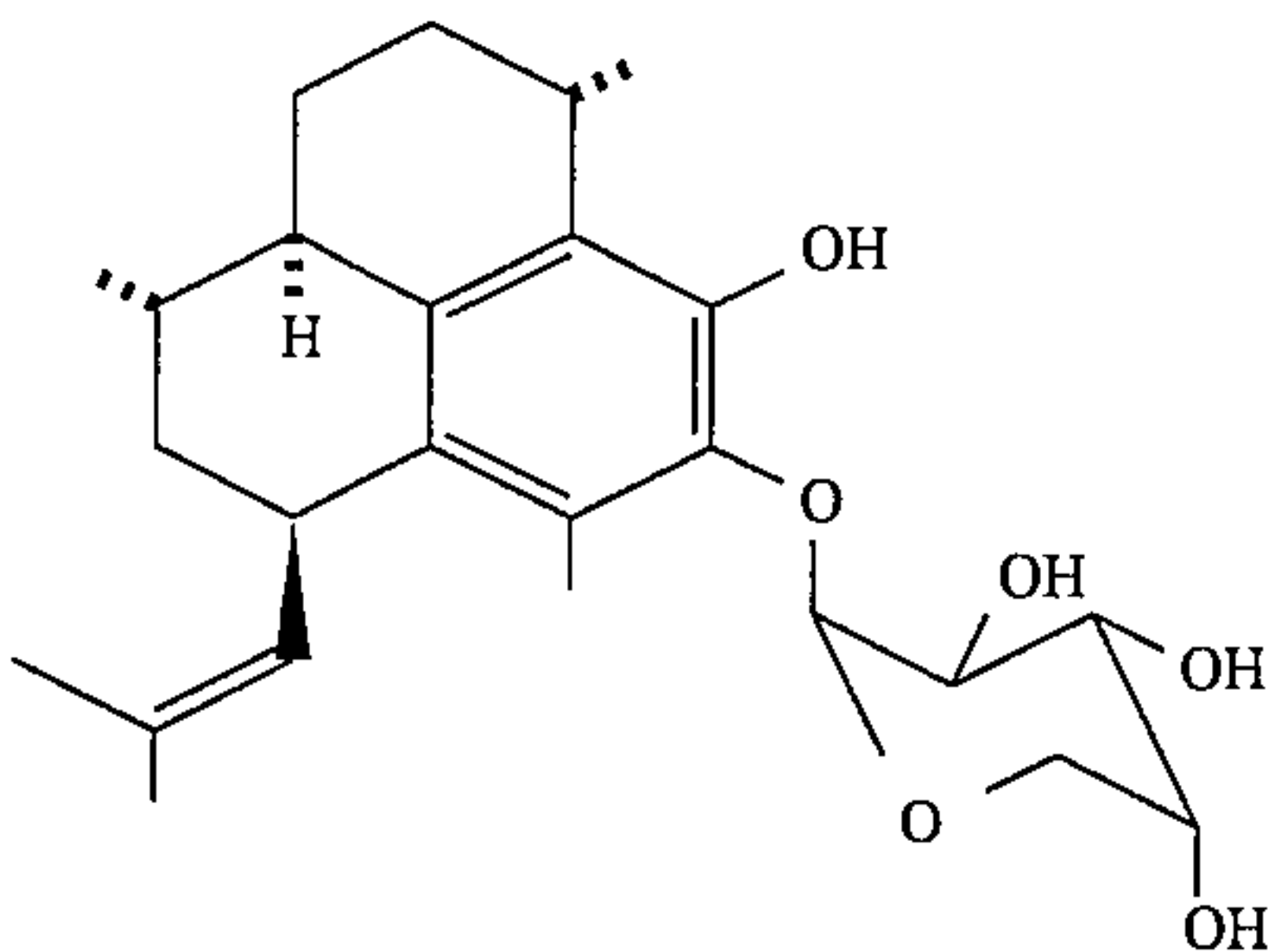
(7) (Pseudopteriosin F)
