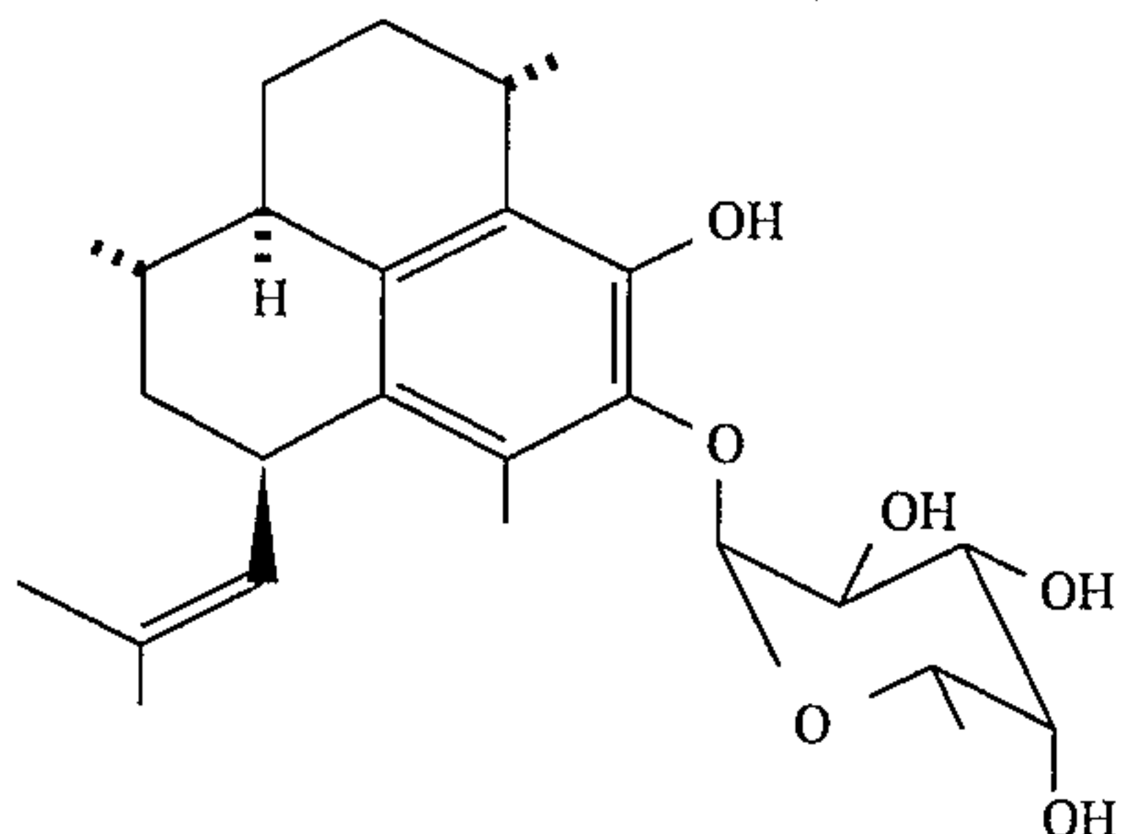
(6) (Pseudopteriosin E)
