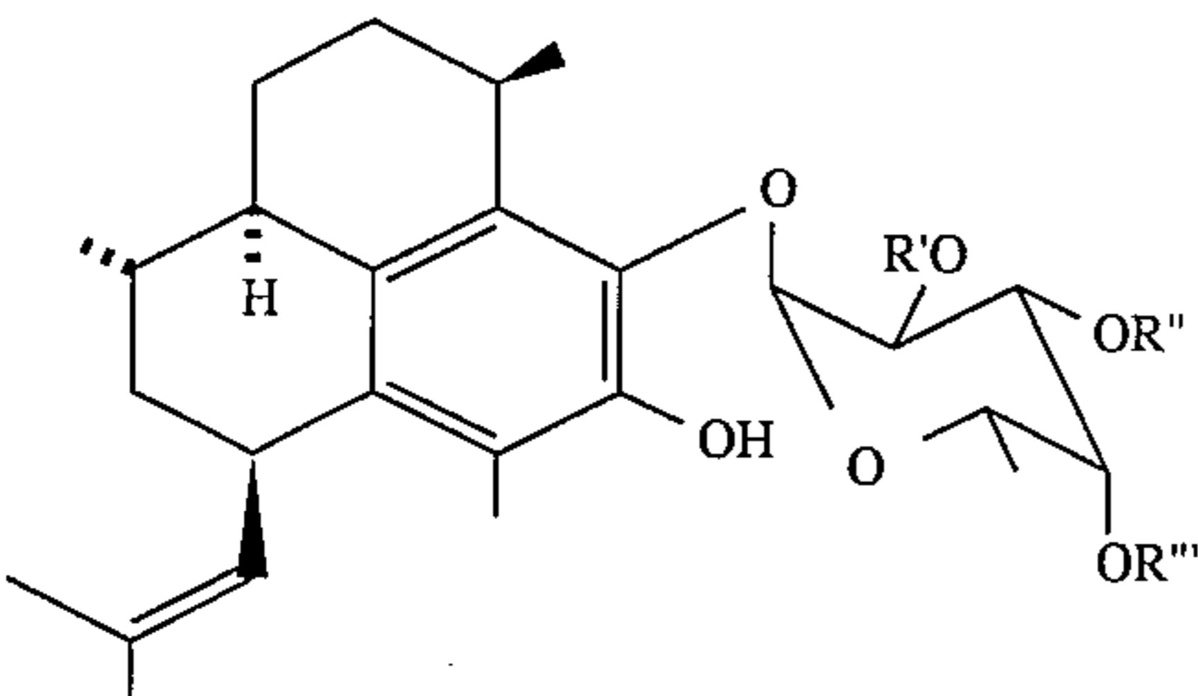
(8) R', R'' and R''' = H (Pseudopterisin G)
