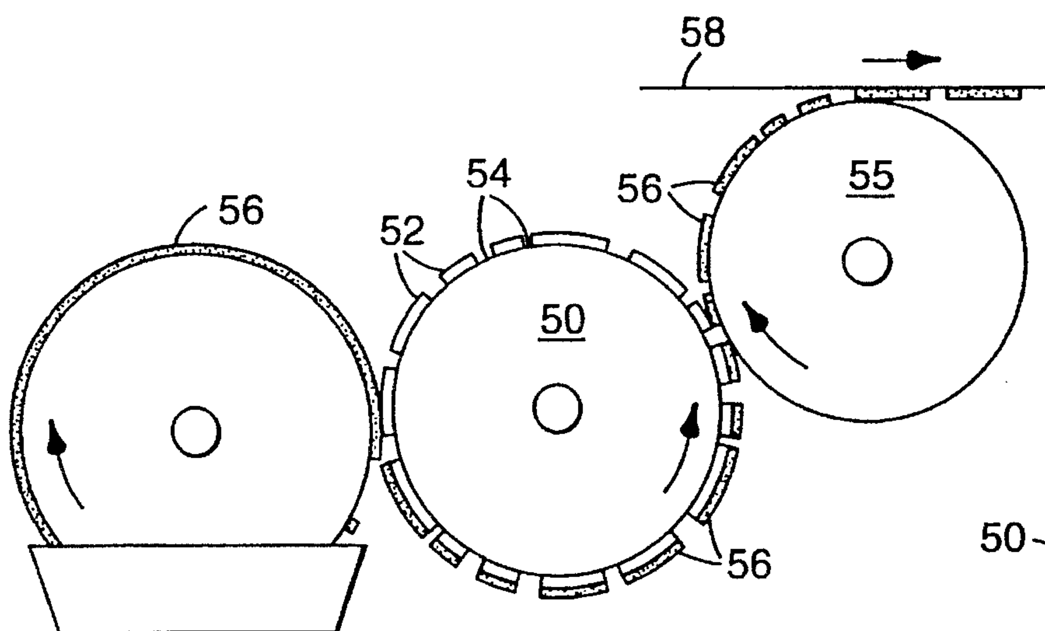
Fig. 4 PRIOR ART
