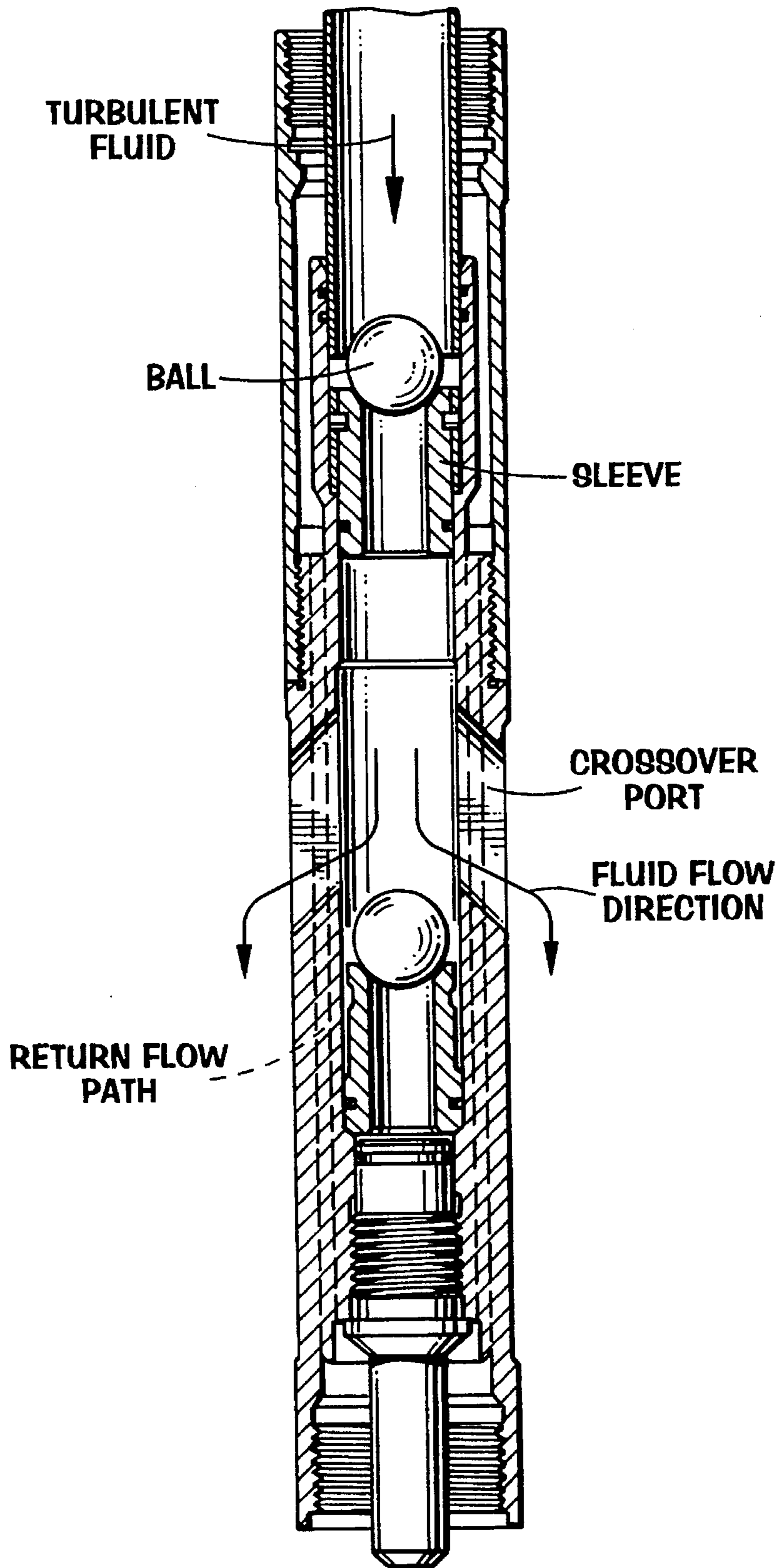
FIG. 1 (PRIOR ART)
