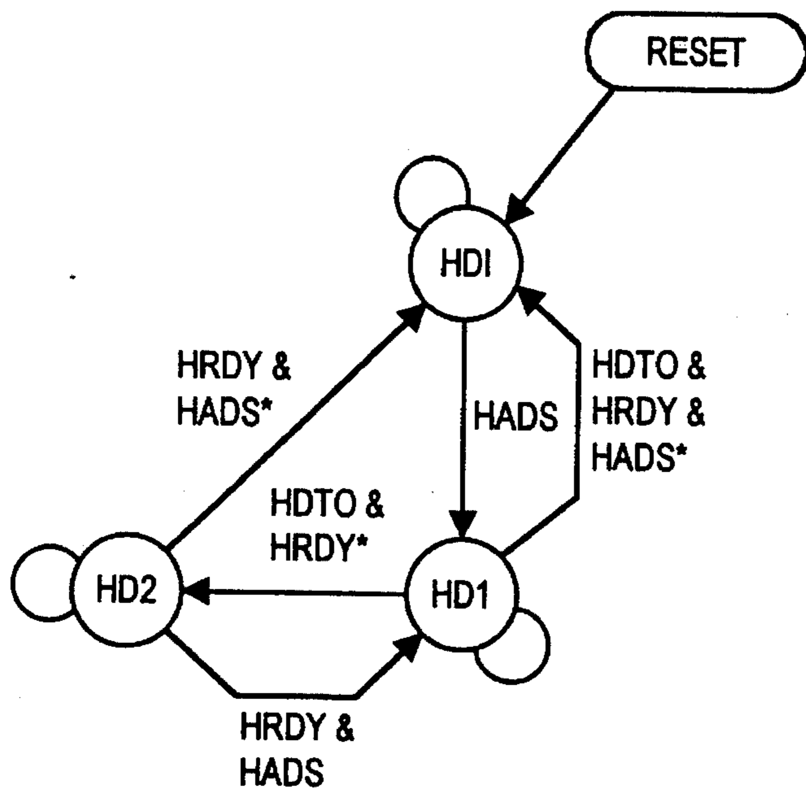
HDAT STATE MACHINE
