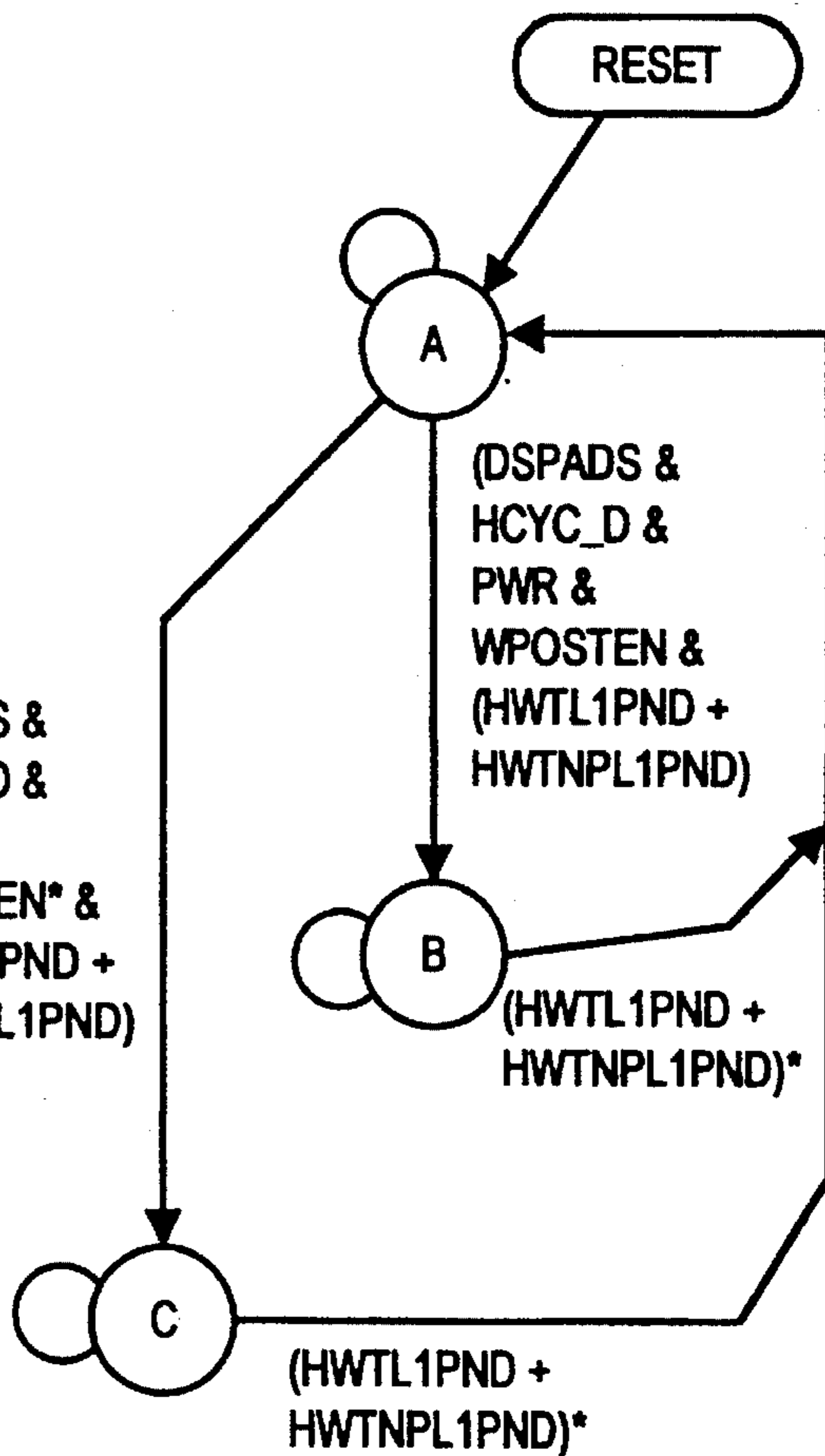
HWL2PND STATE MACHINE
