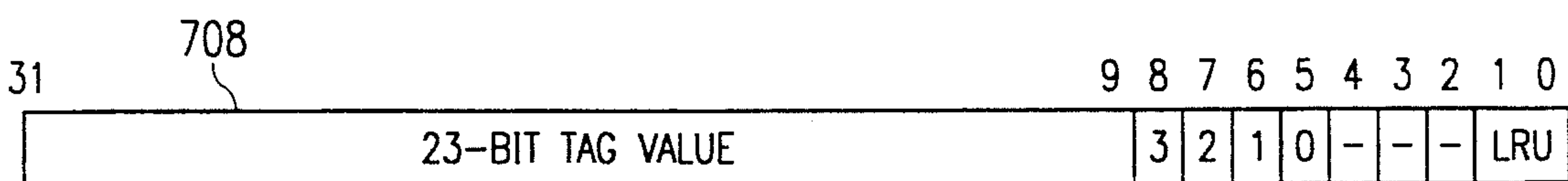
FIG. 35 SUB-BLOCK PRESENT BITS
