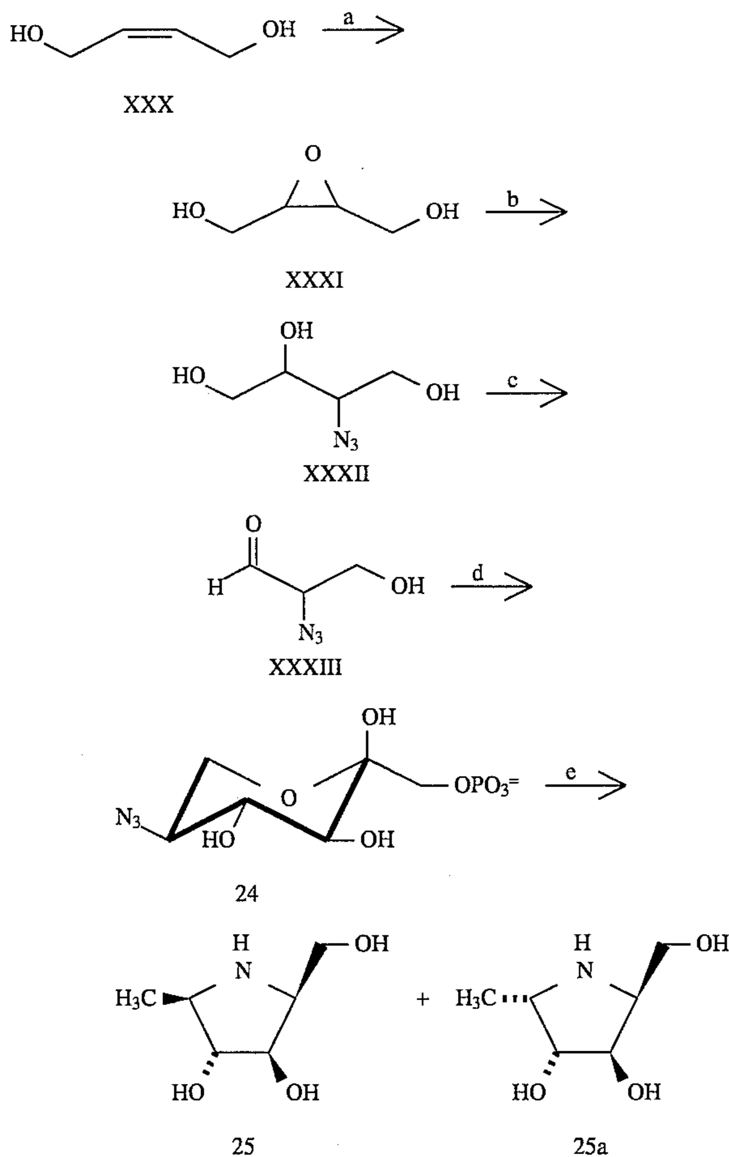
Scheme 10
