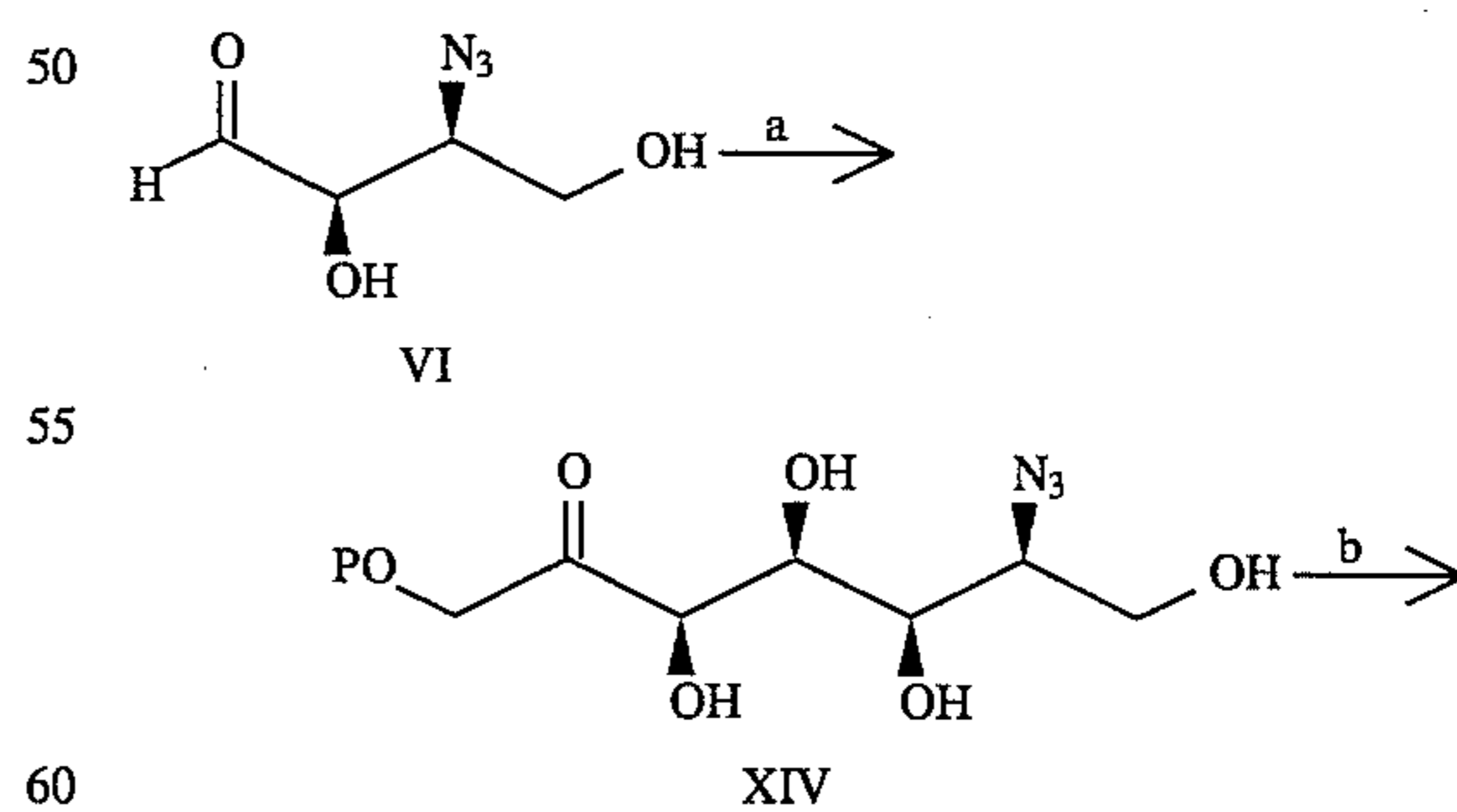
Scheme 5
