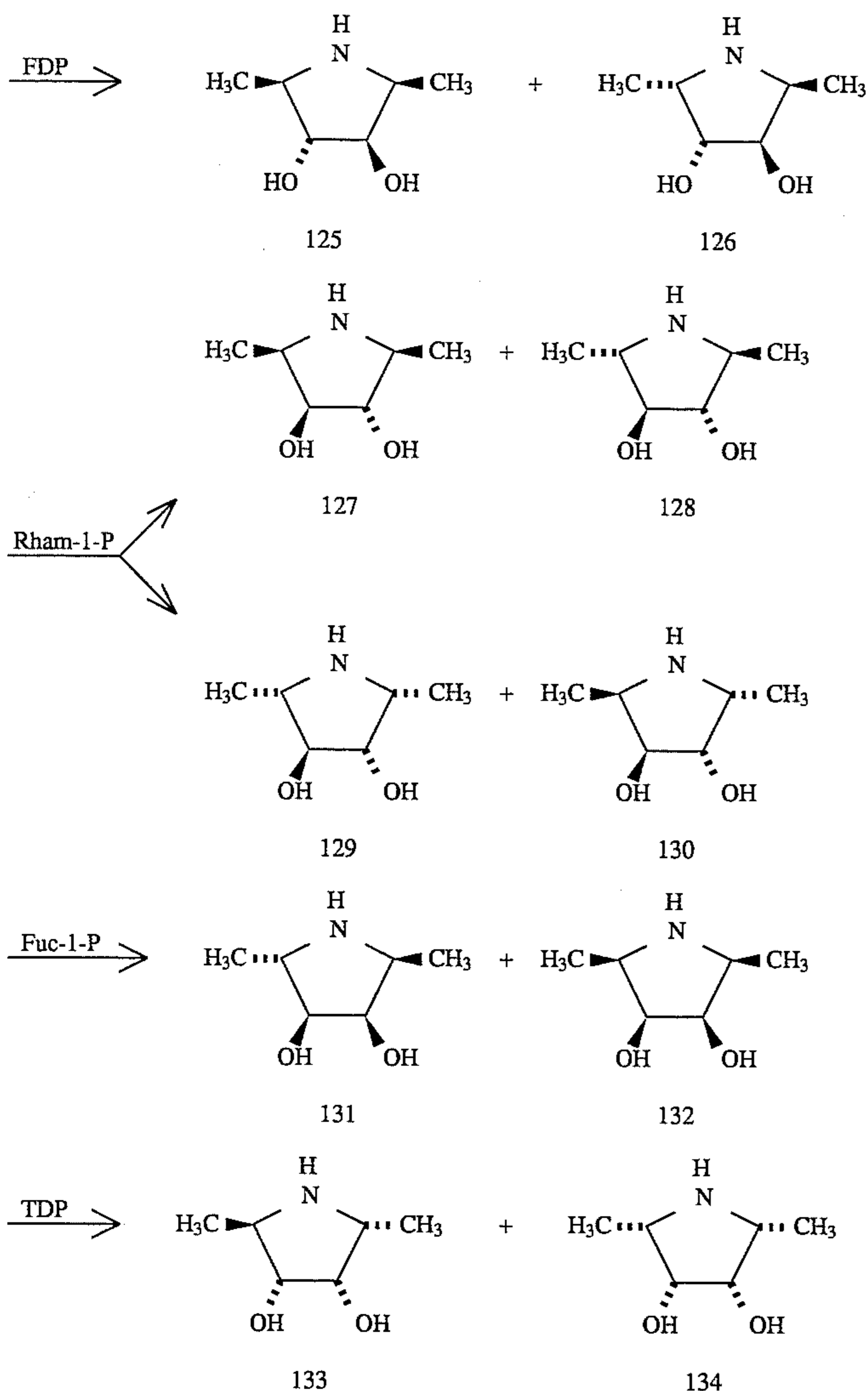
Scheme 12
