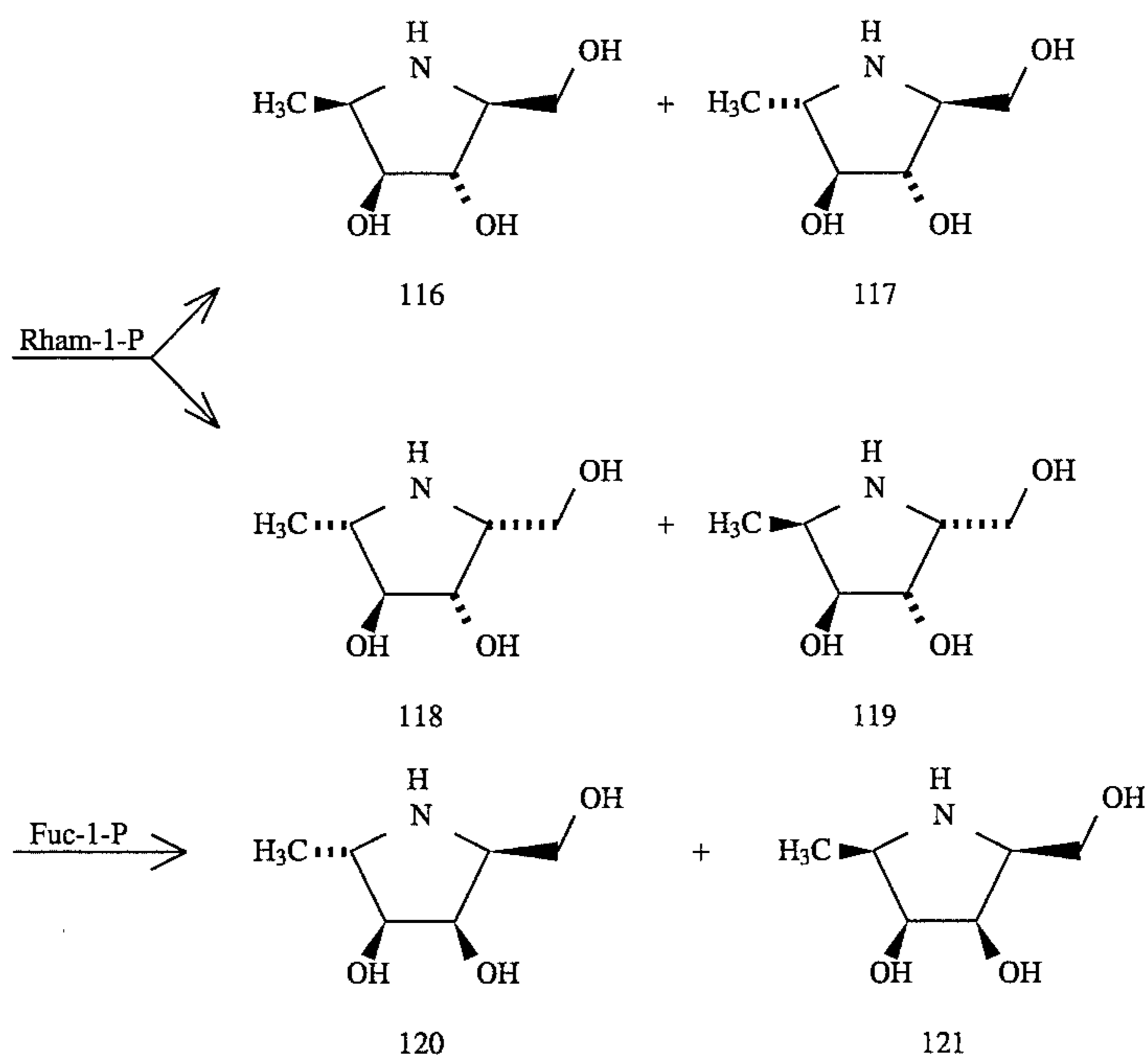
Scheme 11
