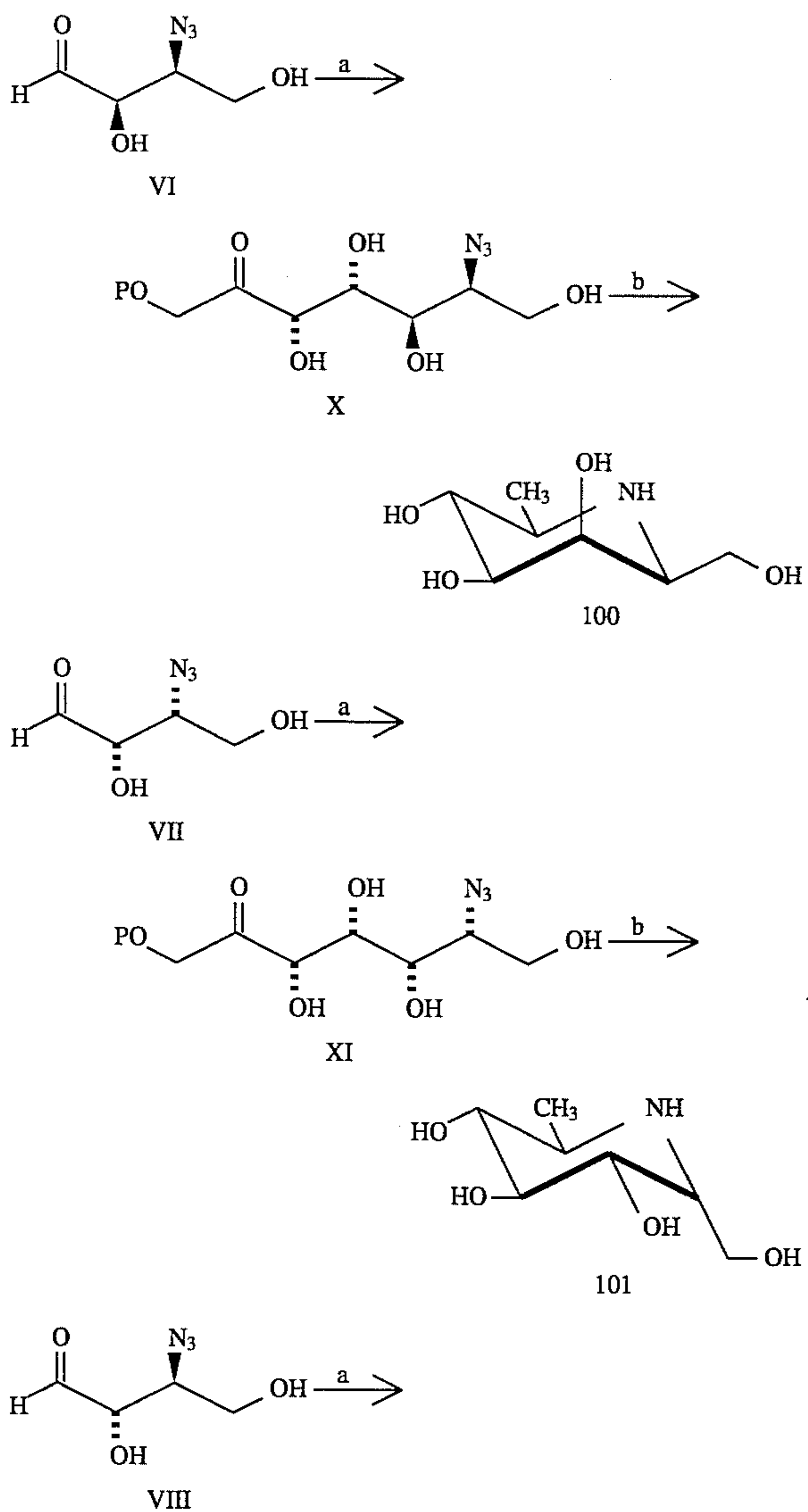
Scheme 4
