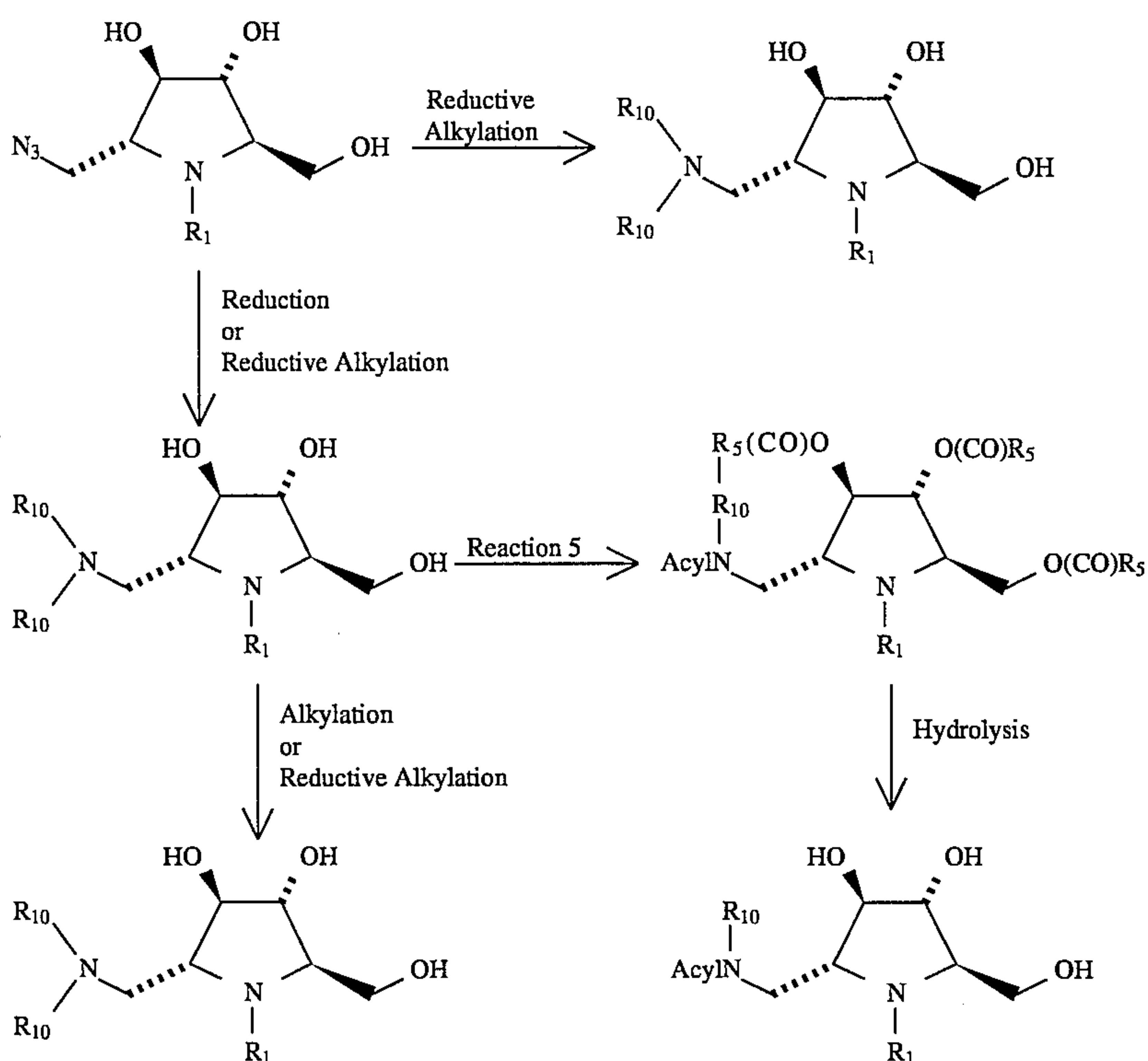
Scheme 6
