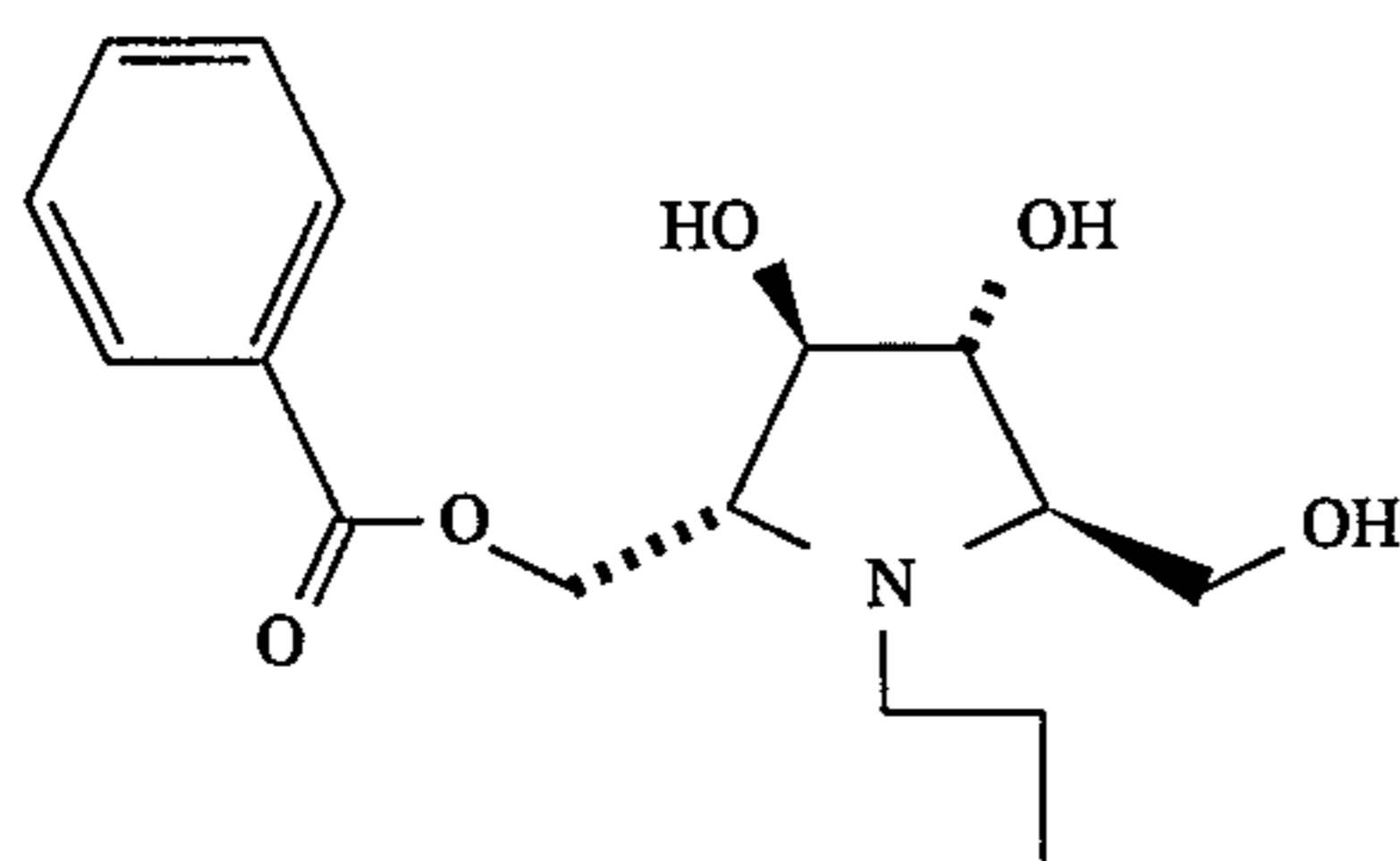
2,5-(Butylimino)-2,5-dideoxy-D-mannitol, 1-benzoate
