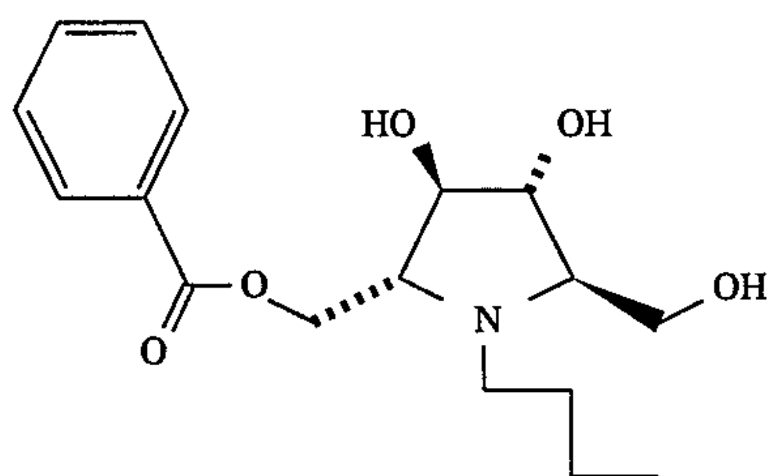
2,5-(Butylimino)-2,5-dideoxy-D-mannitol, 1-benzoate
