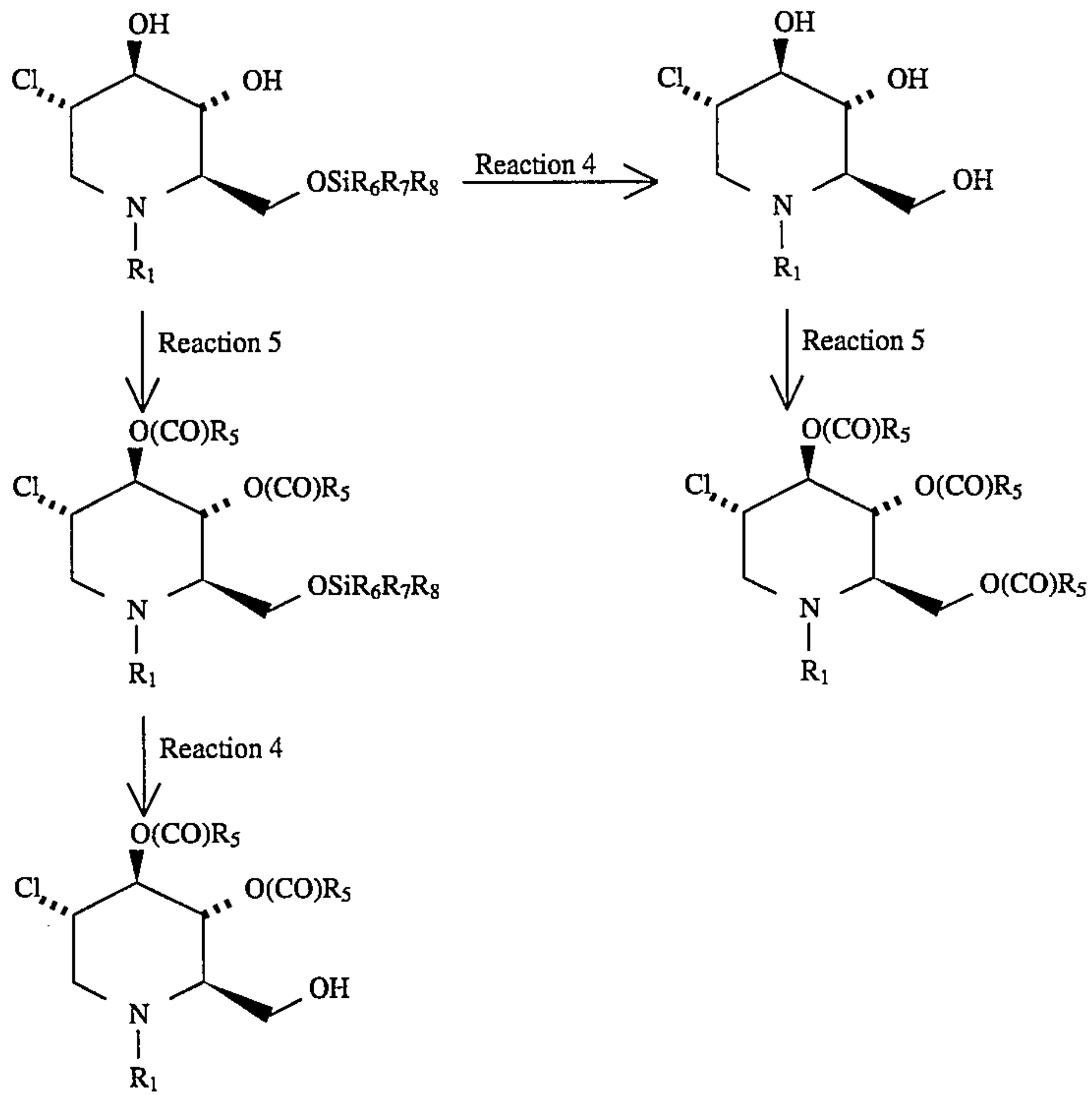
Scheme 2
