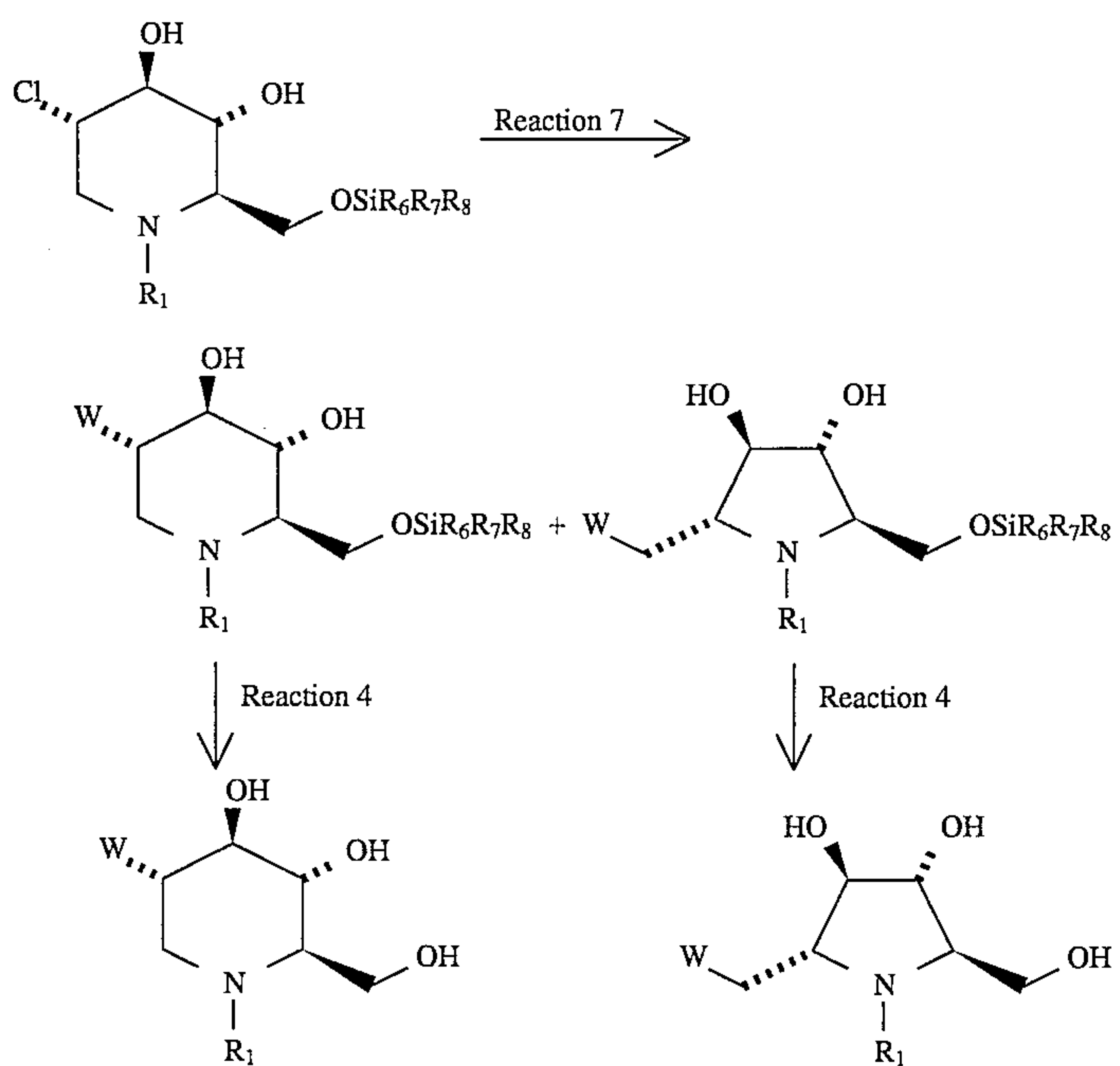
Scheme 5
