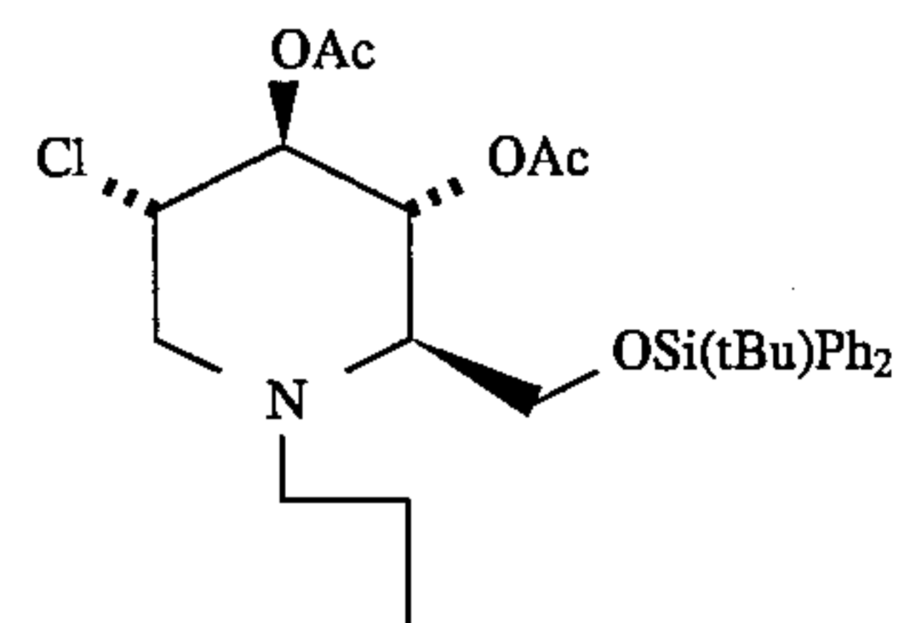
1,5-(Butylimino)-2-chloro-1,2,5-trideoxy-6-O-[(1,1-dimethylethyl)diphenylsilyl]-D-glucitol, diacetate
