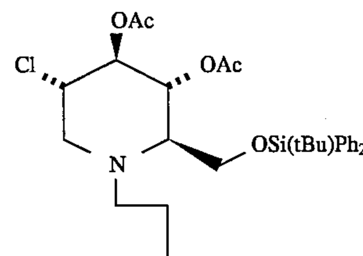
1,5-(Butylimino)-2-chloro-1,2,5-trideoxy-6-O-[(1,1-dimethylethylethyl)diphenylsilyl]-D-glucitol, diacetate
