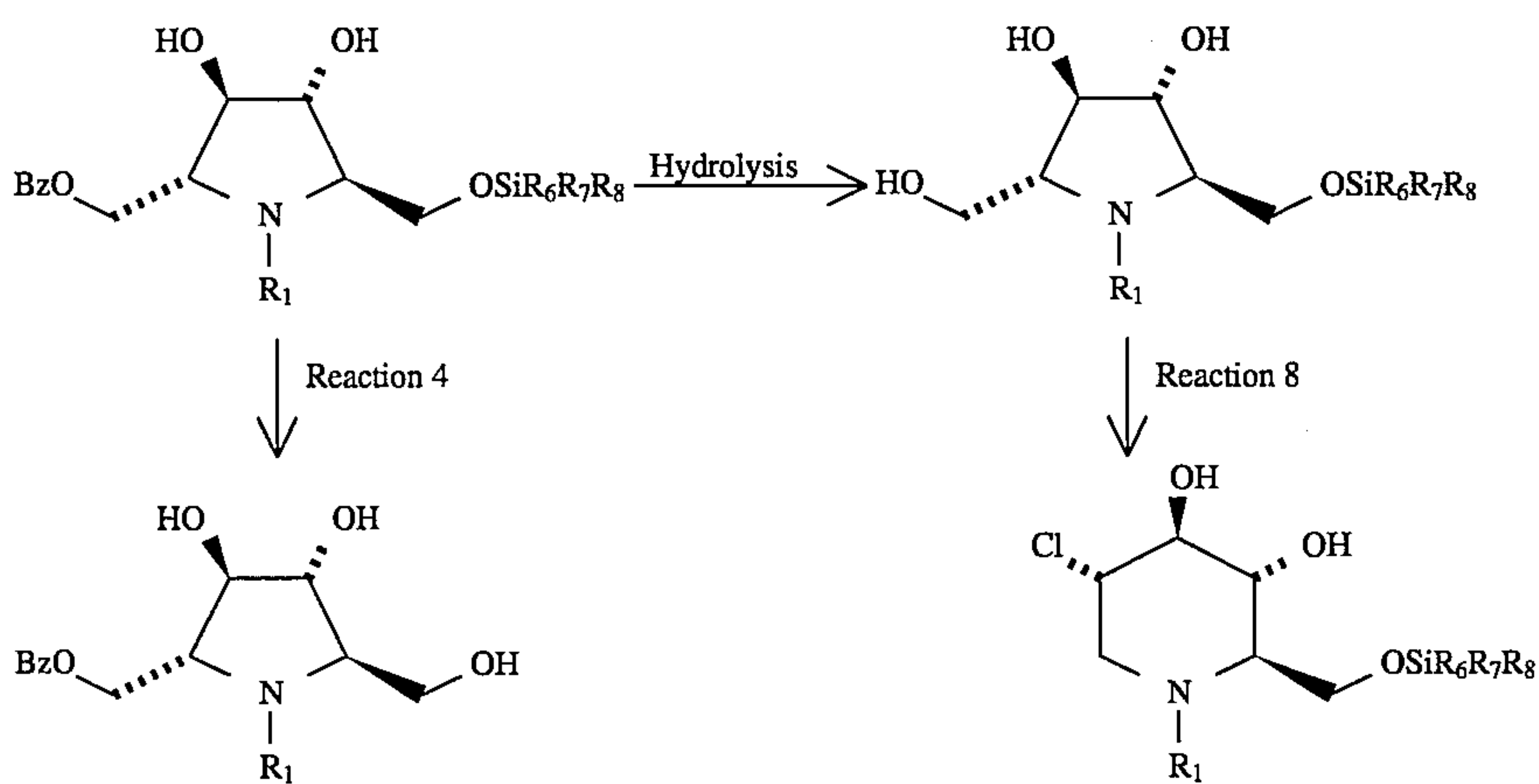
Scheme 7
