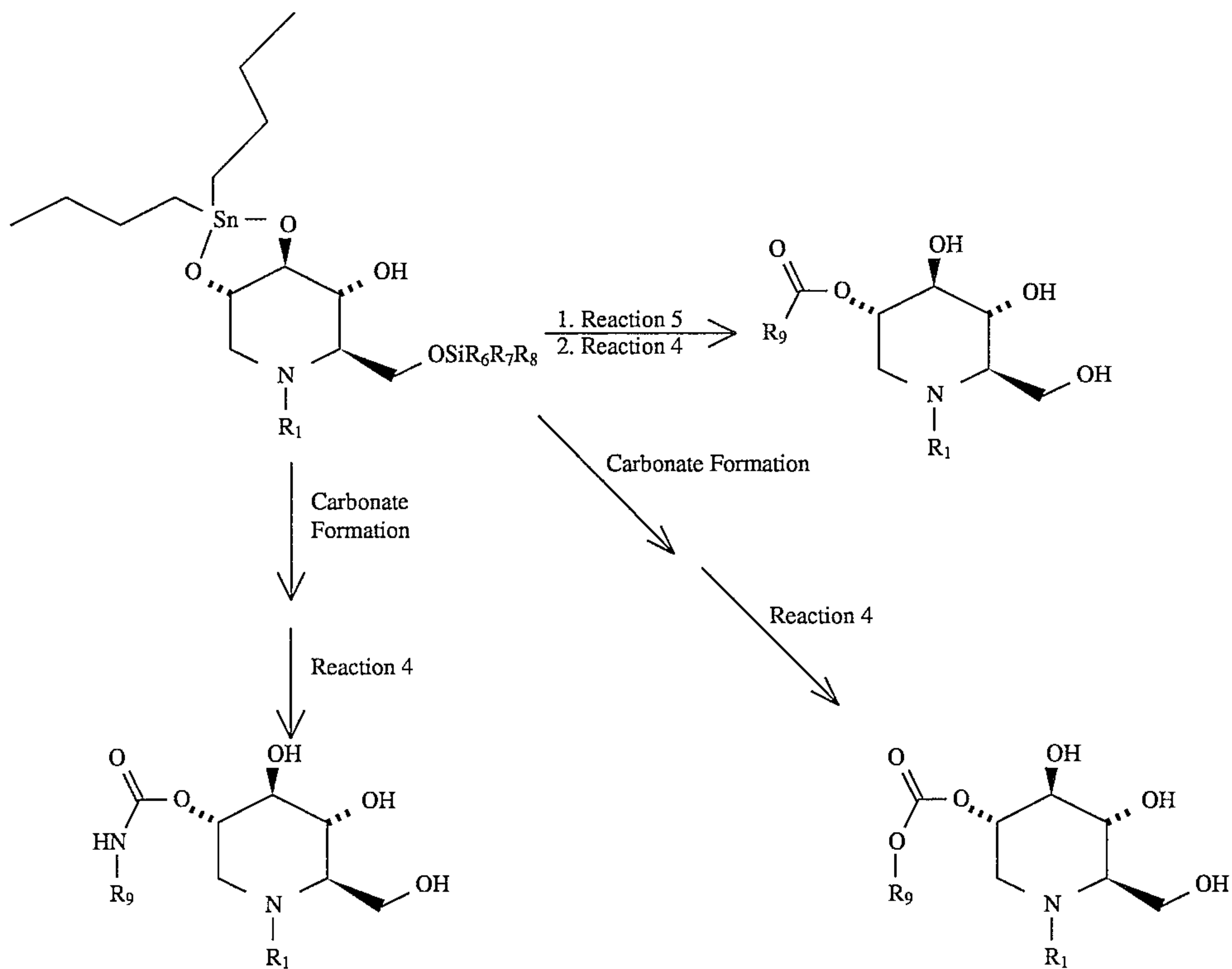
Scheme 4
