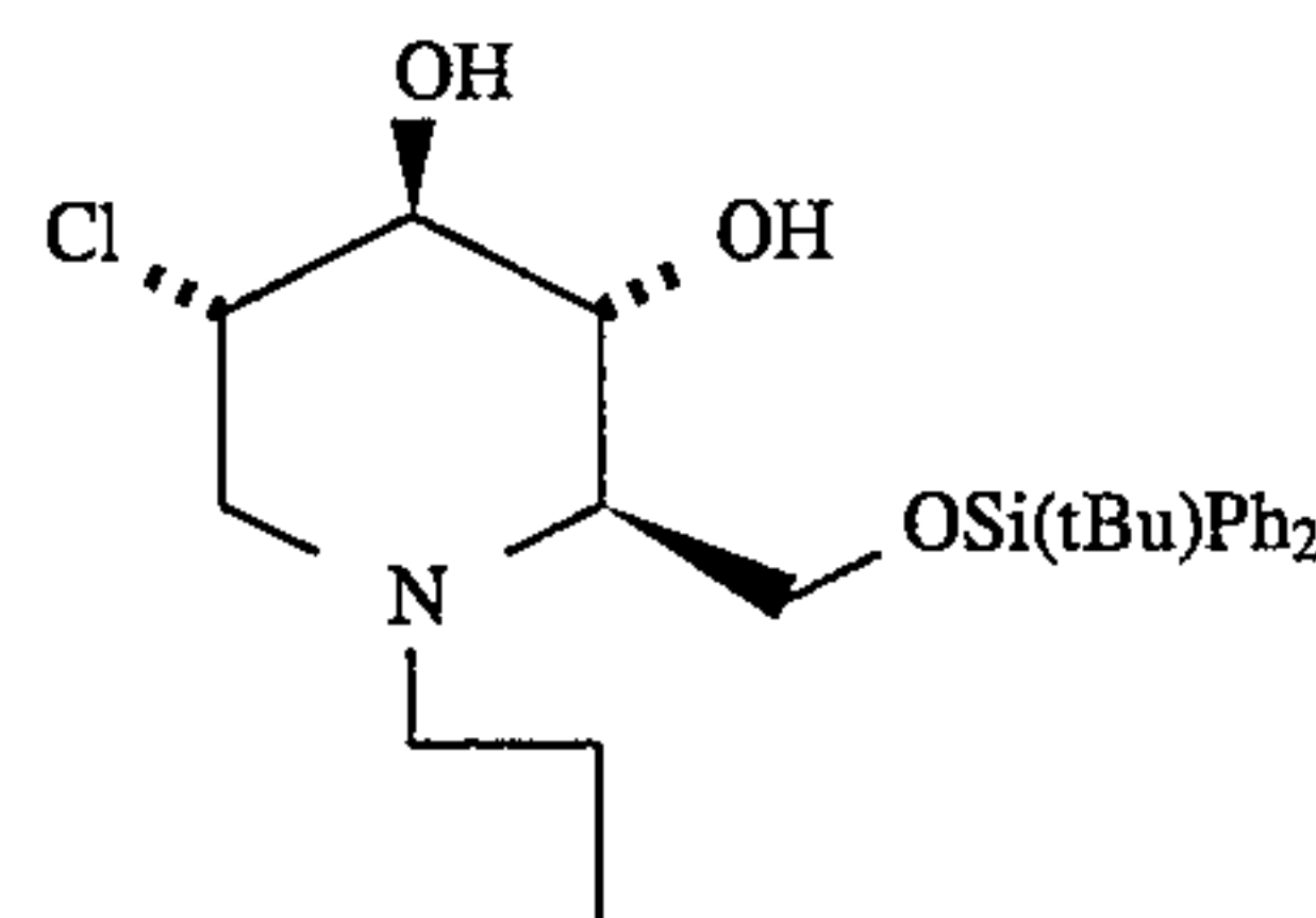
1,5-(Butylimino)-2-chloro-1,2,5-trideoxy-6-O-[(1,1-dimethylethyl)diphenylsilyl]-D-glucitol
