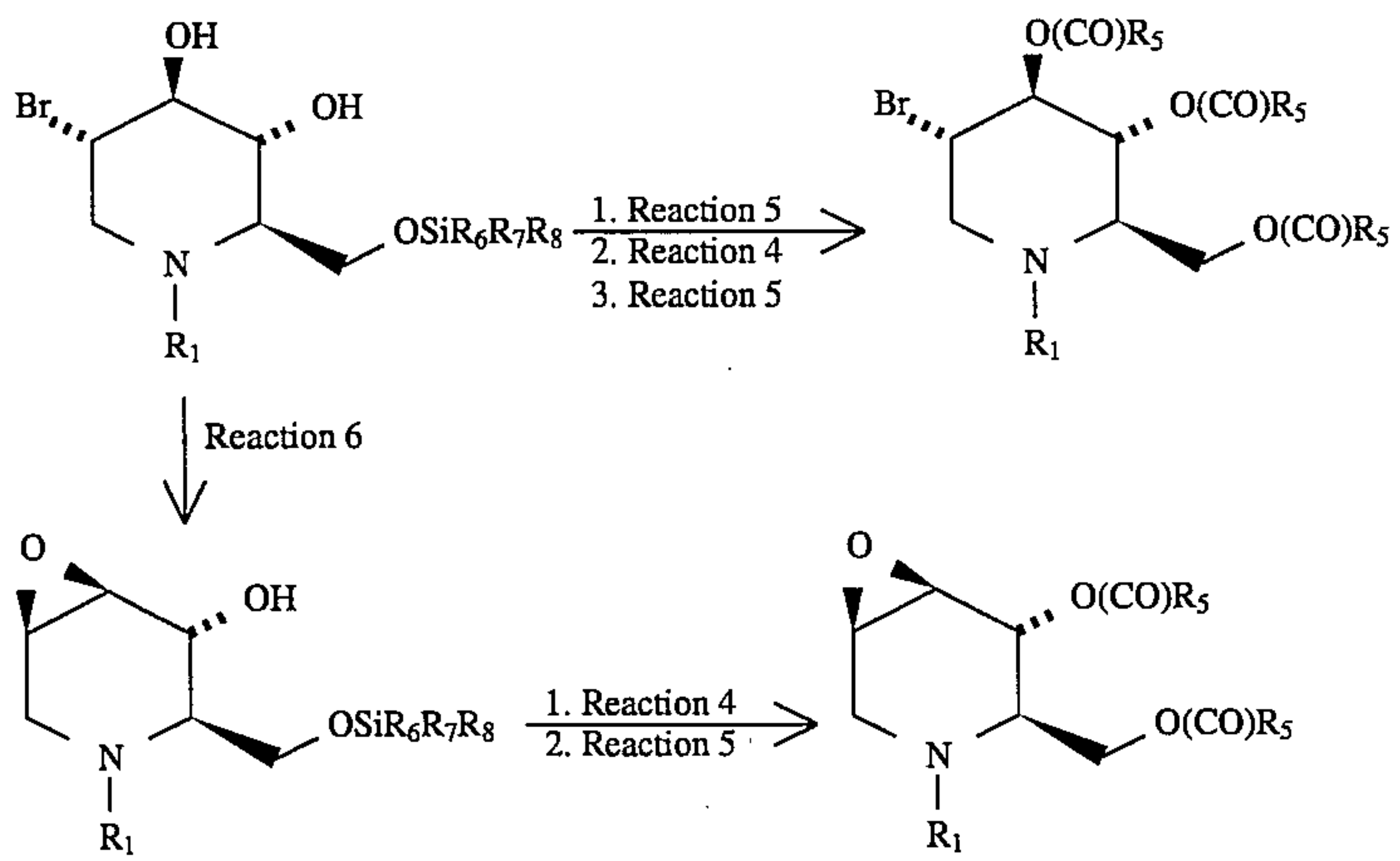
Scheme 3
