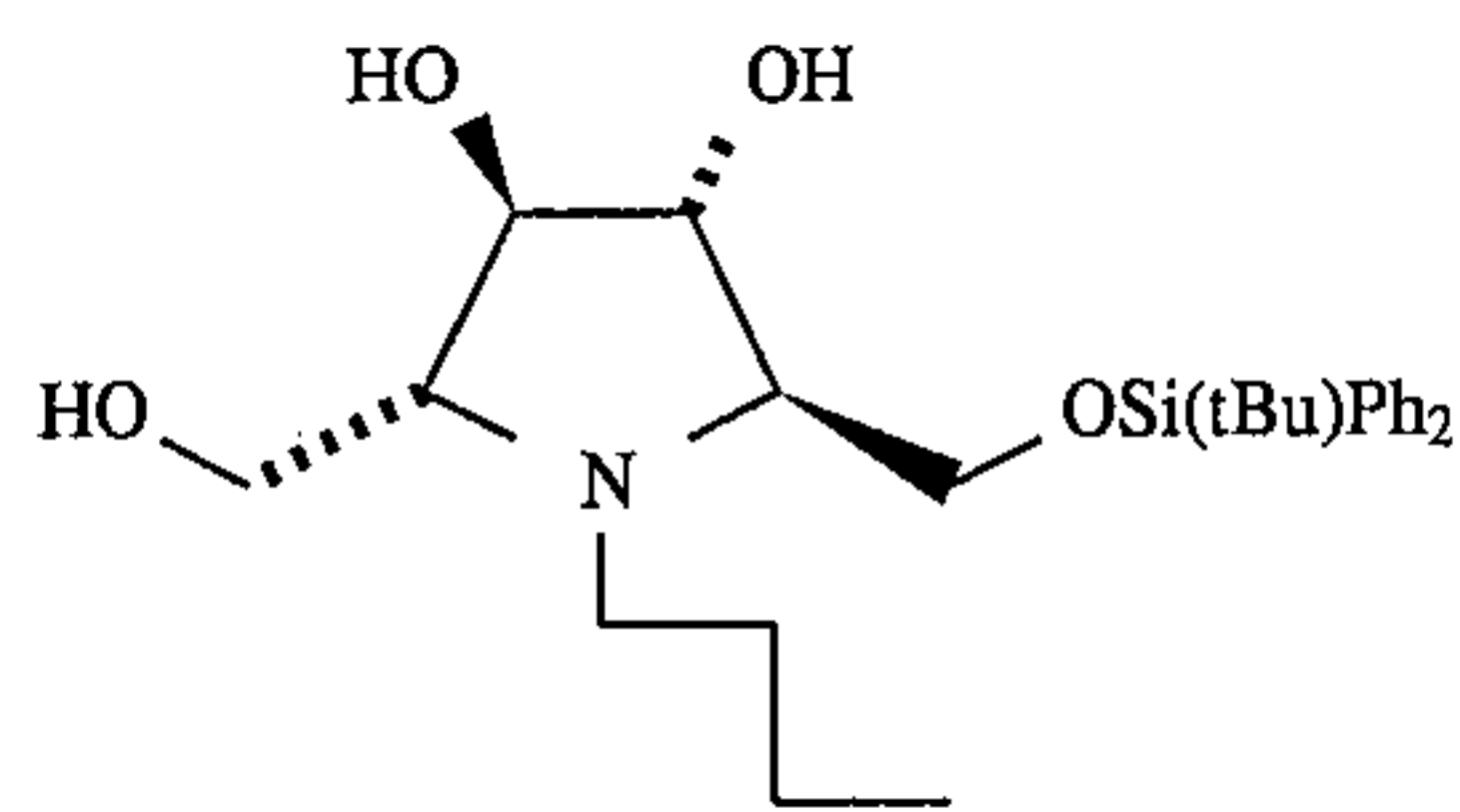
2,5-(Butylimino)-2,5-dideoxy-6-O-[(1,1-dimethylethyl)diphenylsilyl]-D-mannitol
