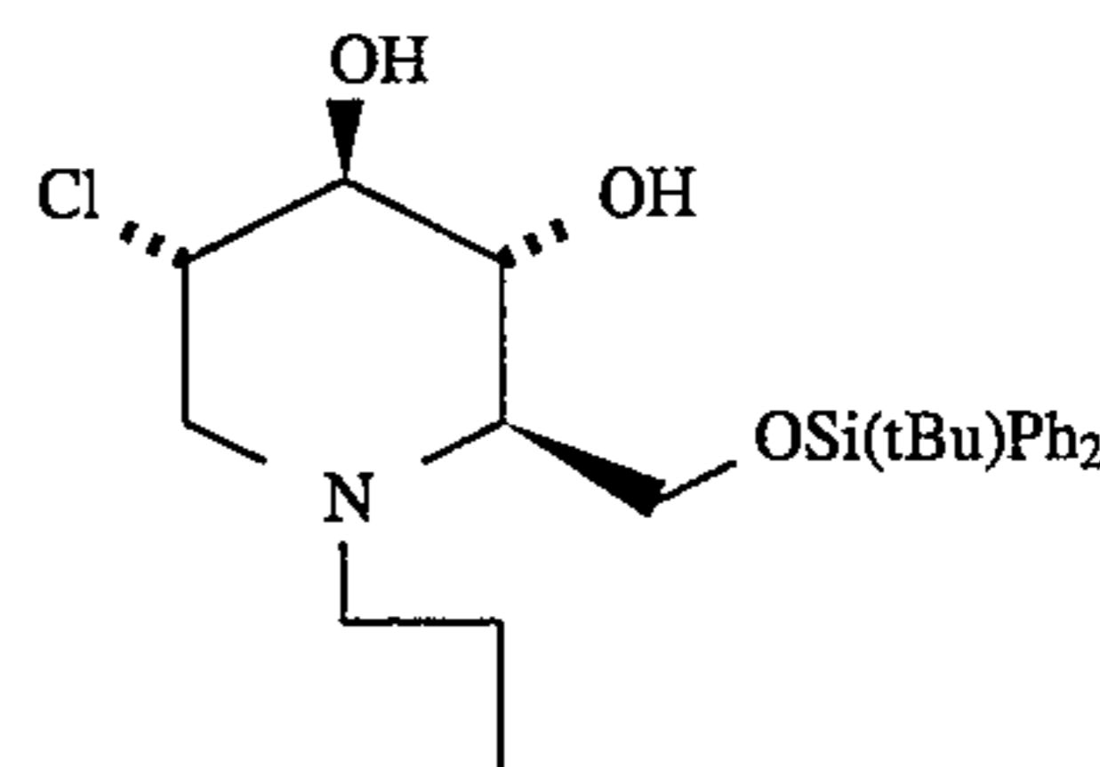
1,5-(Butylimino)-2-chloro-1,2,5-trideoxy-6-O-[(1,1-dimethylethylethyl)diphenylsilyl]-D-glucitol
