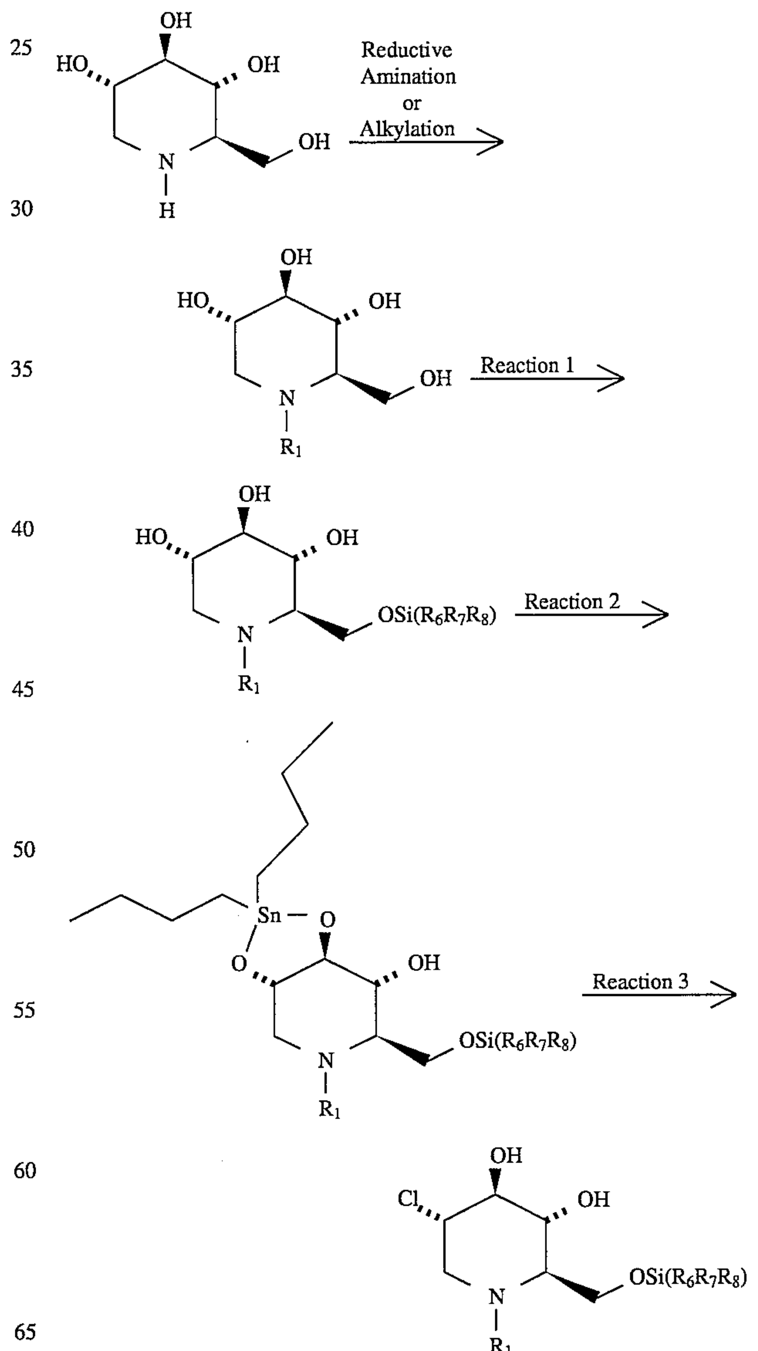
Scheme 1
