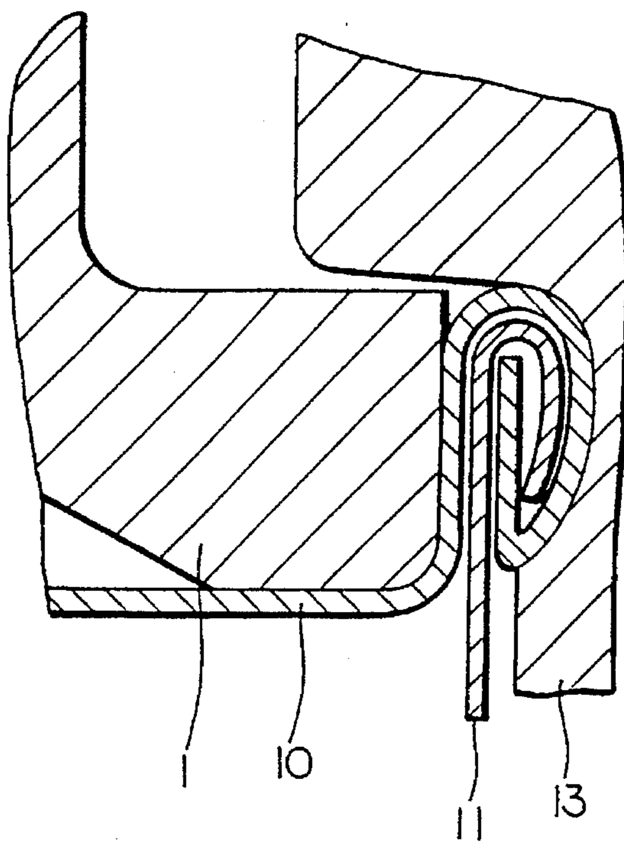
FIG. 24 PRIOR ART
