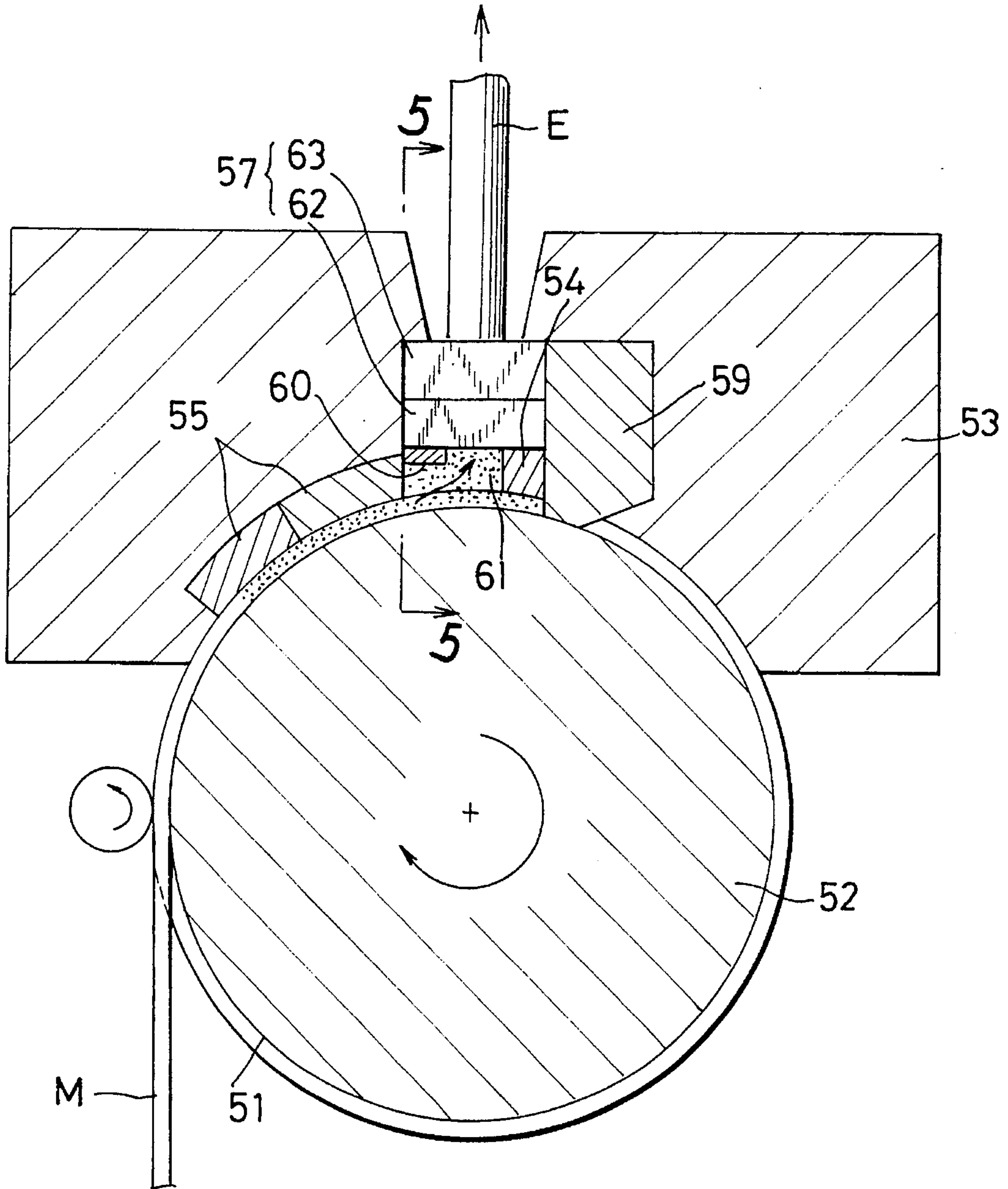
FIG. 10 (PRIOR ART)
