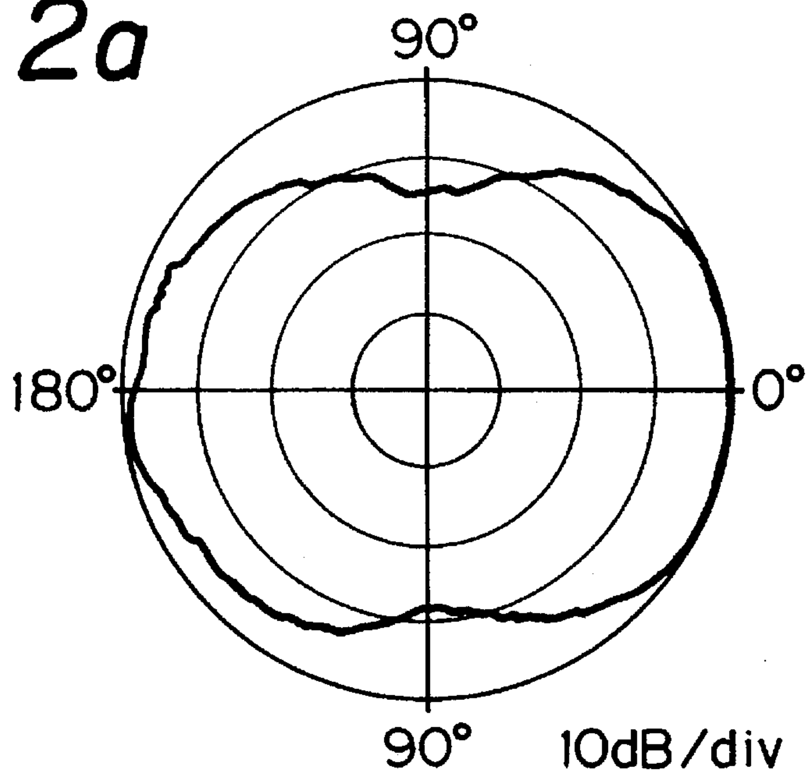
MAGNETIC FIELD PLANE (H-PLANE)
