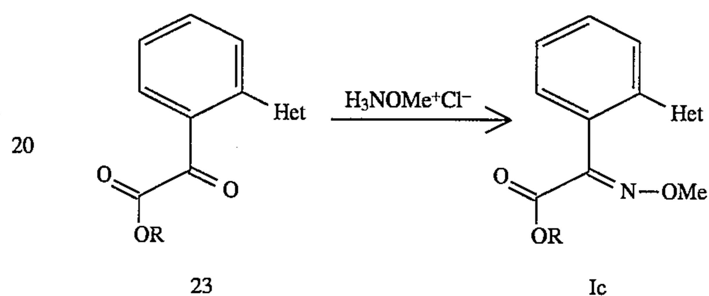
Scheme 9
