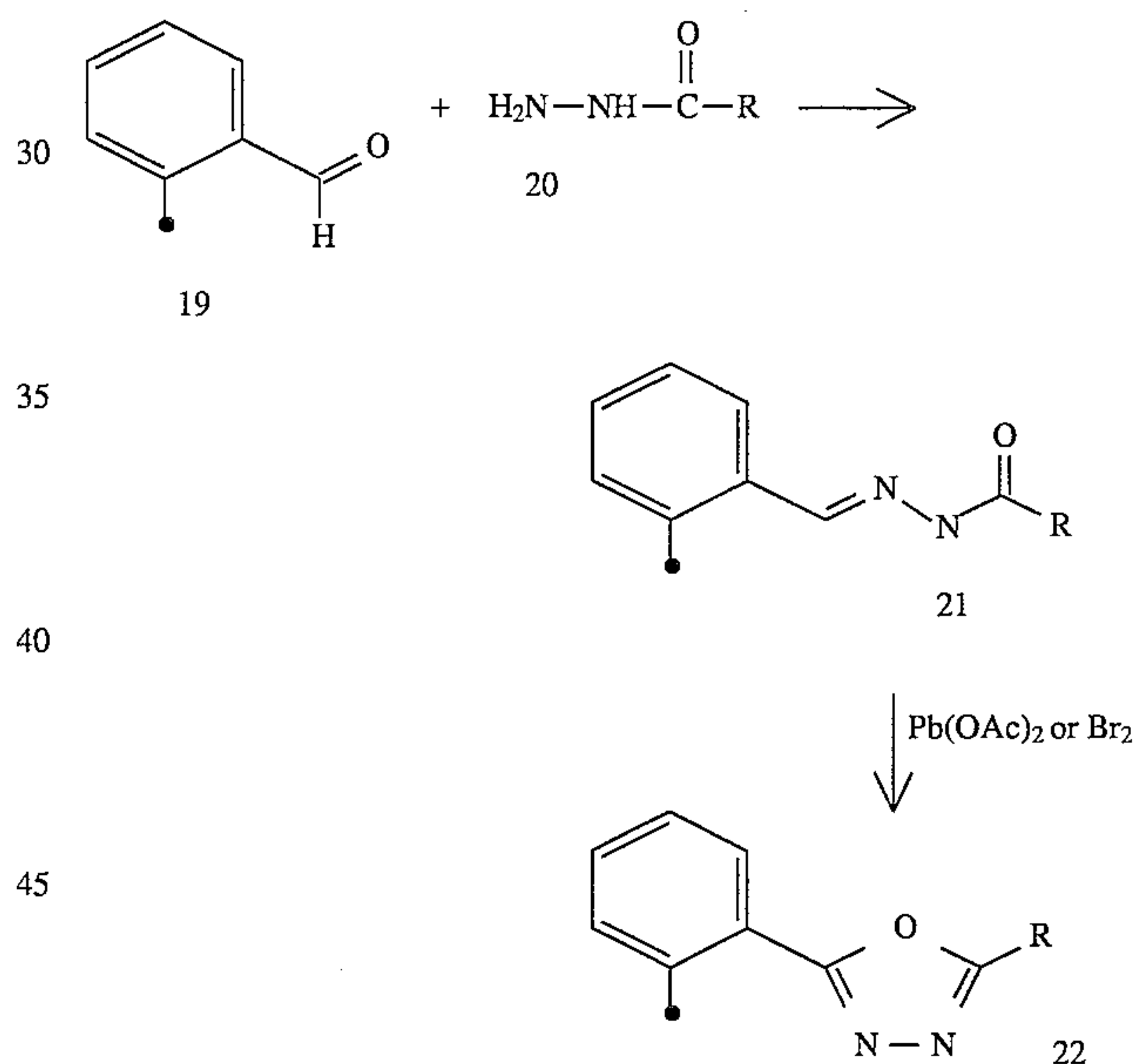
Scheme 7
