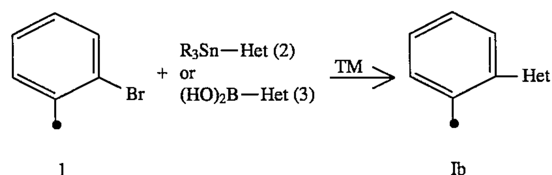
Scheme 1
