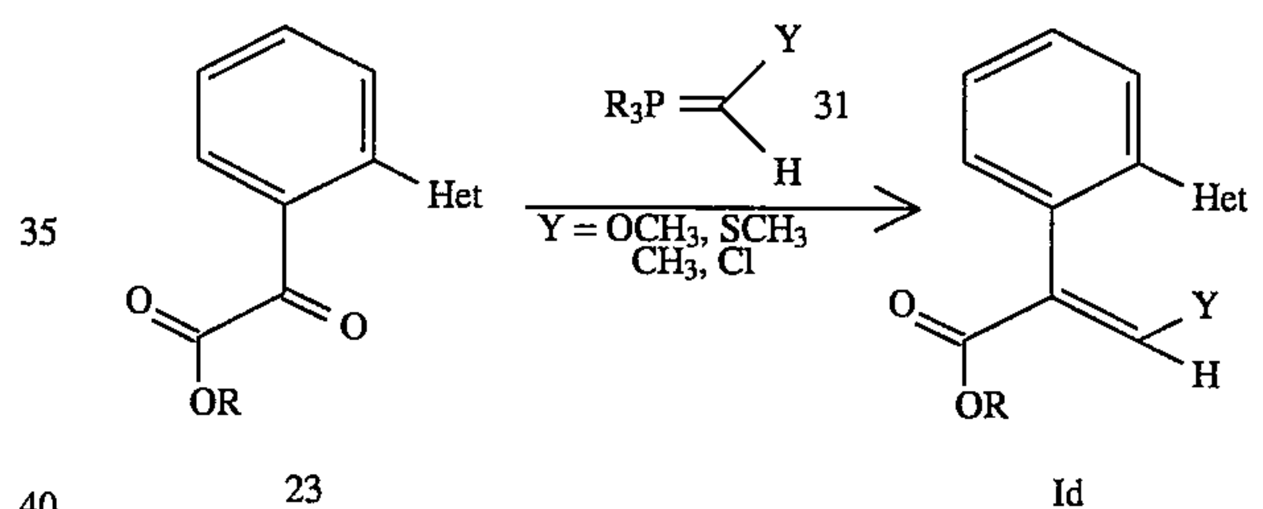
Scheme 10
