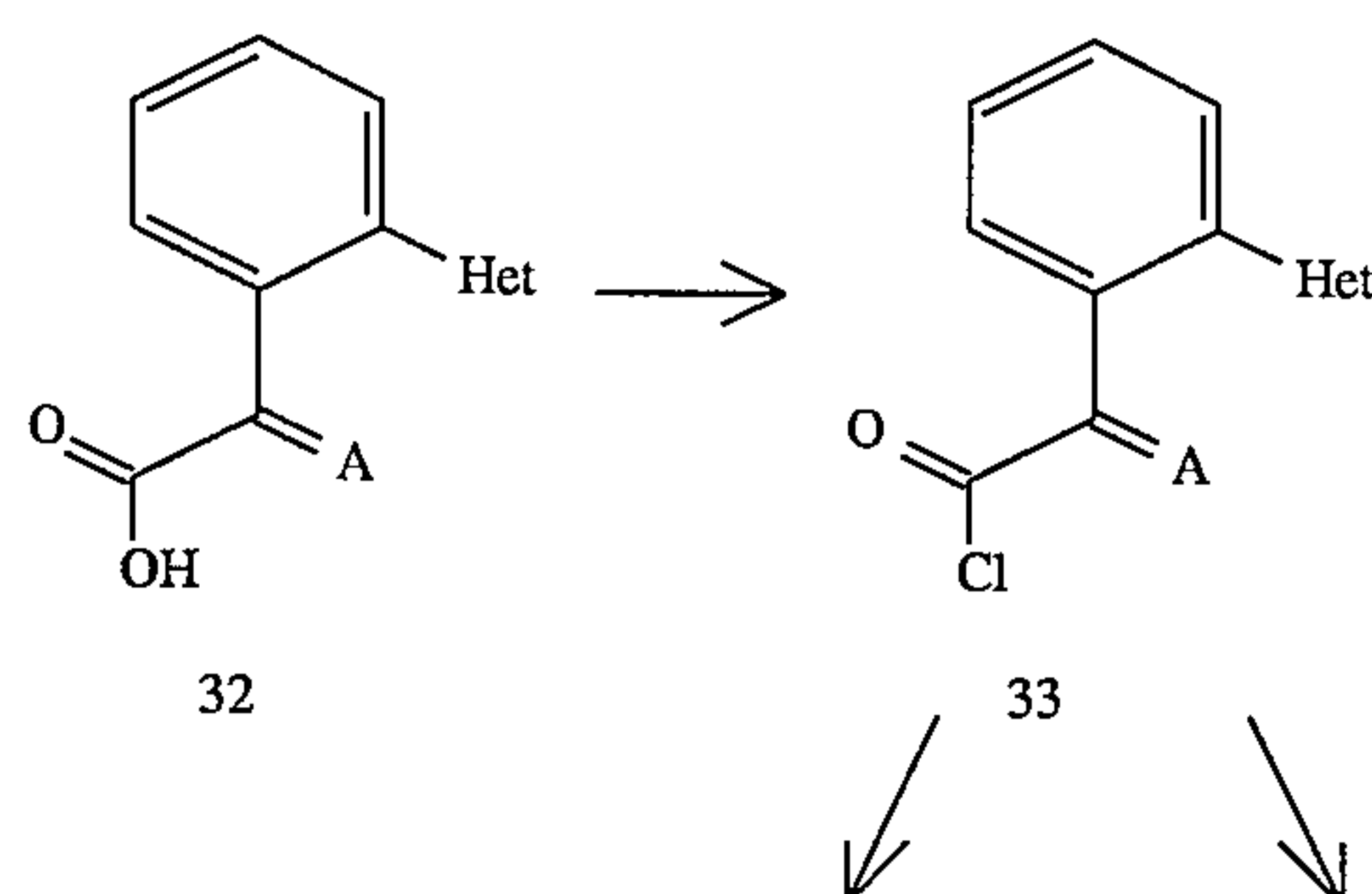
Scheme 11
