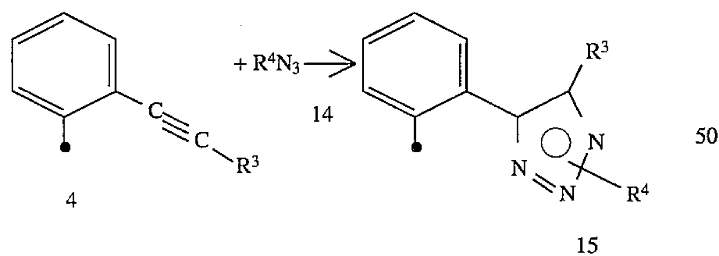
Scheme 5
