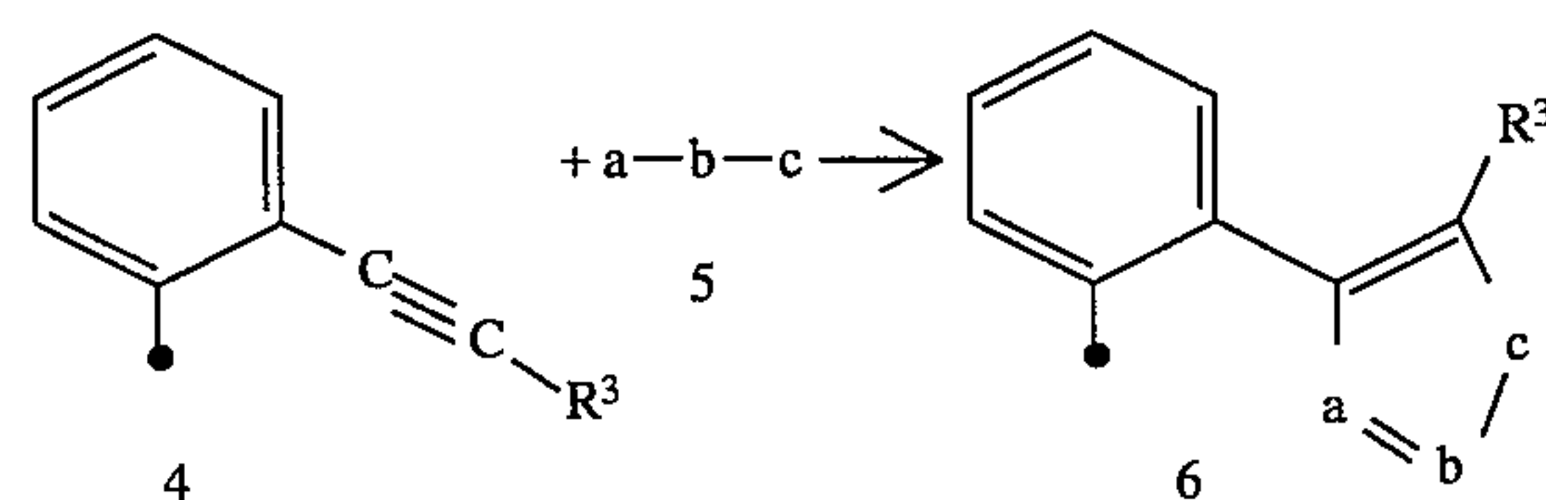
Scheme 2
