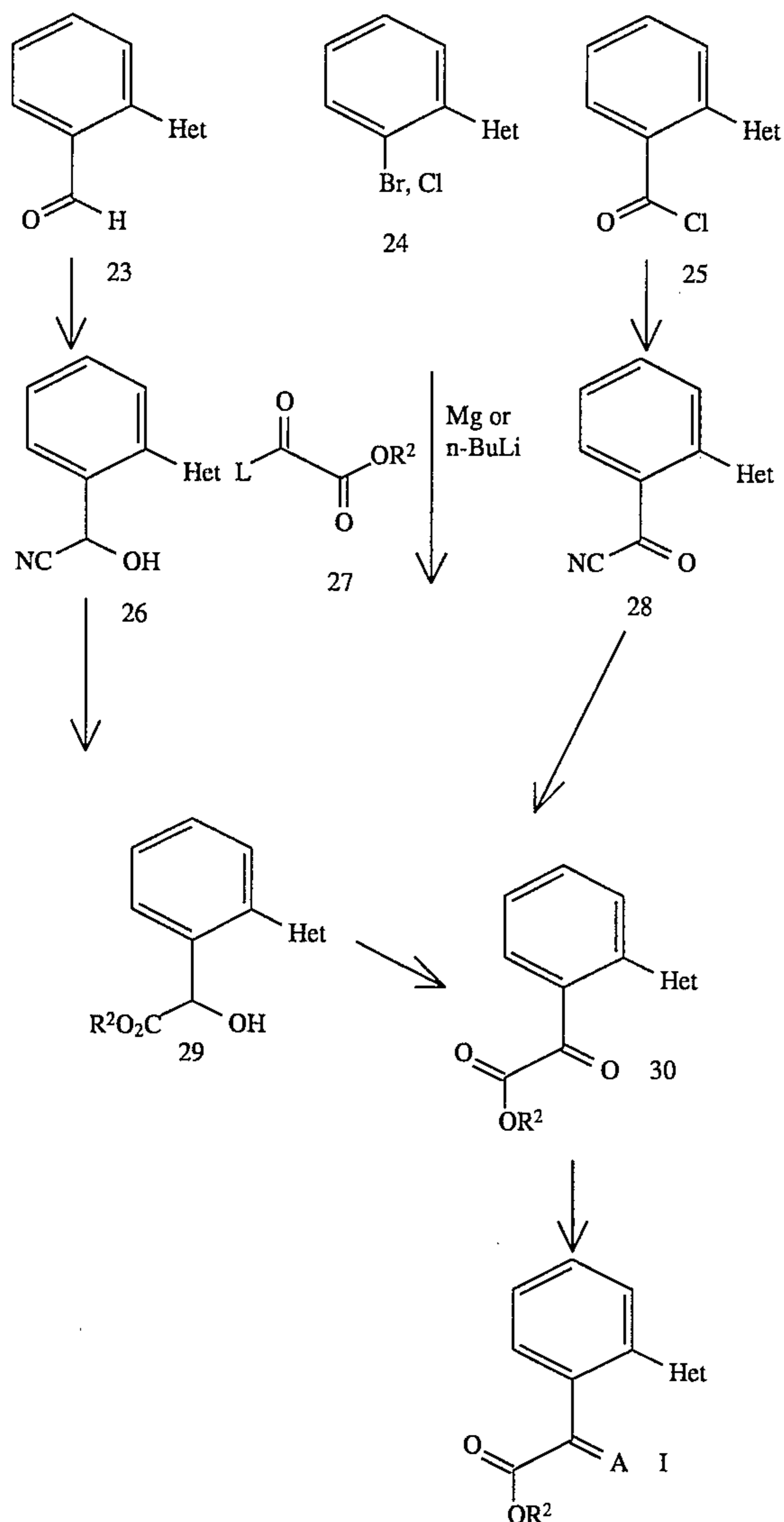
Scheme 8
