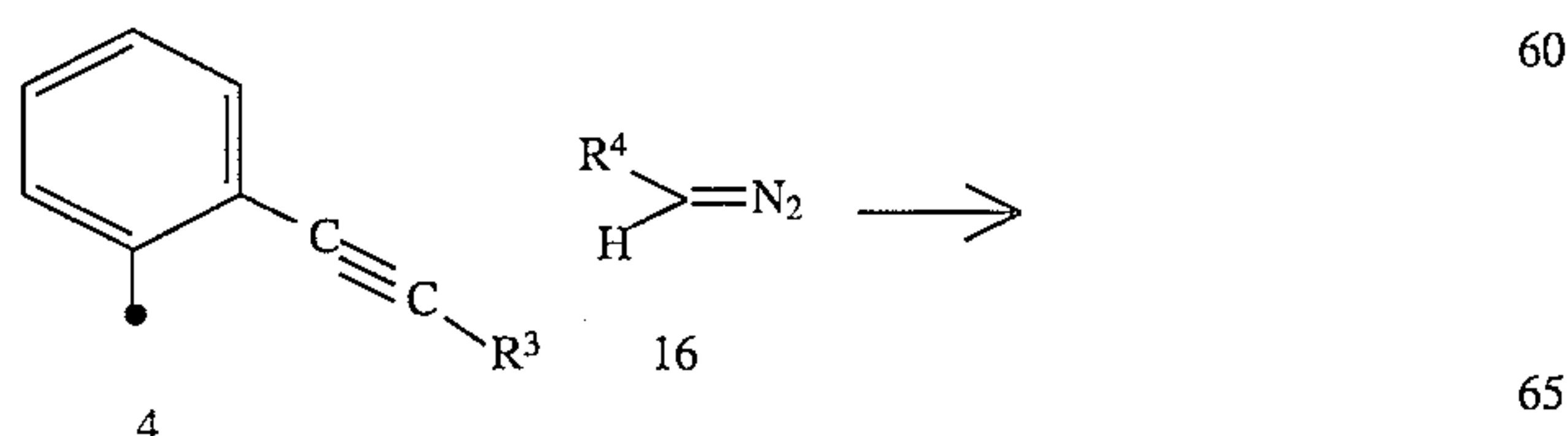
Scheme 6
