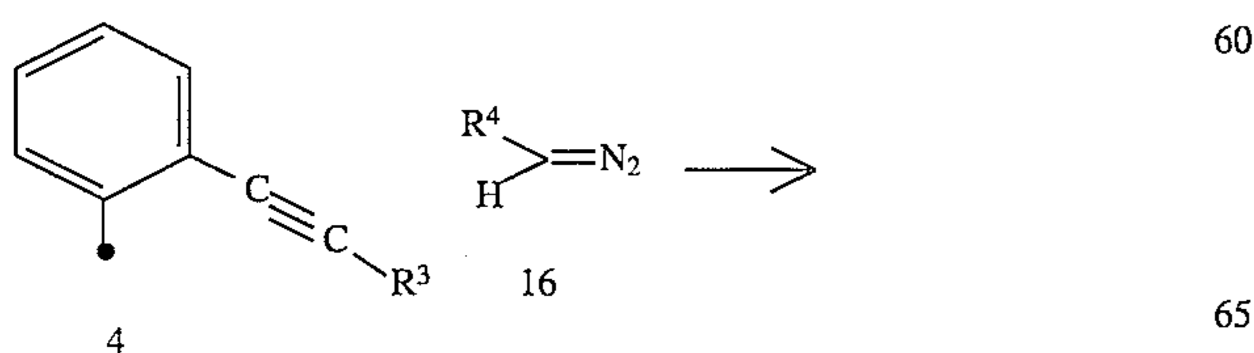
Scheme 6
