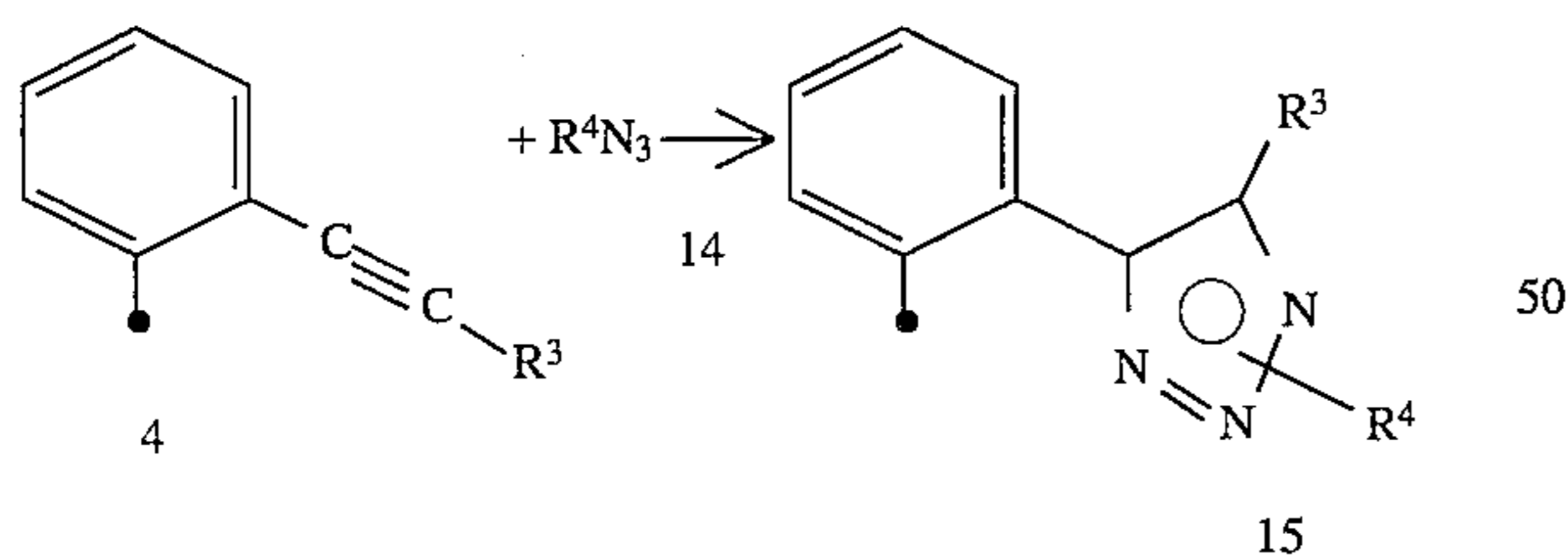
Scheme 5
