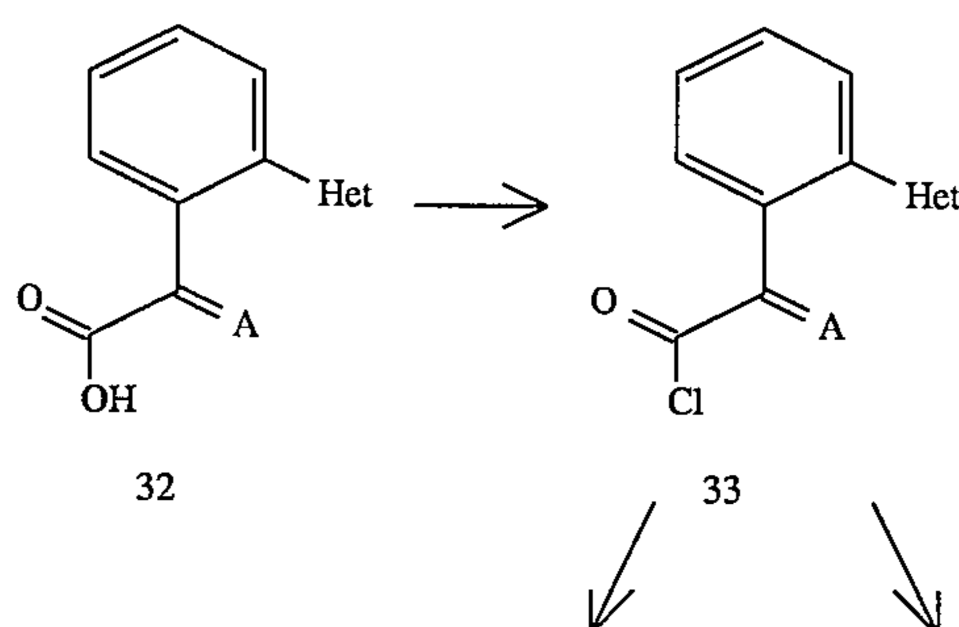
Scheme 11
