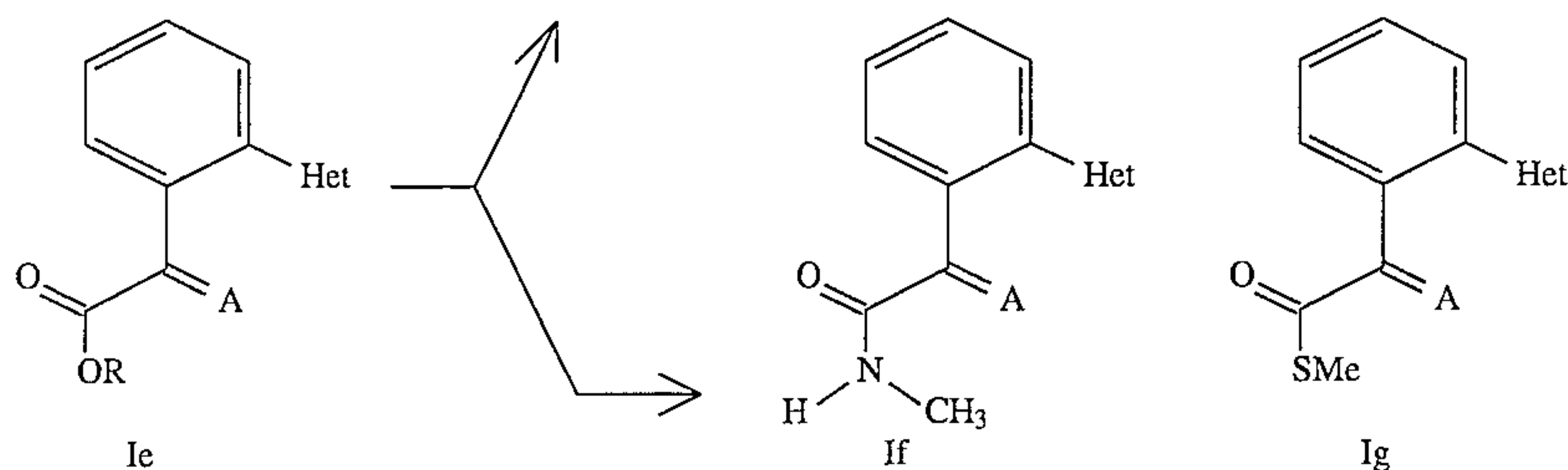
-continued Scheme 11
