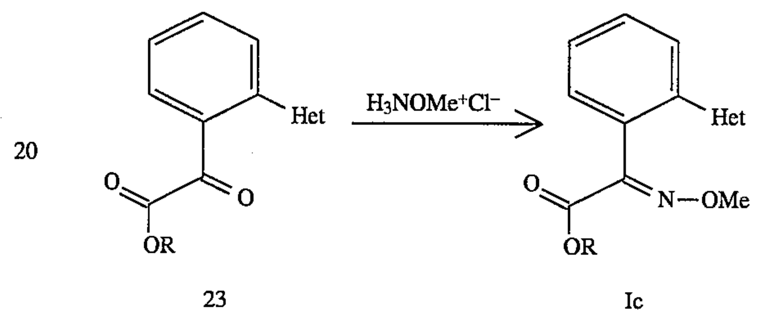
Scheme 9
