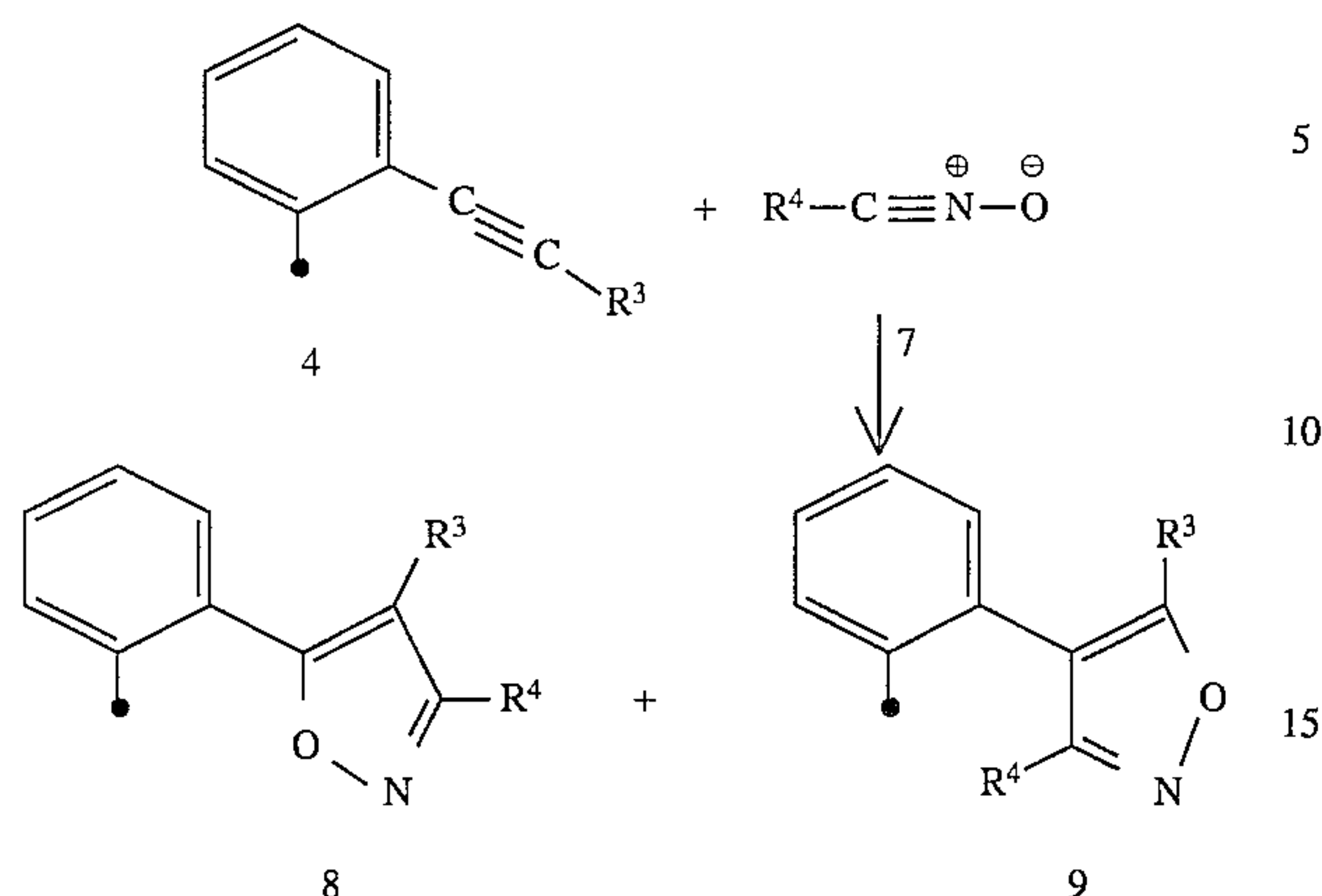
Scheme 3
