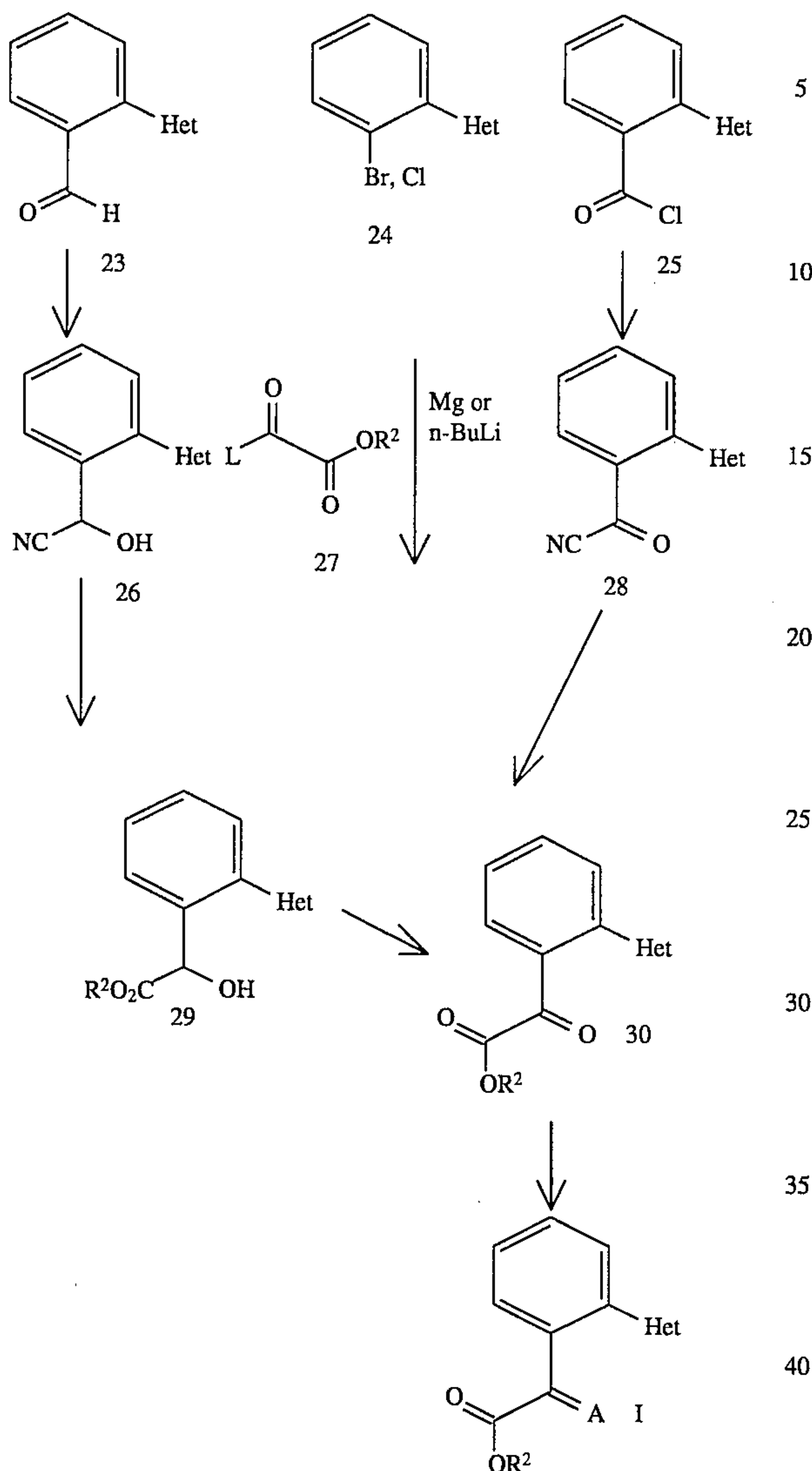
Scheme 8
