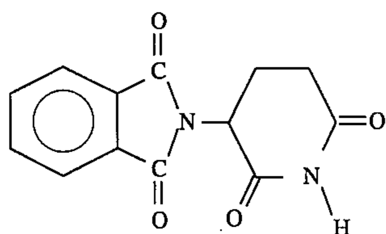
thalidomide
