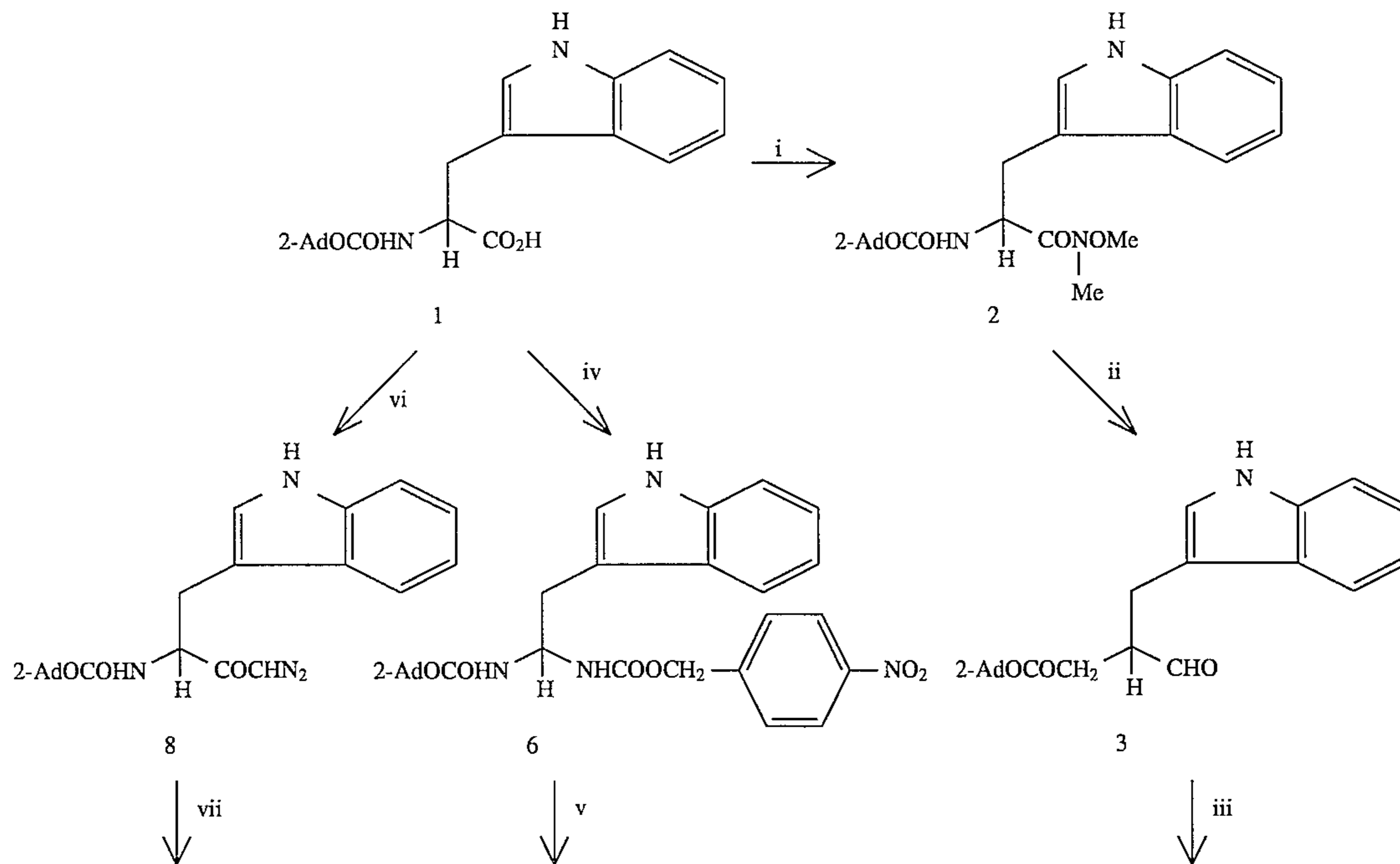
Scheme 1
