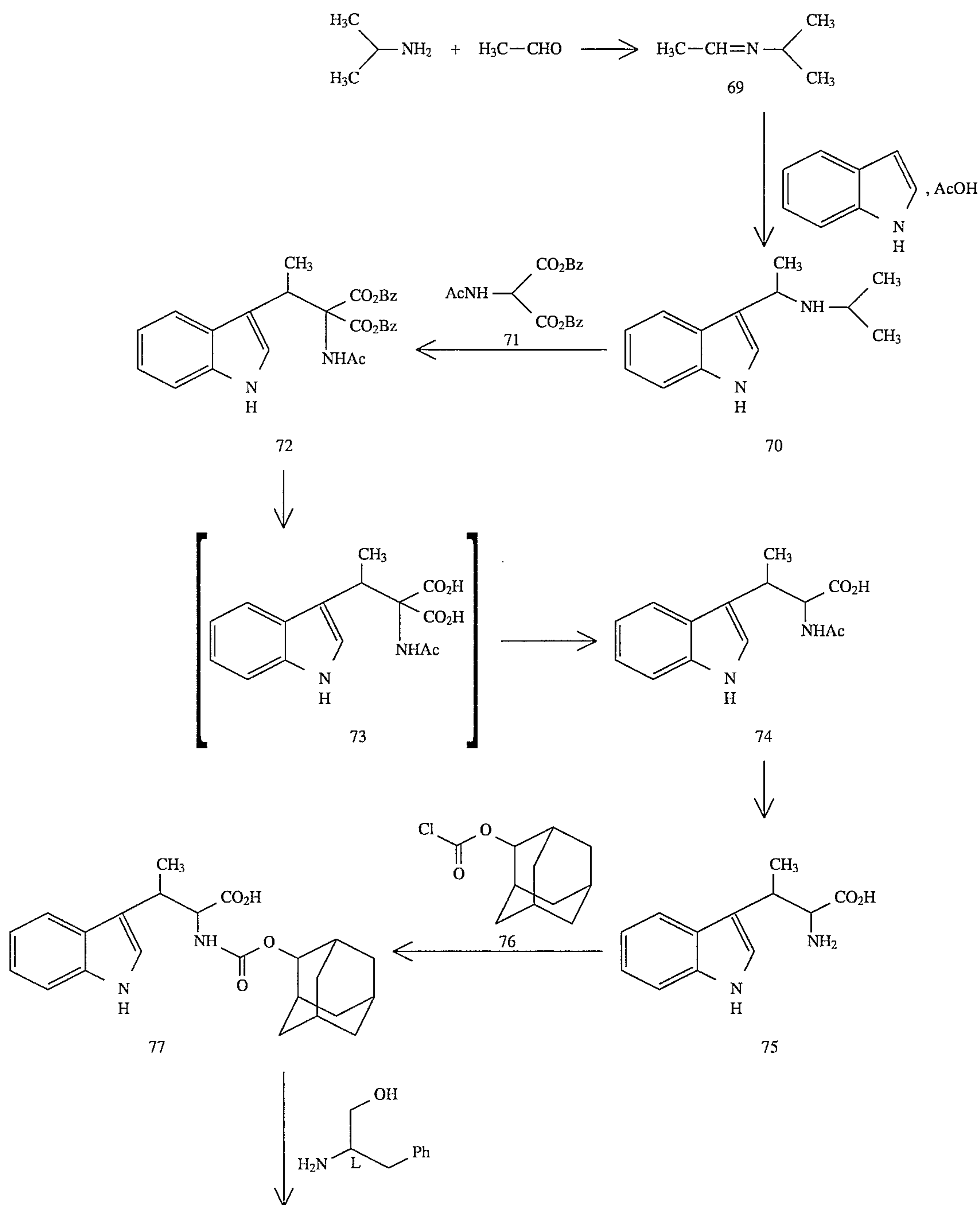
SCHEME 10
