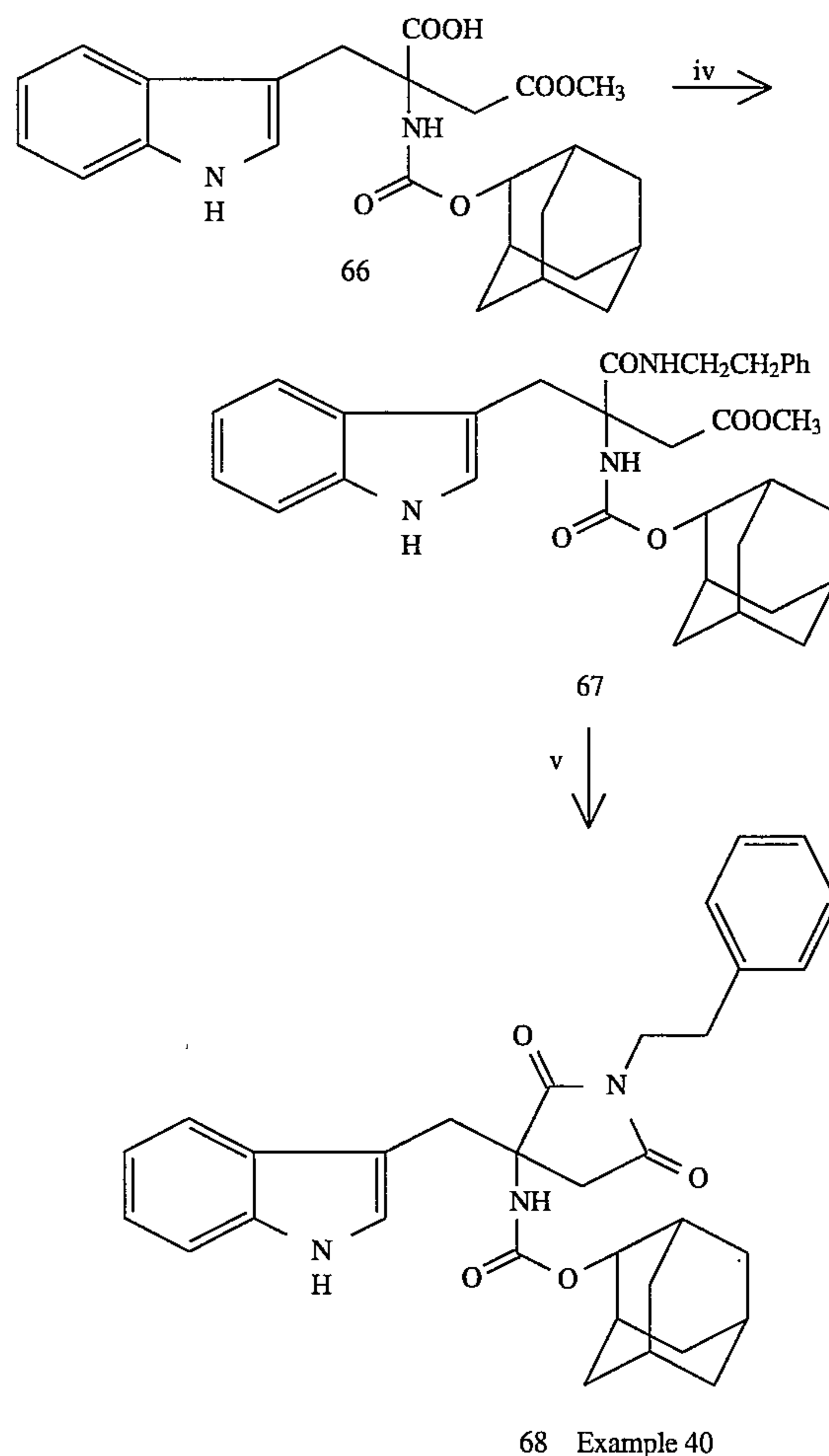
-continued SCHEME 9
