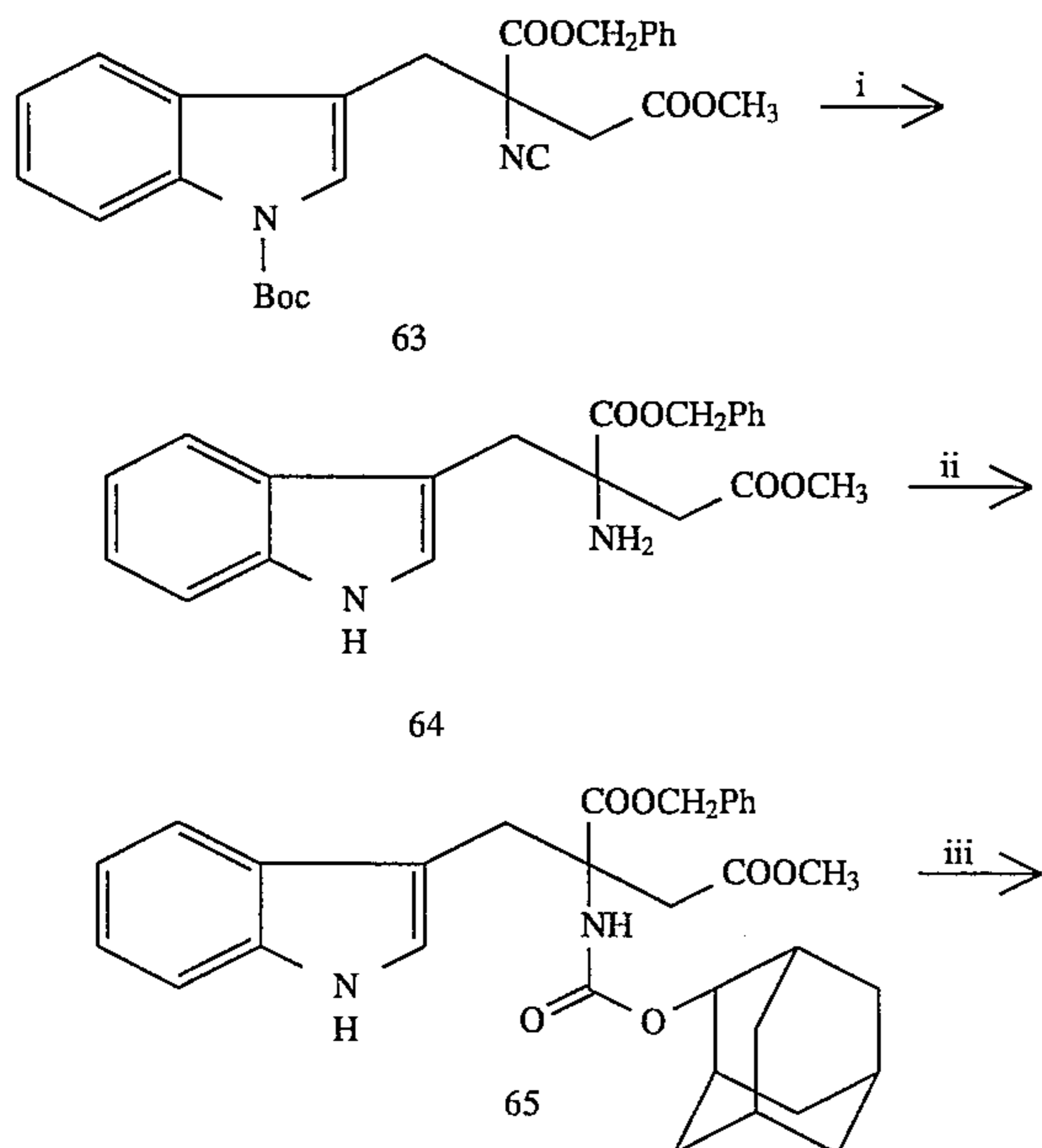
SCHEME 9
