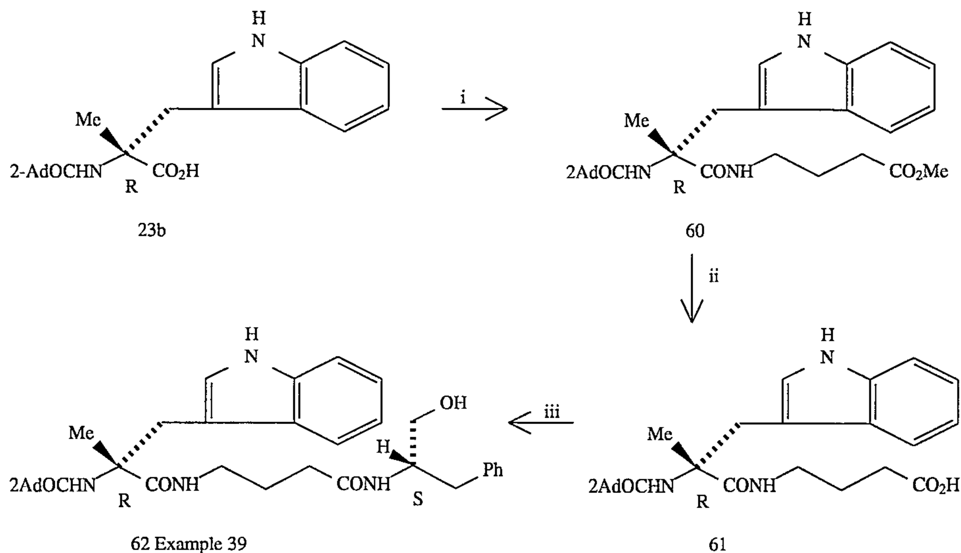
SCHEME 8
