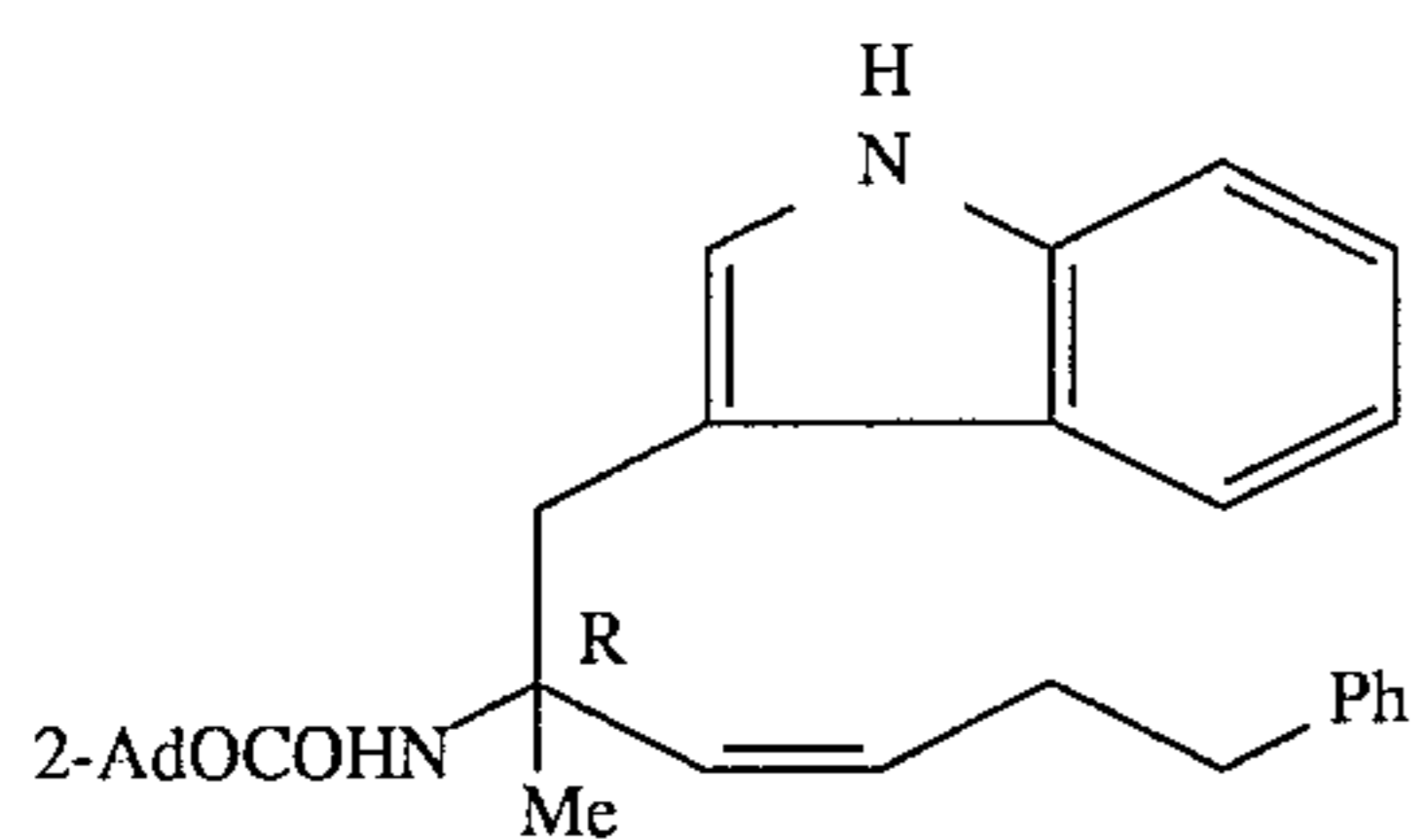
27 Example 14
