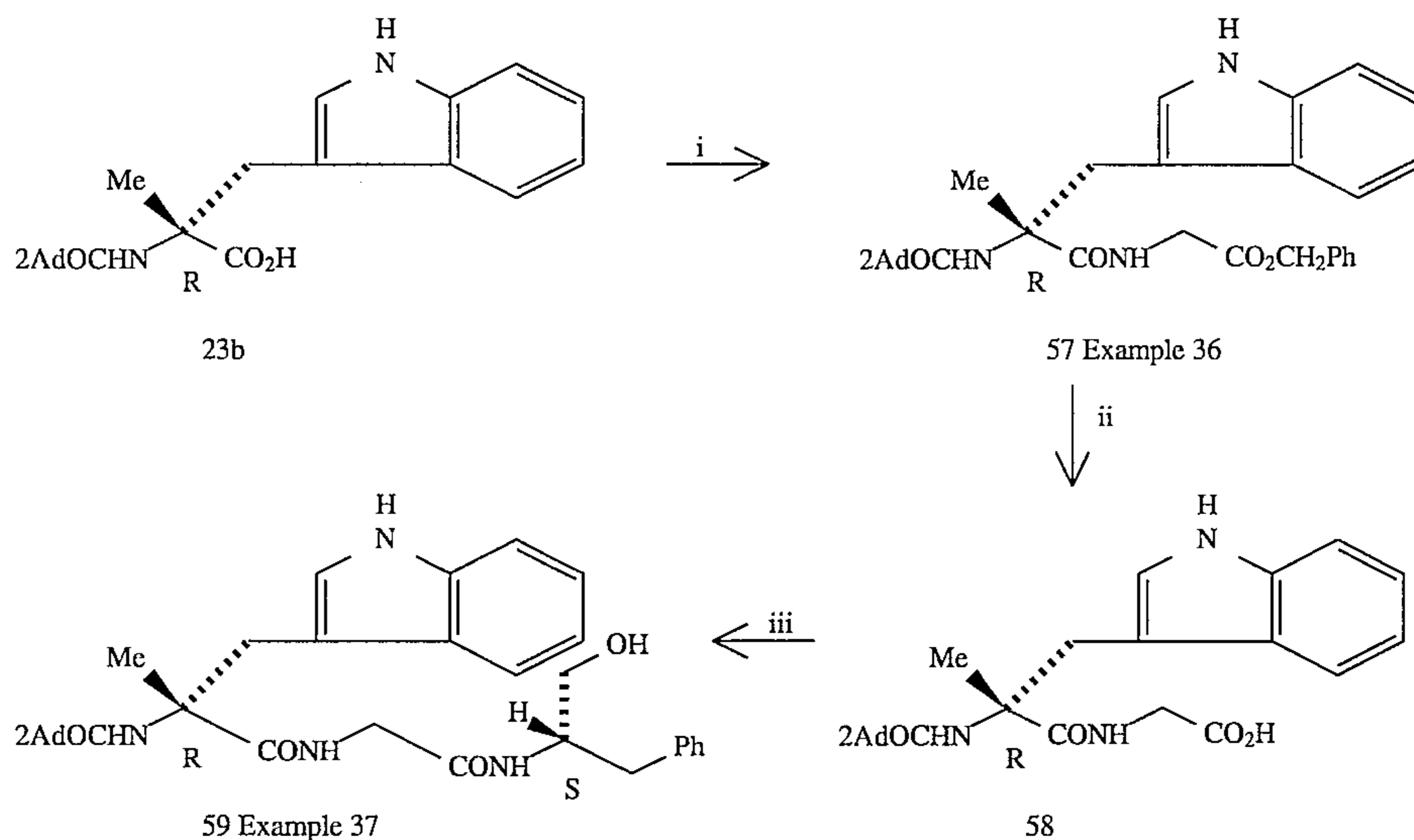
SCHEME 7
