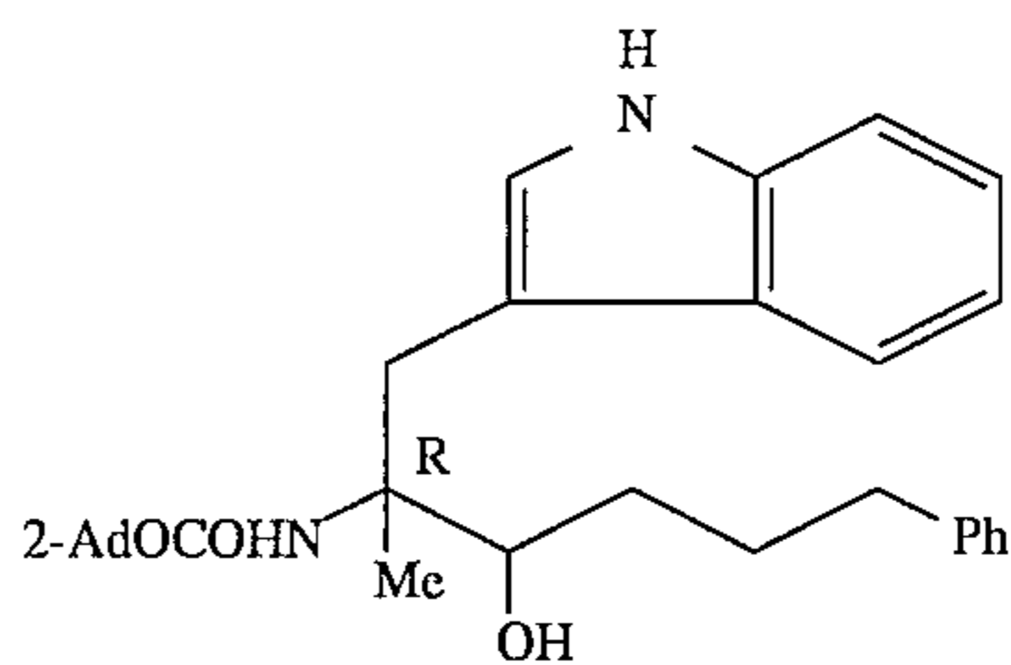
28 Example 15
