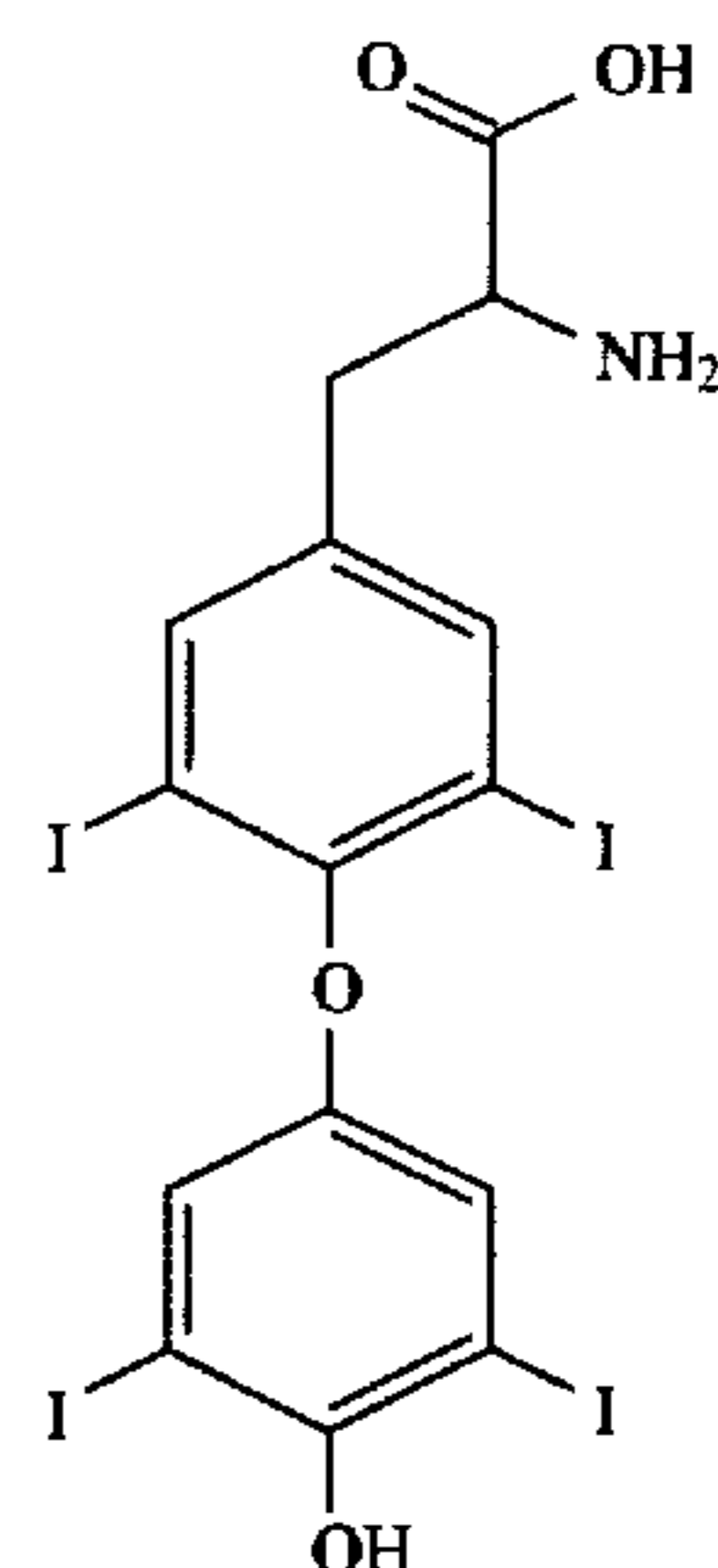
FORMULA 1 L- AND D- THYROXINE
