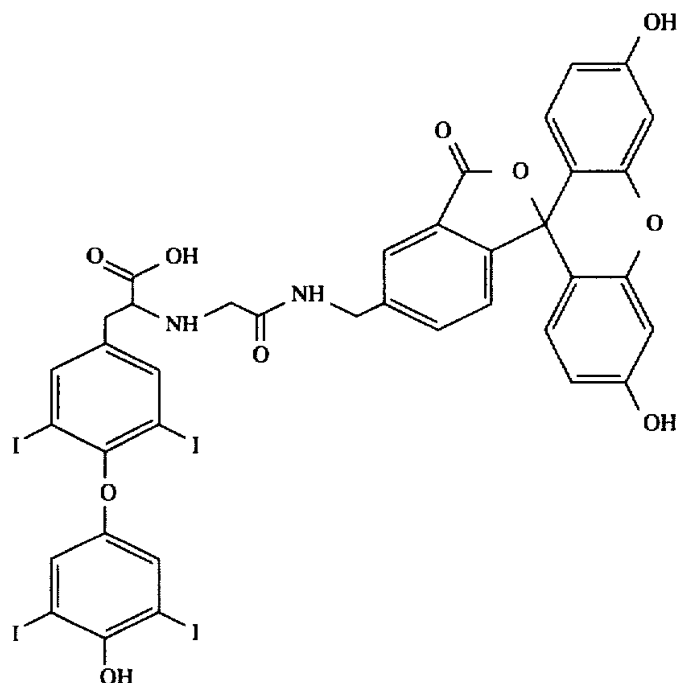
FORMULA 5 STRUCTURE OF THE PREFERRED THYROXINE TRACER
