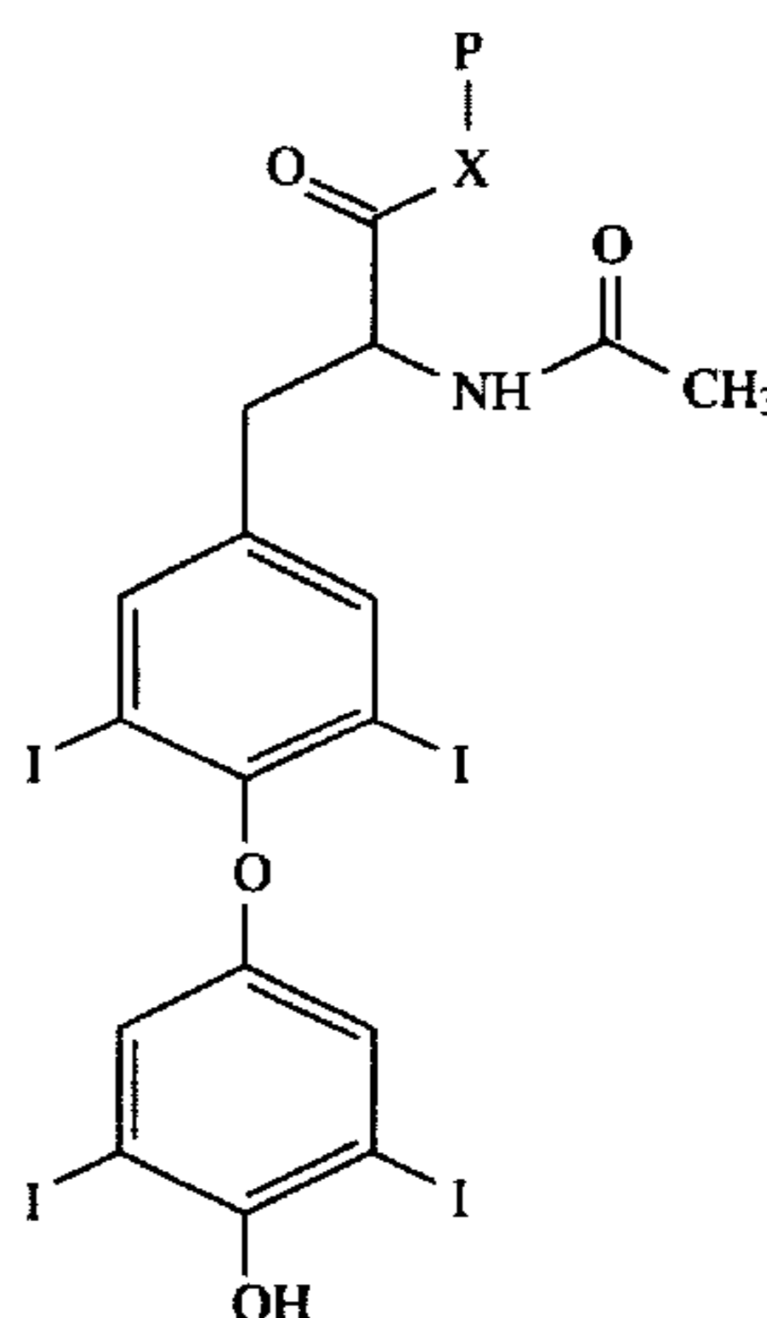
FORMULA 2. GENERAL STRUCTURE OF THE IMMUNOGEN
