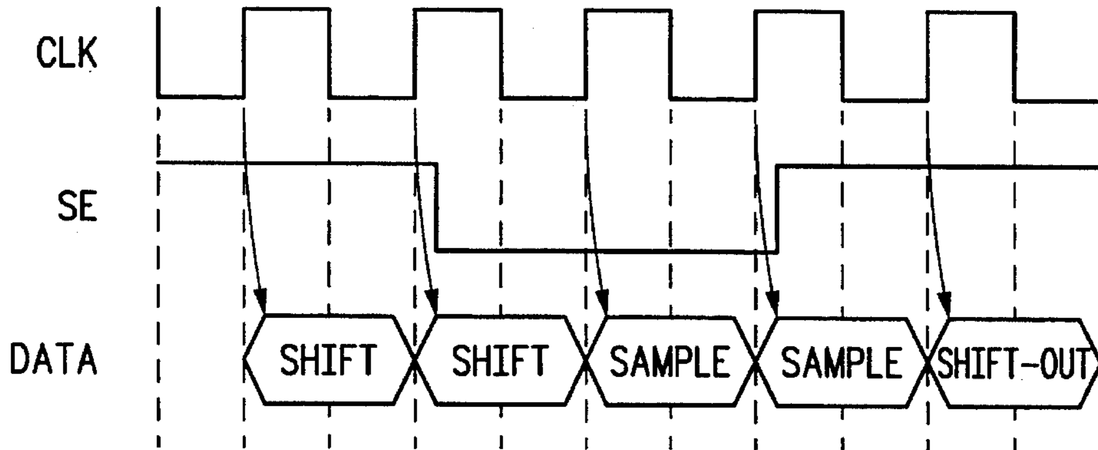
DELAY FAULT TIMING SCAN
