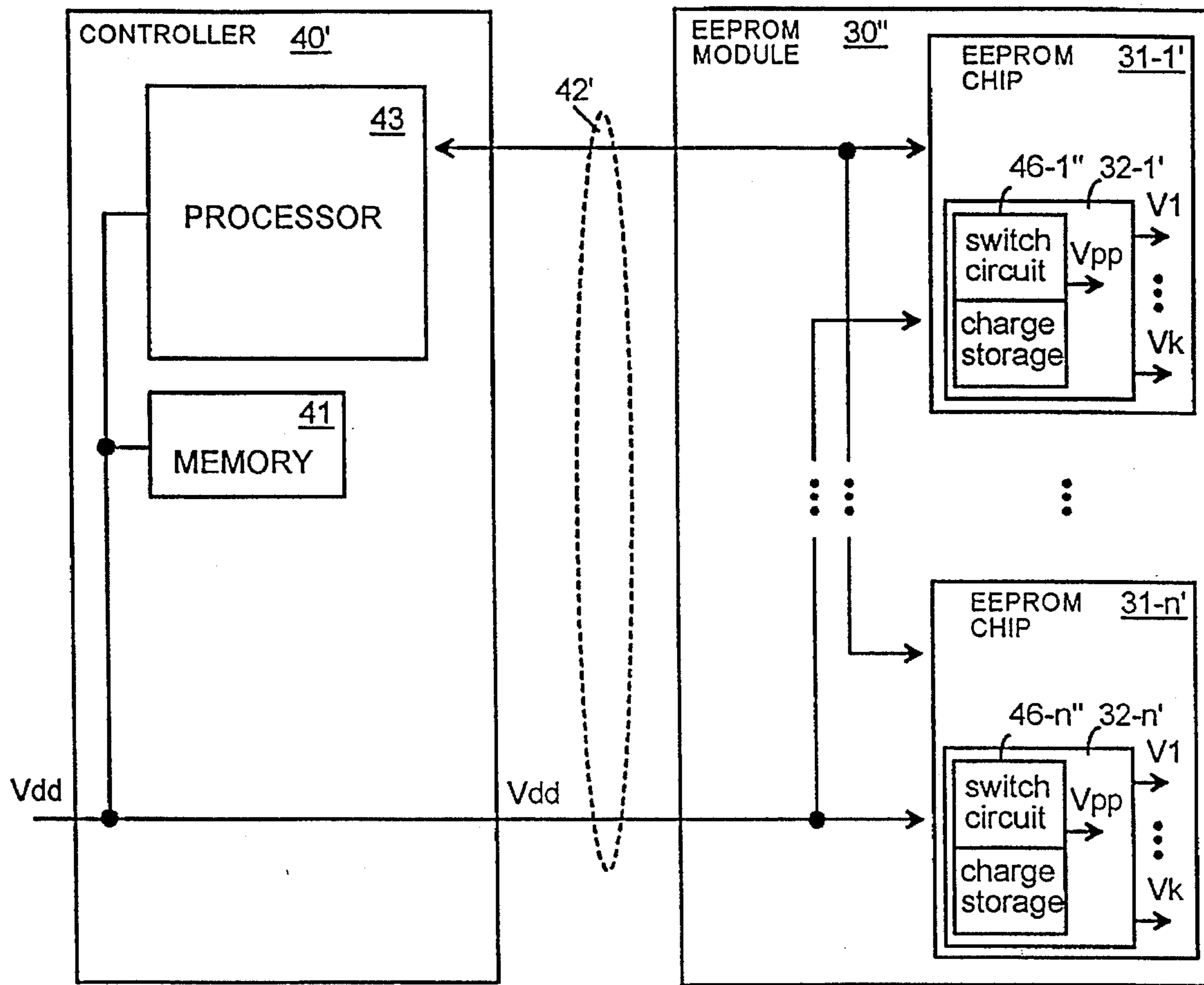
FIG.2C PRIOR ART
