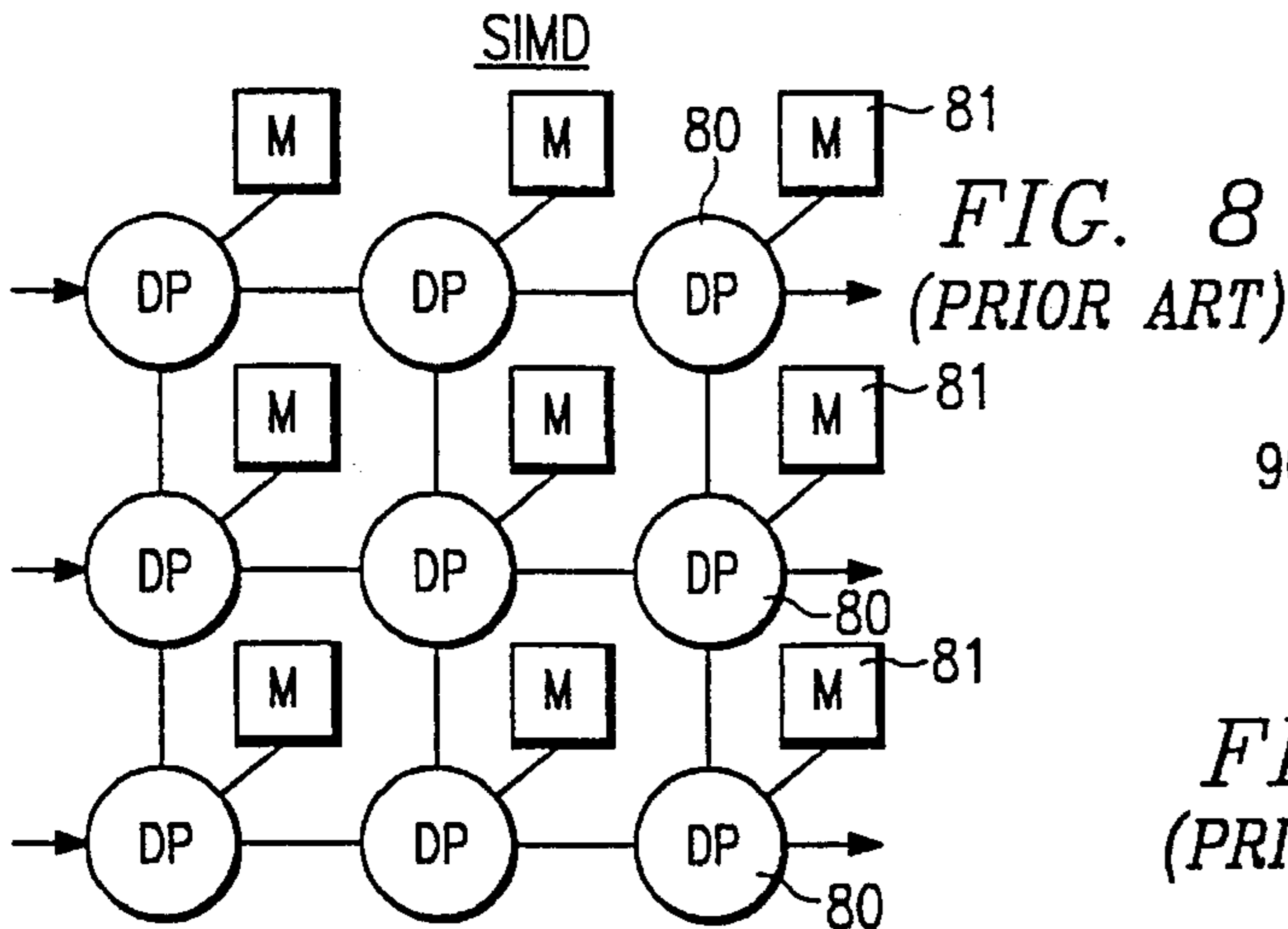
FIG. 7 (PRIOR ART)
