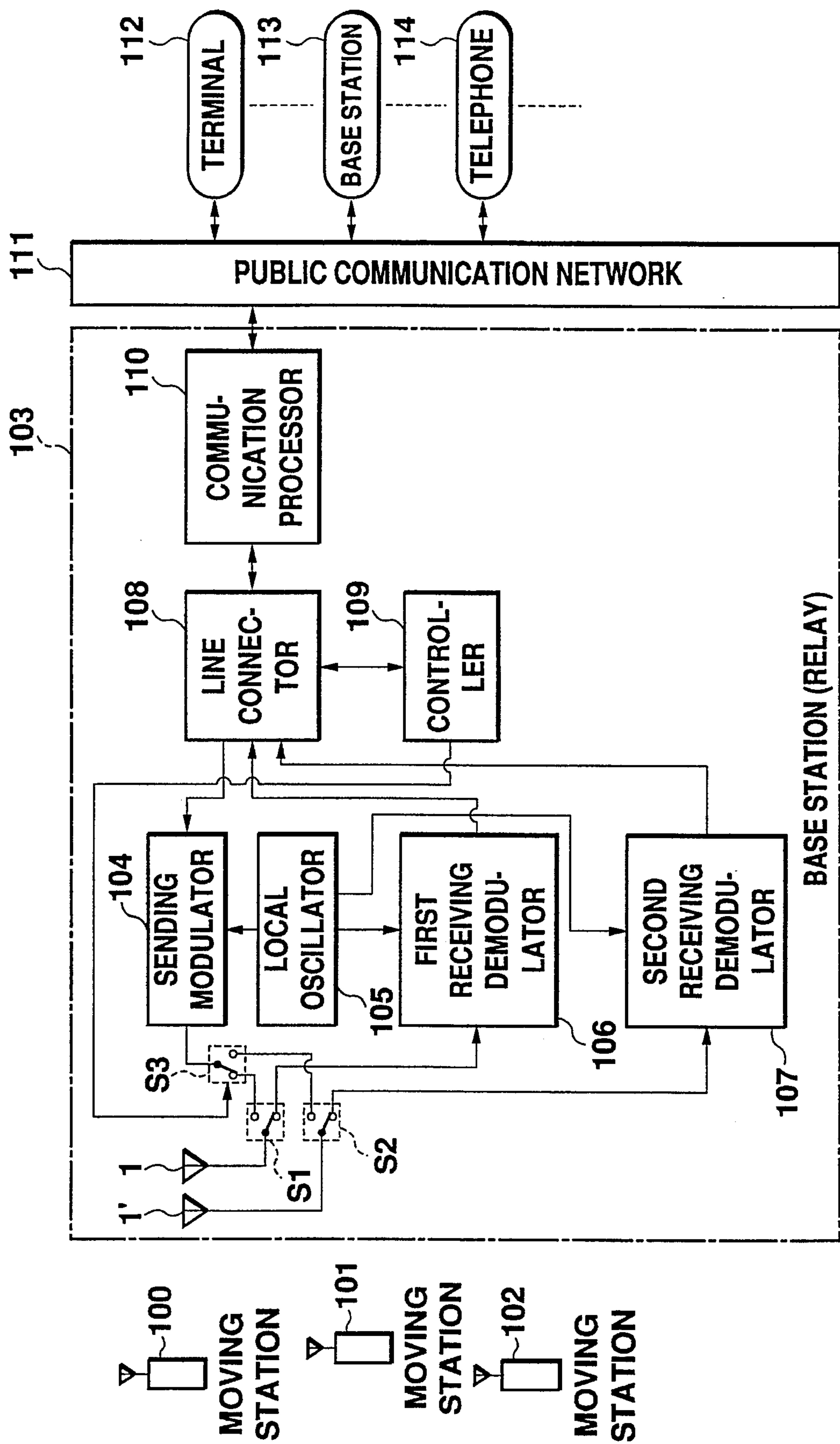
Fig. 30 PRIOR ART
