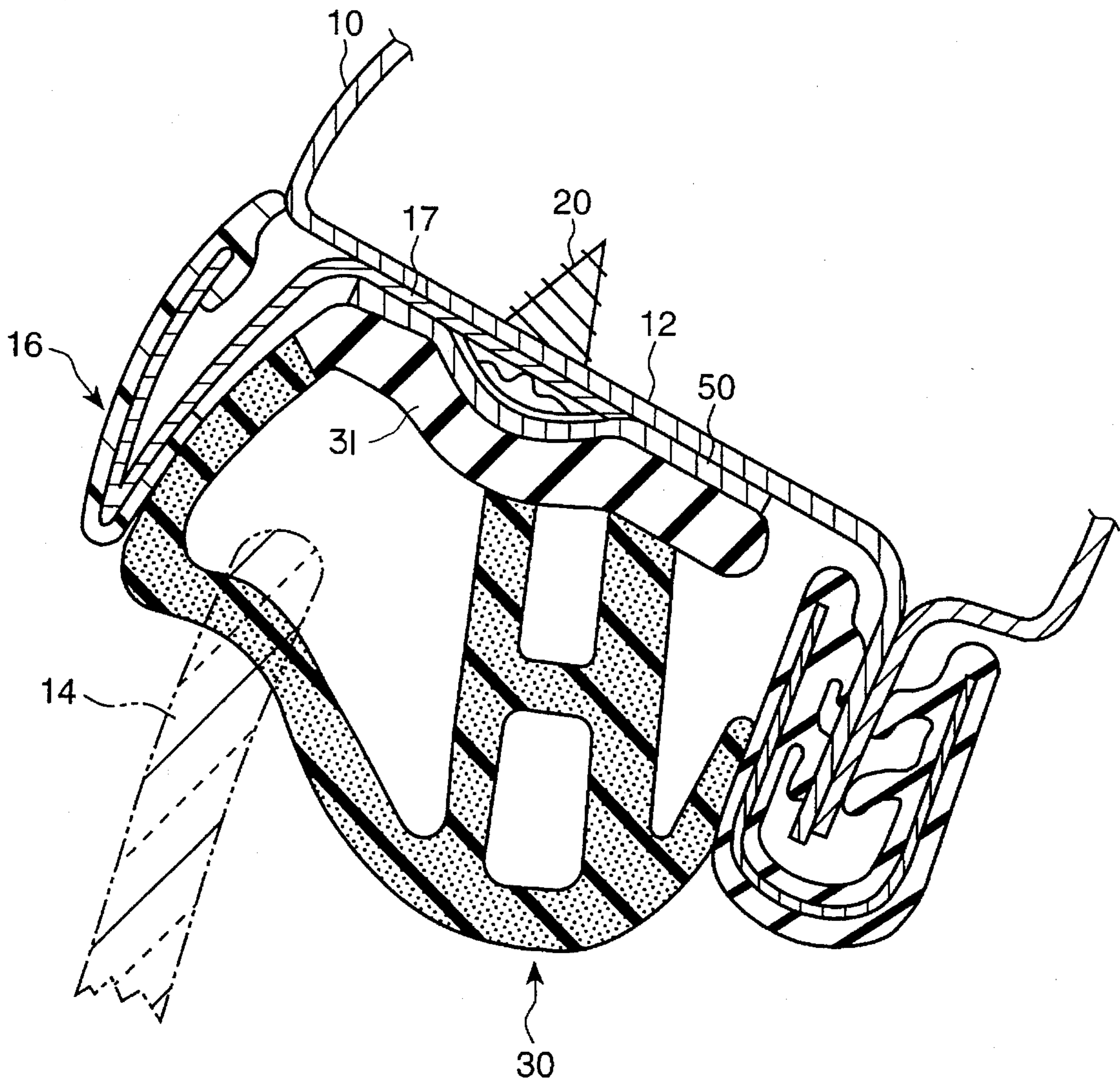
Fig. 1 (PRIOR ART)
