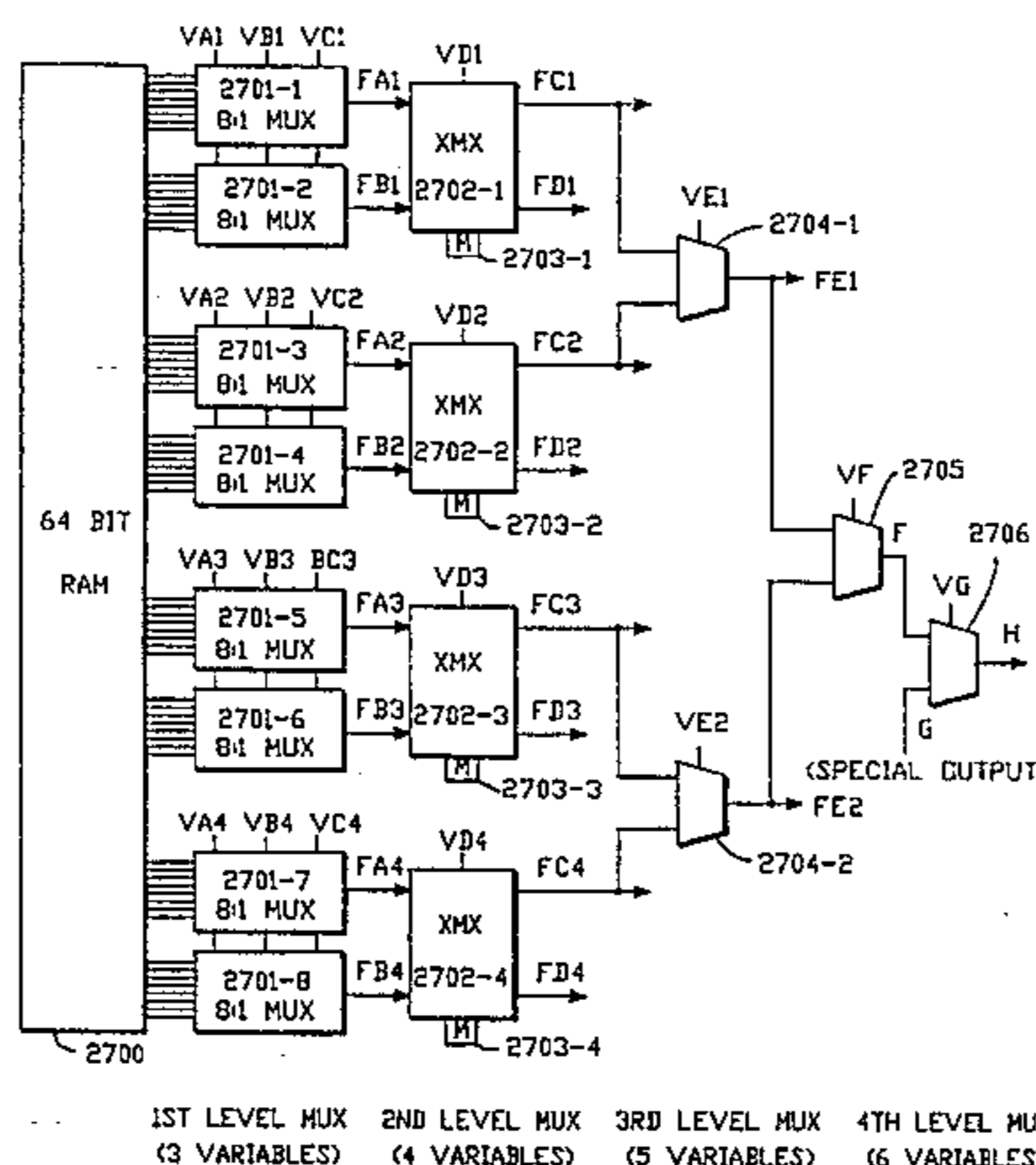
CLB CONFIGURATION
