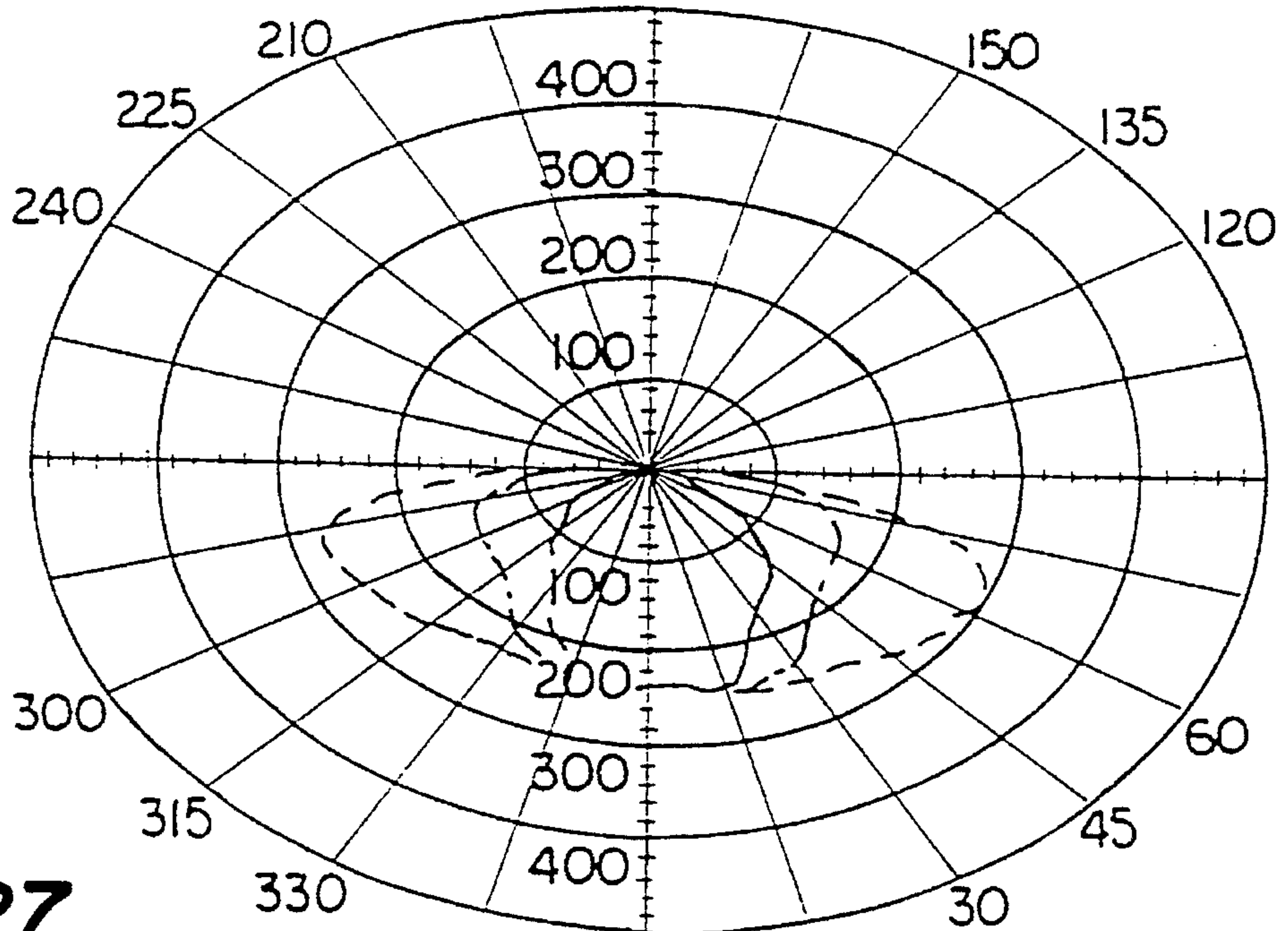
CANDLEPOWER DISTRIBUTION WITH HALF COATED TUBE
