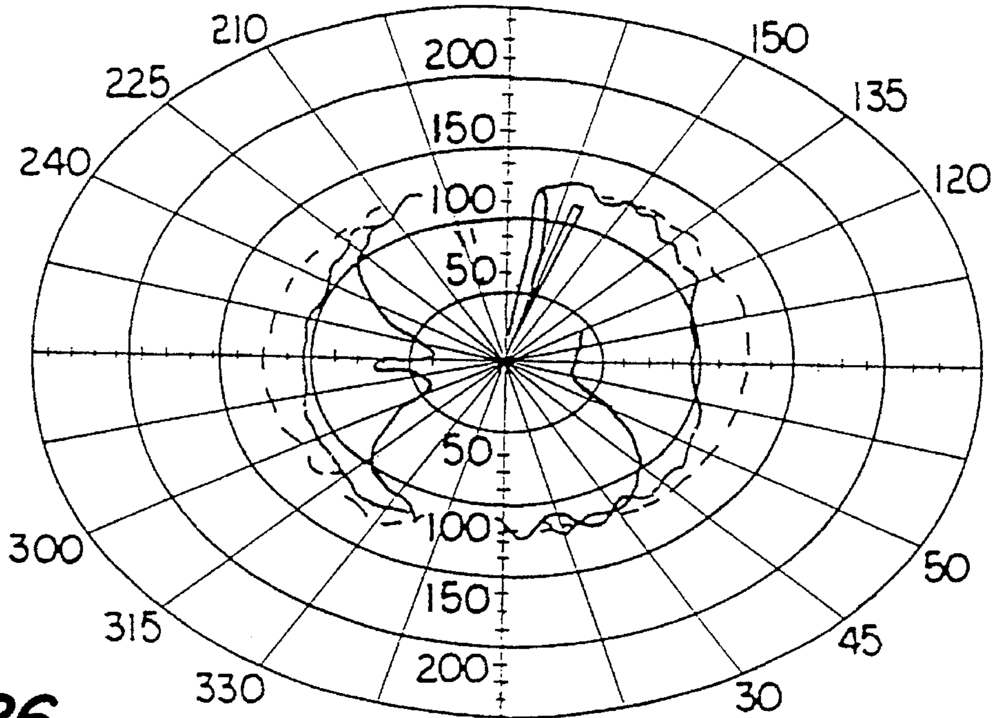
CANDLEPOWER DISTRIBUTION WITH UNCOATED TUBE
