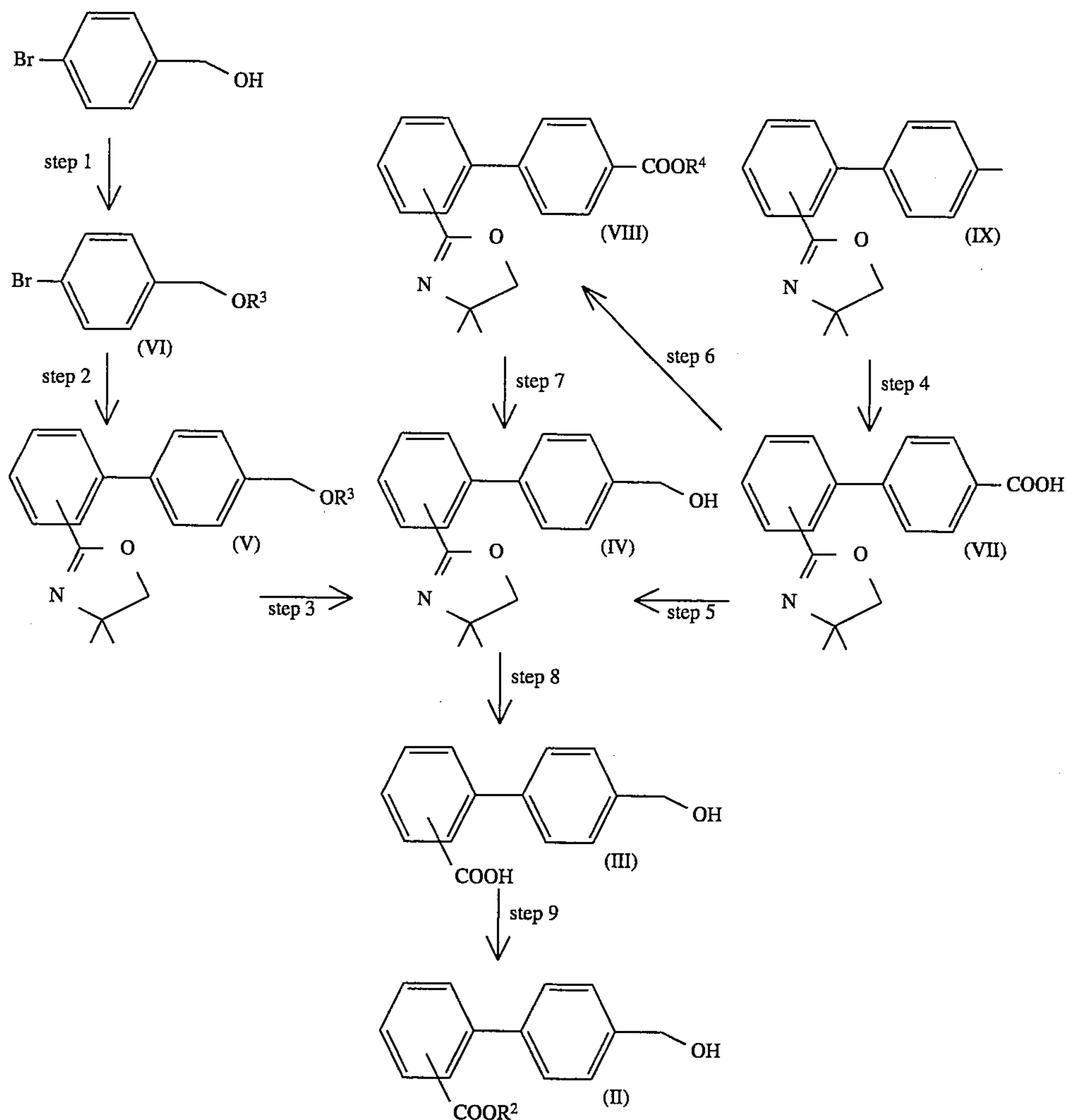
Reaction Scheme-7
