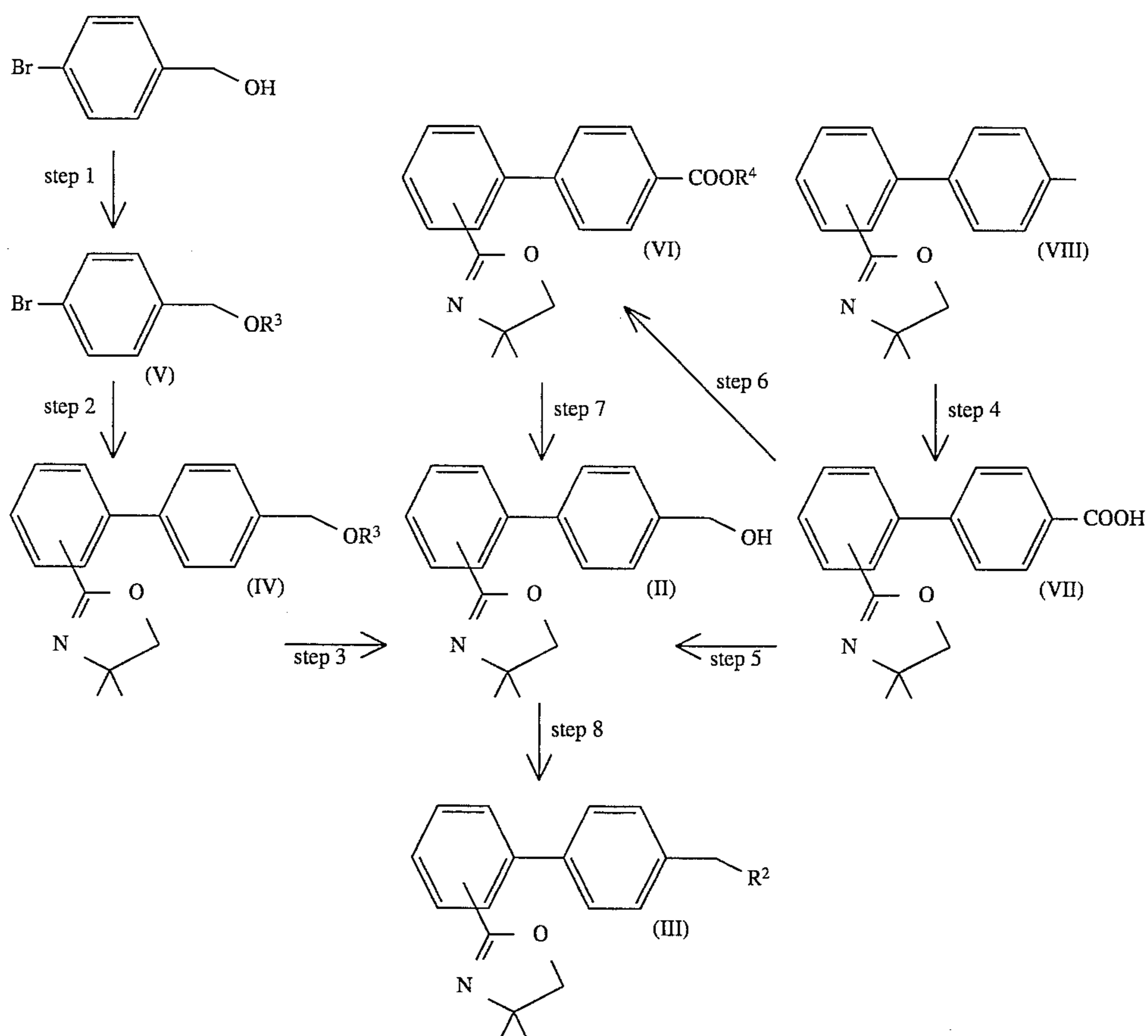
Reaction Scheme-6
