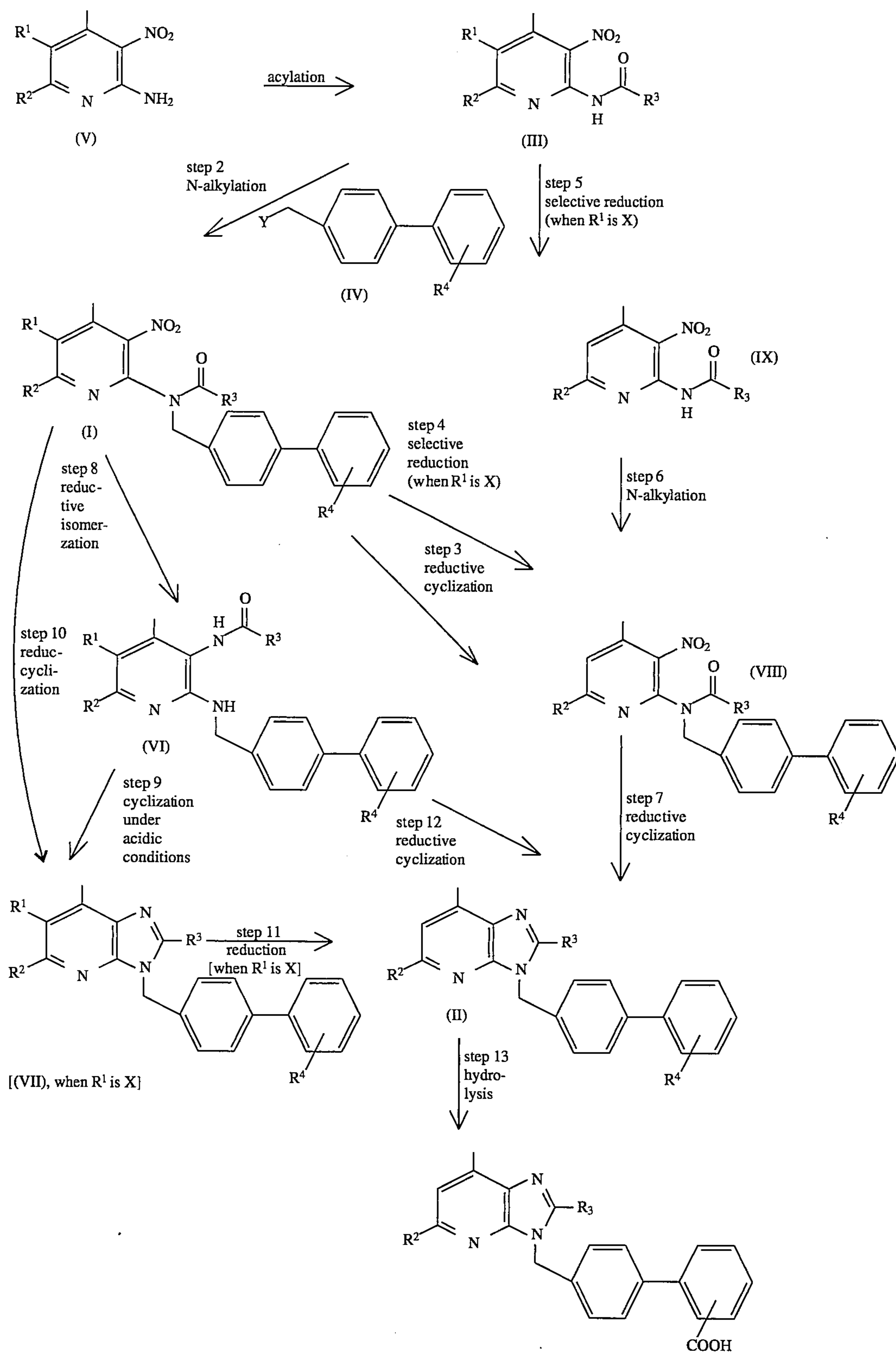
Reaction Scheme-4
