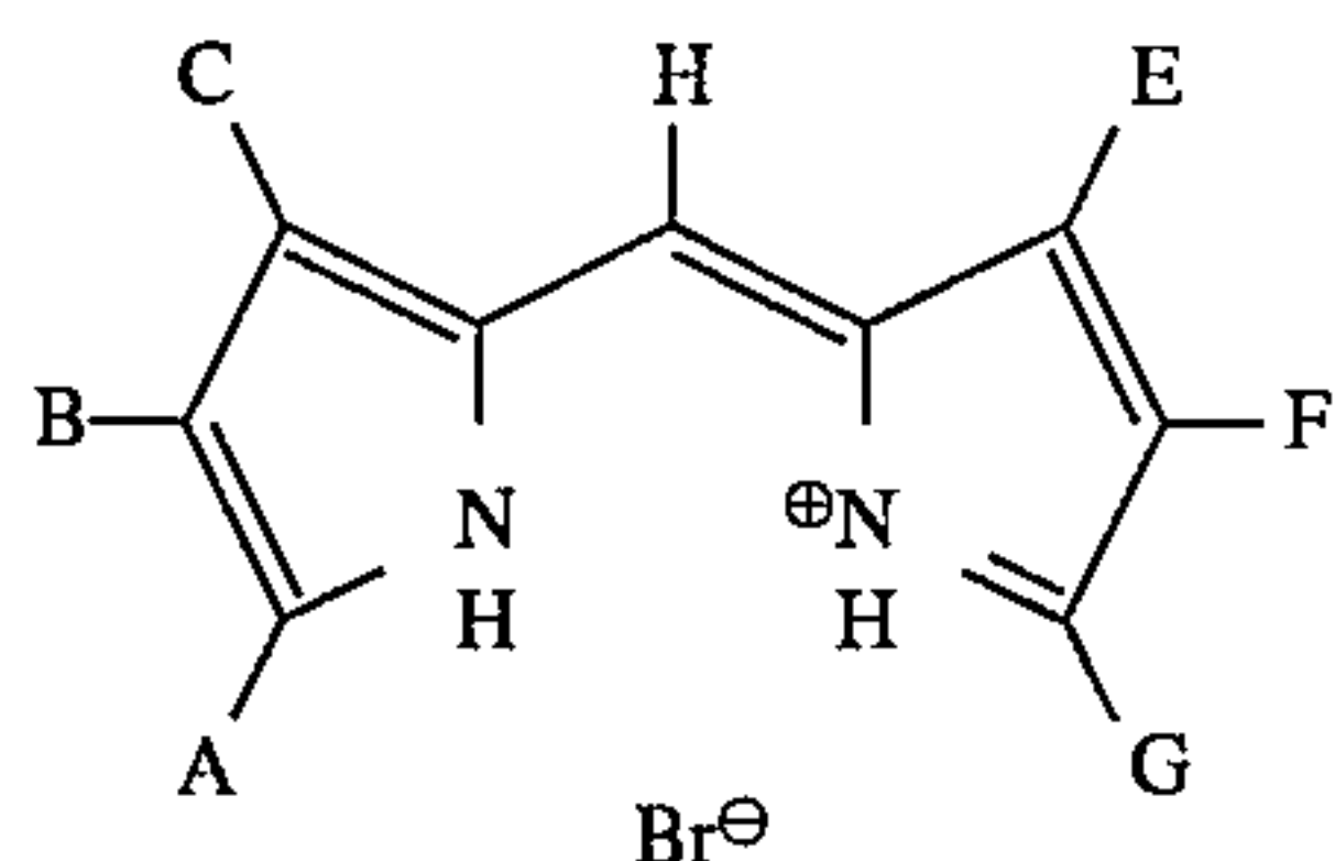
Dipyrromethenes
