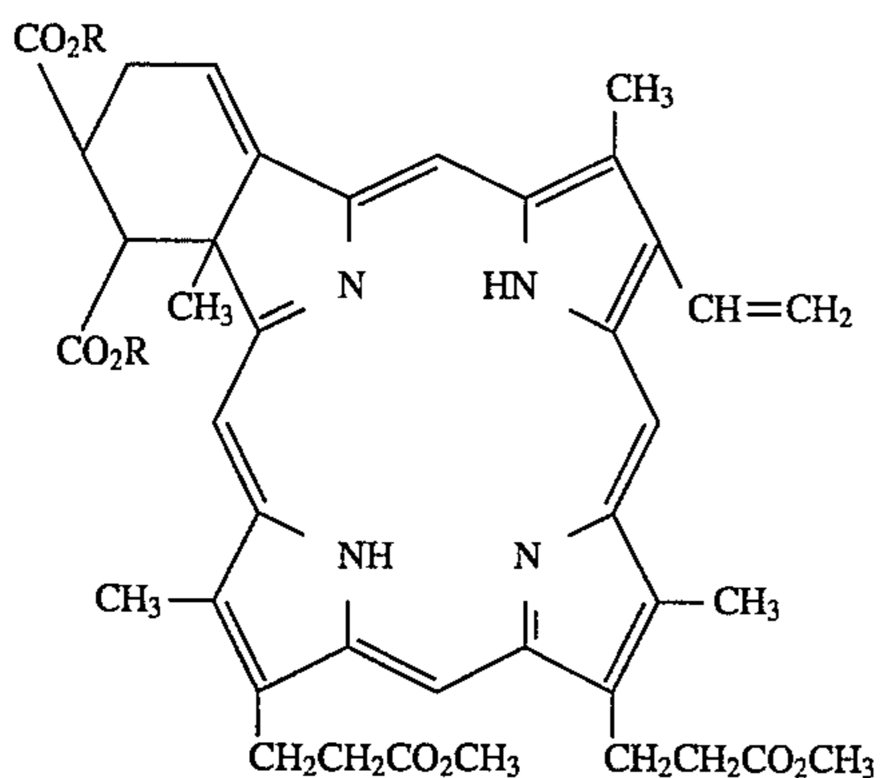
Adduct IX
