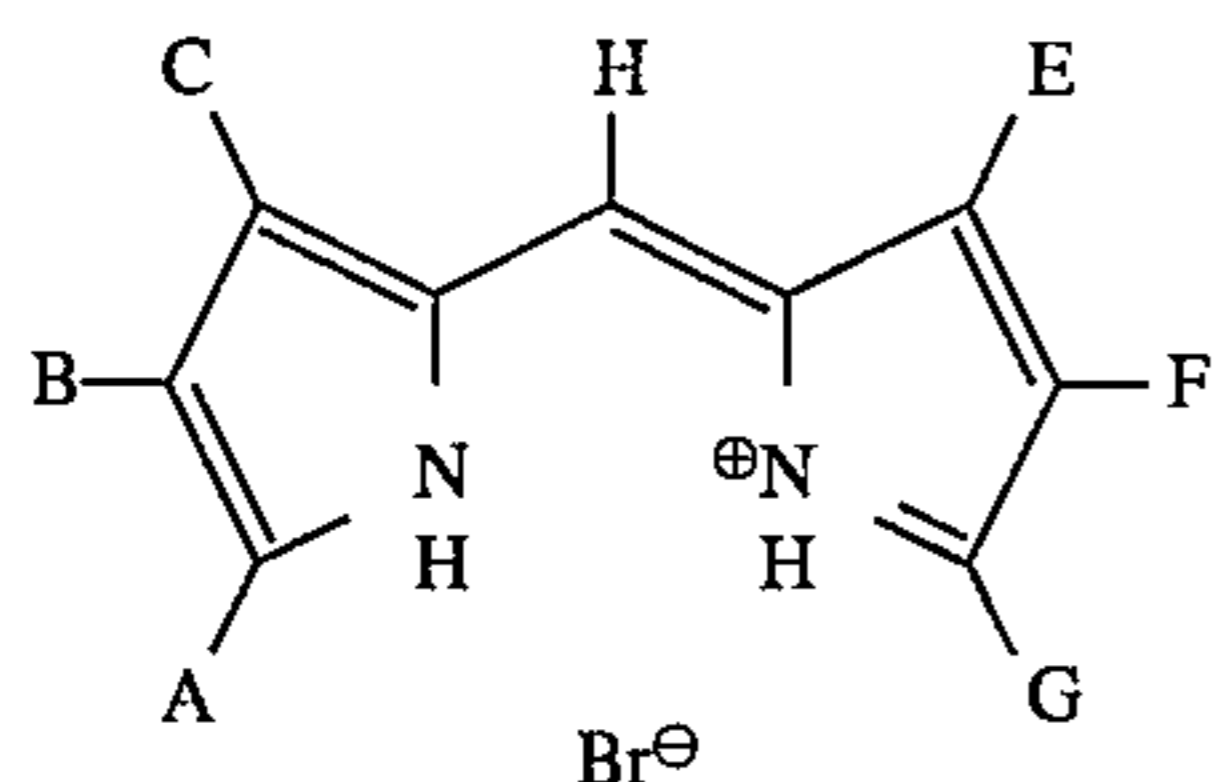
Dipyrromethenes
