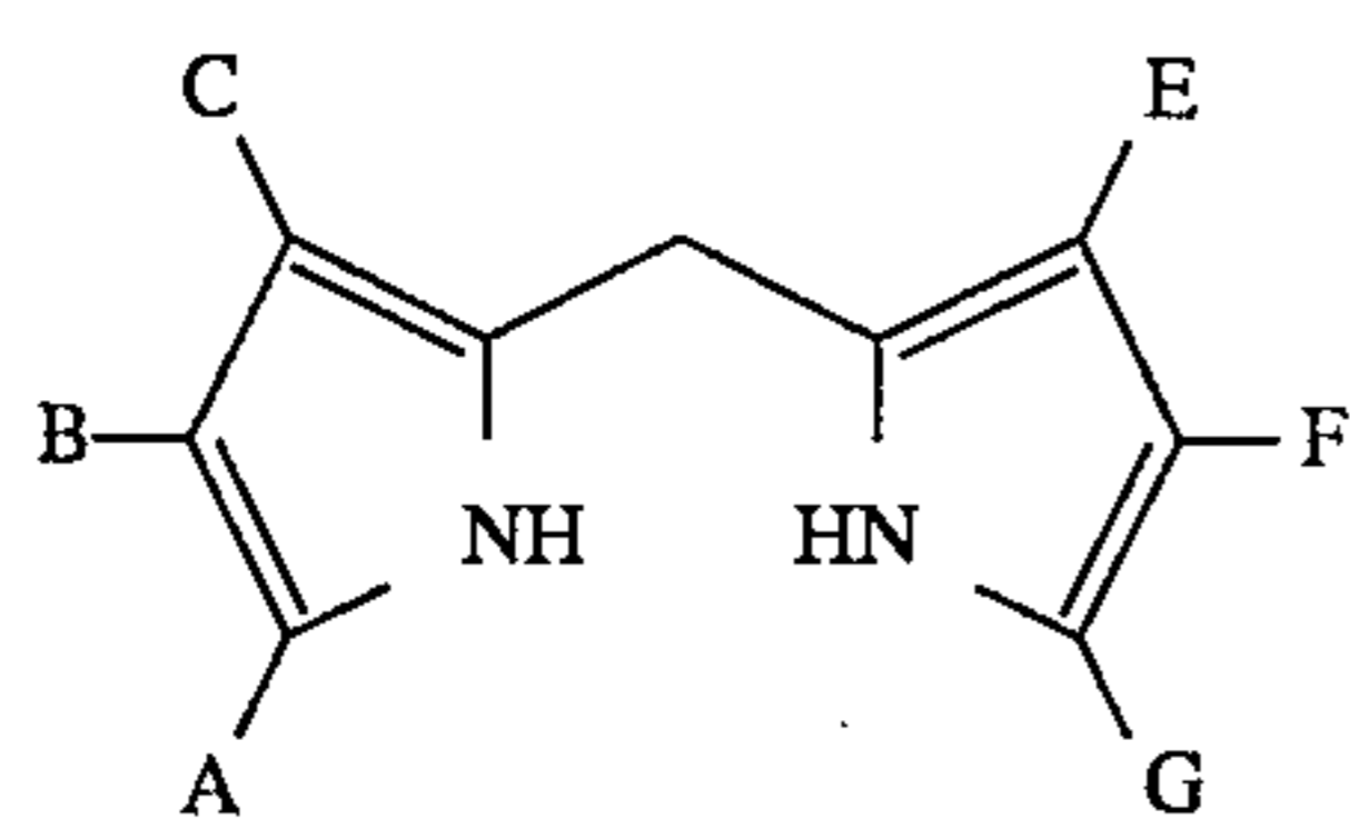
Dipyrromethanes
