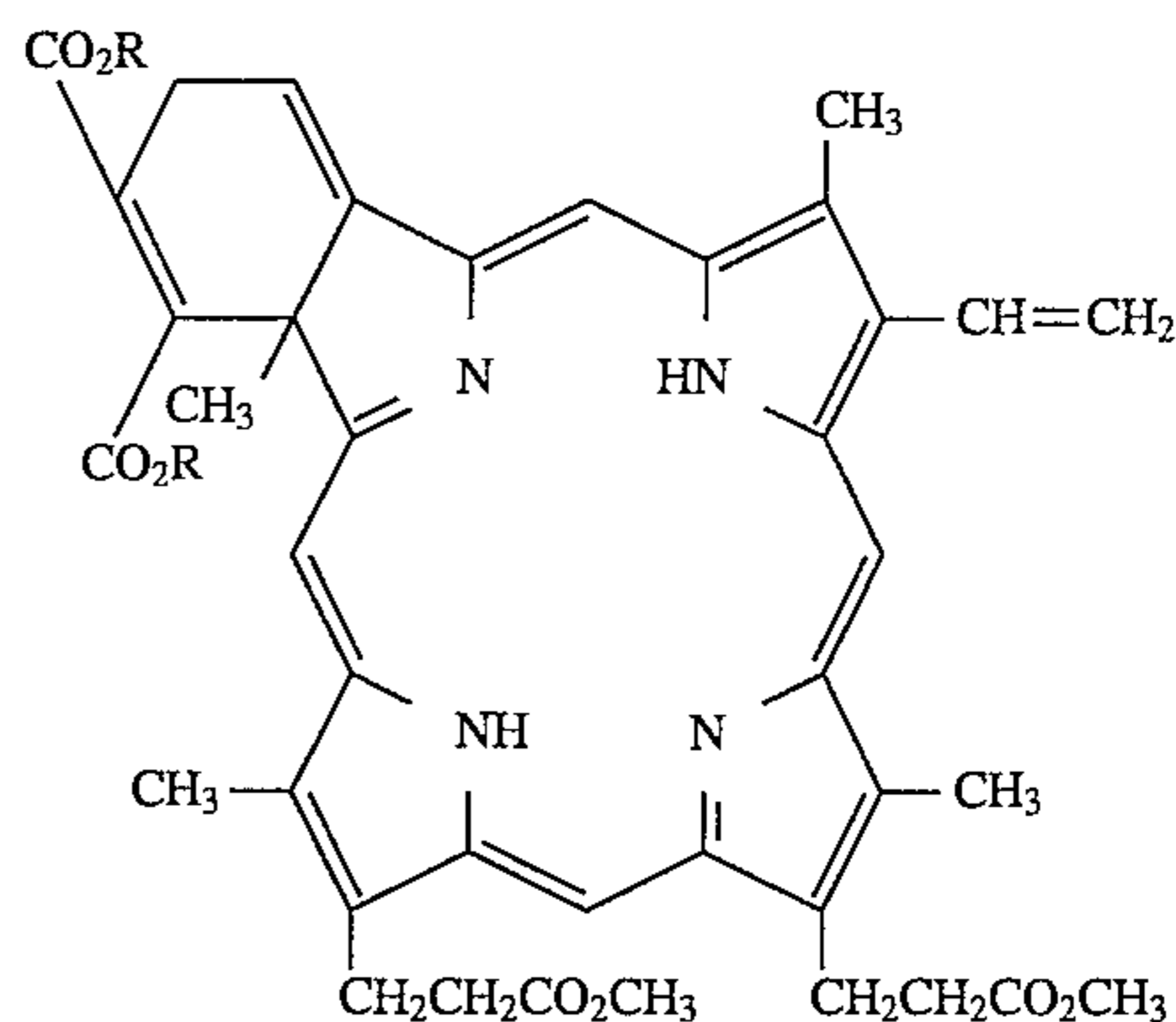
Adduct V
