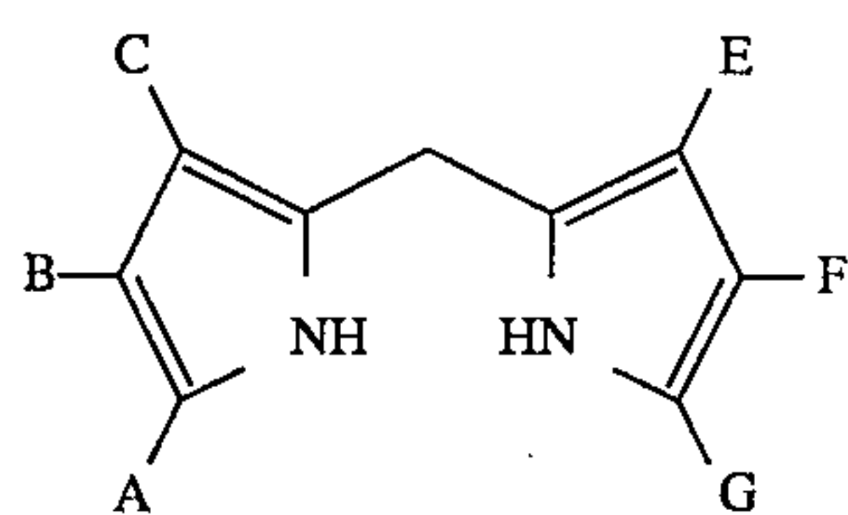
Dipyrromethanes
