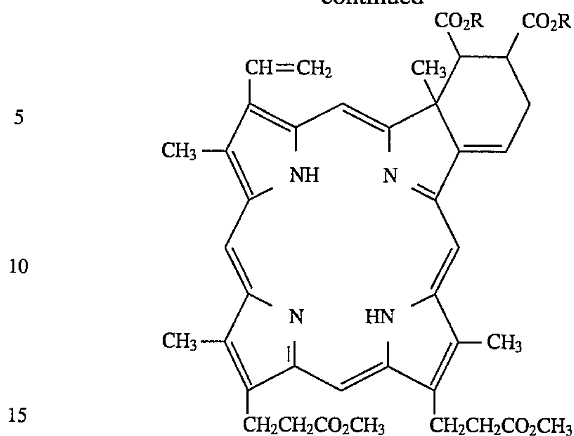
Adduct X
