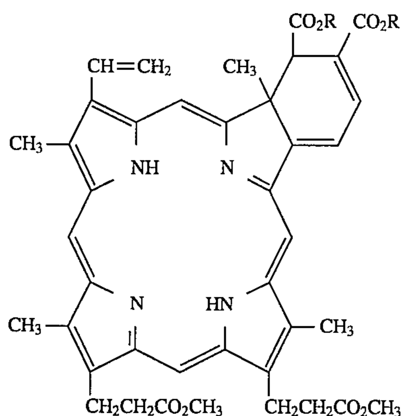
Adduct VIII
