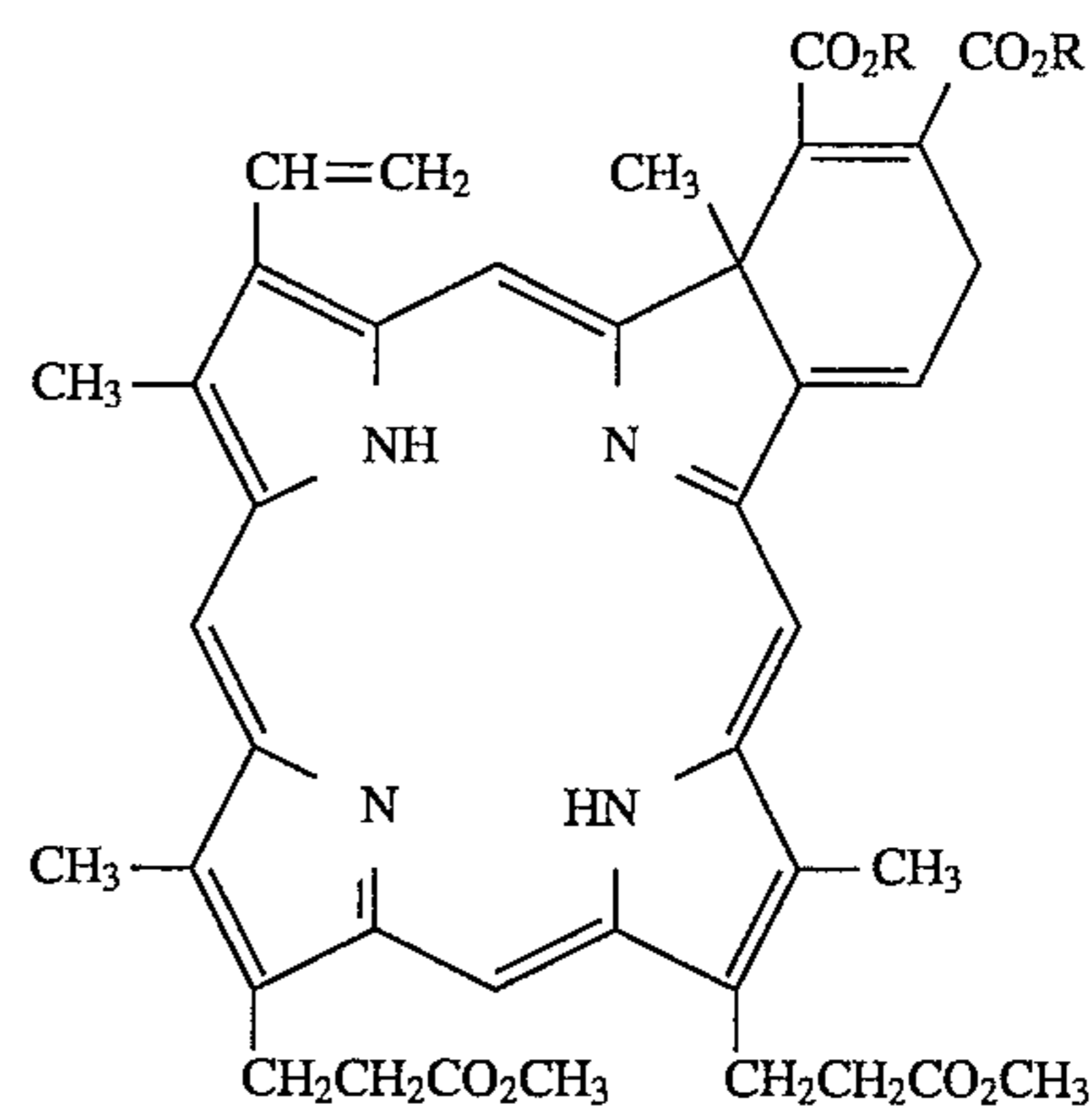
Adduct VI
