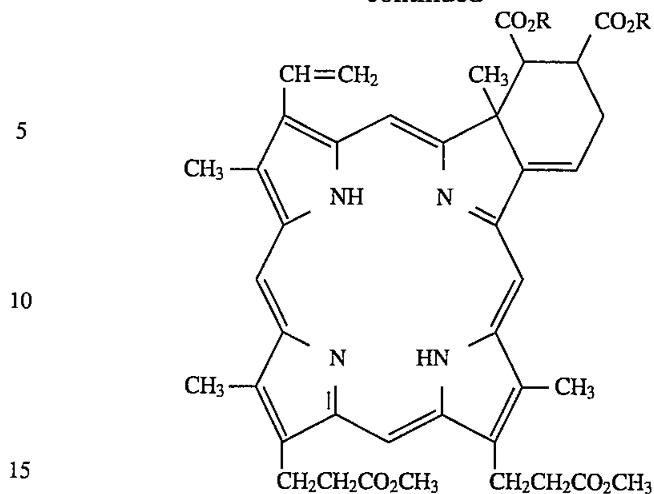
Adduct X
