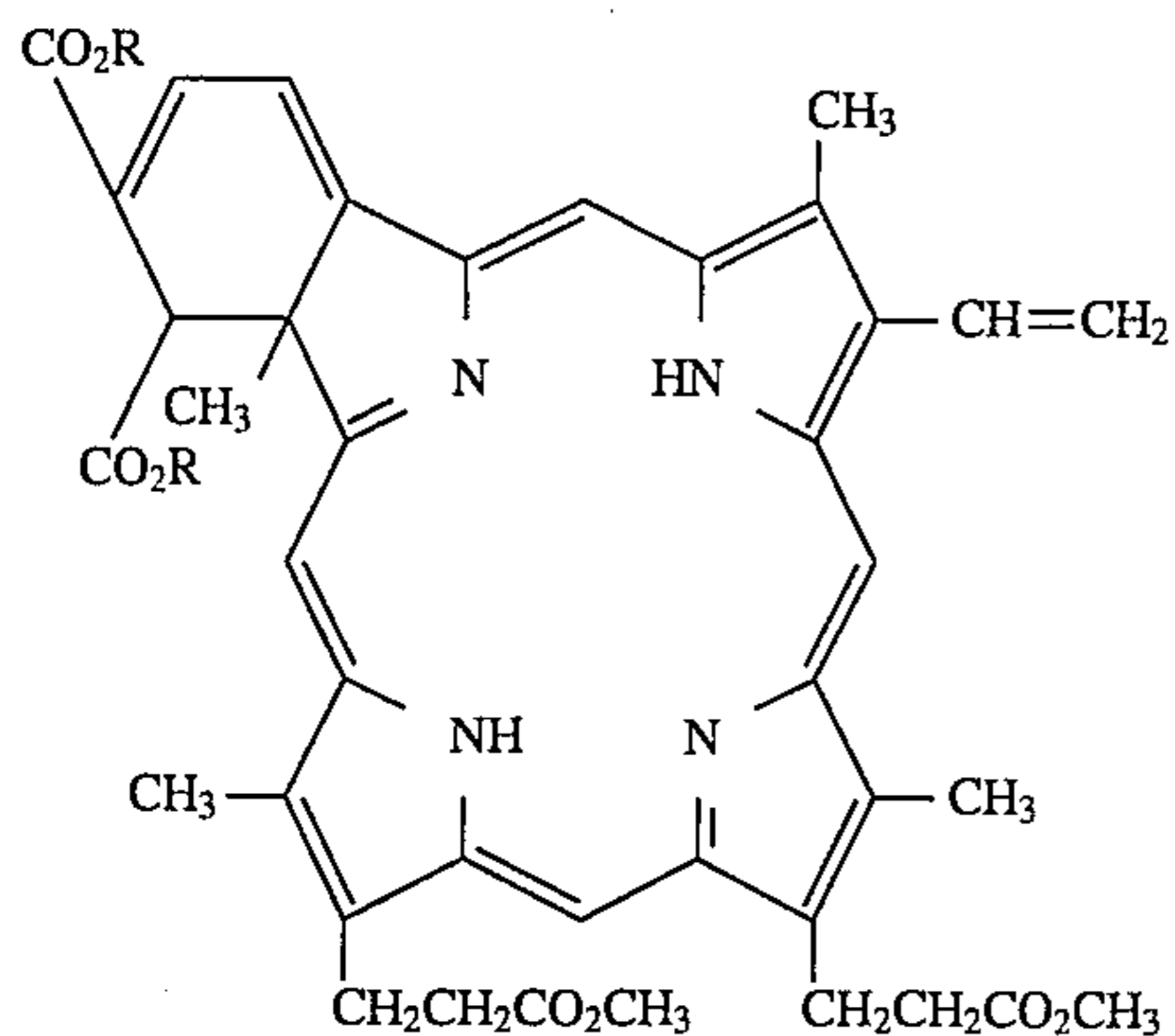
Adduct VII
