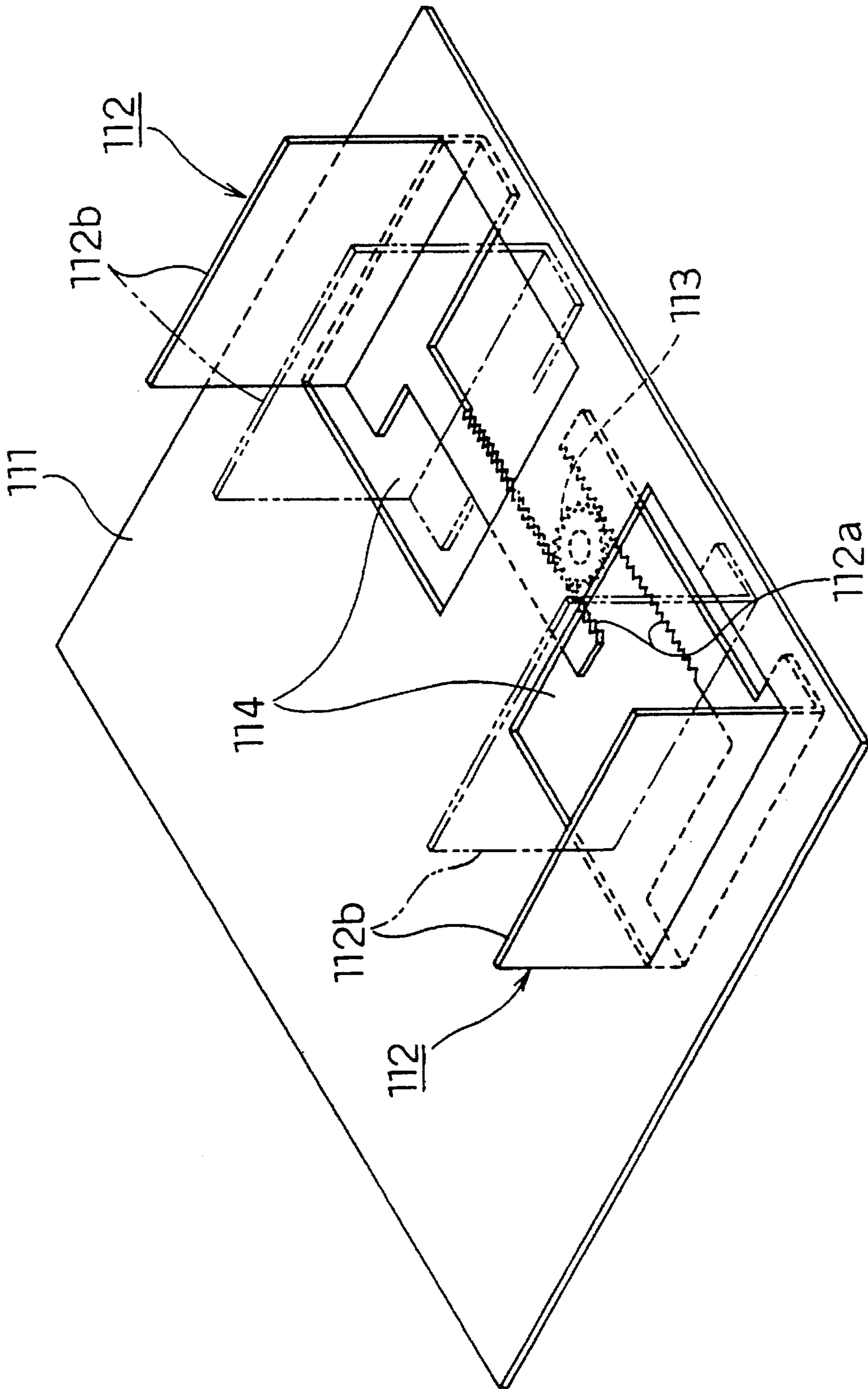
FIG. 3 PRIOR ART
