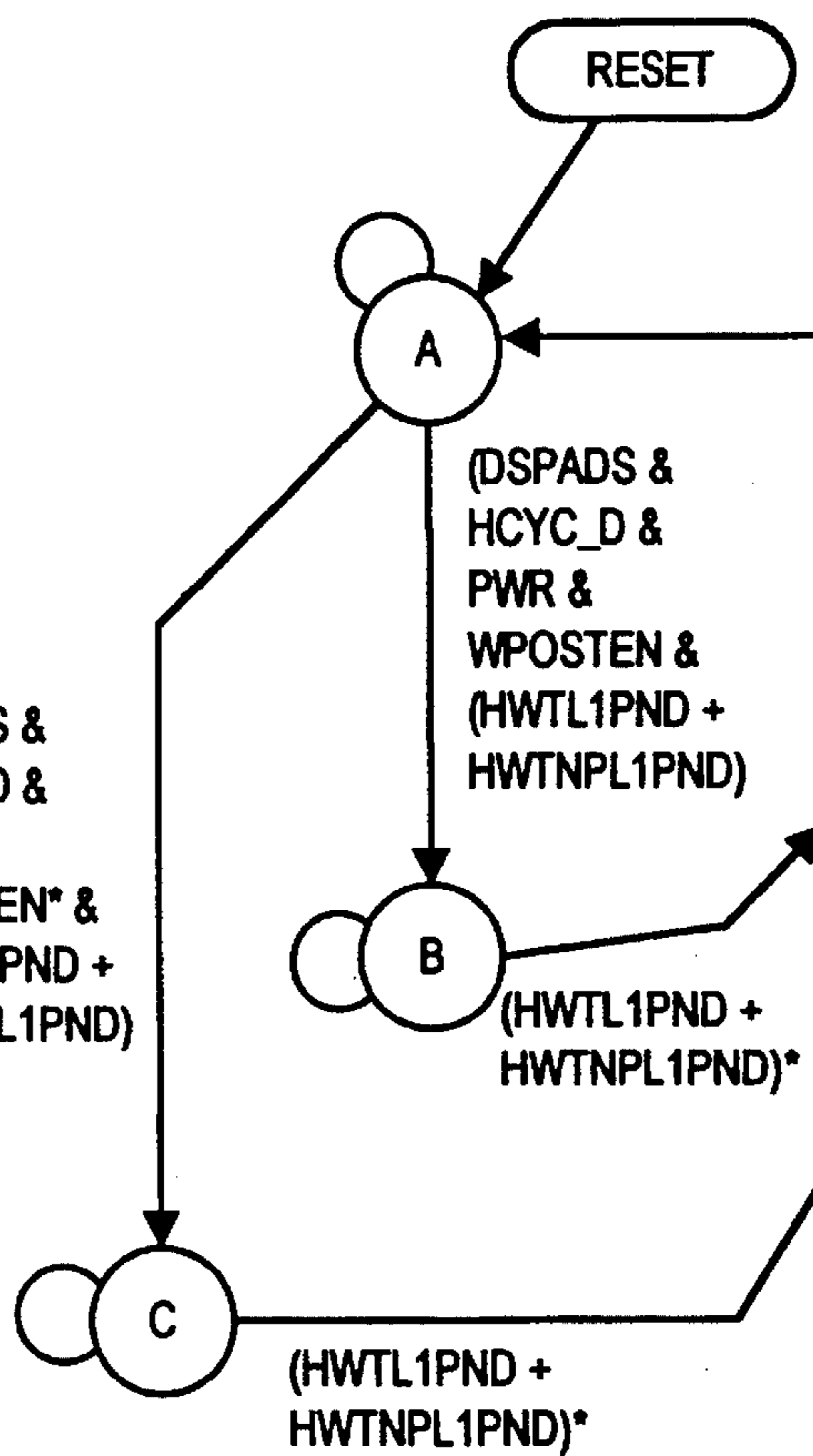
HWL2PND STATE MACHINE
