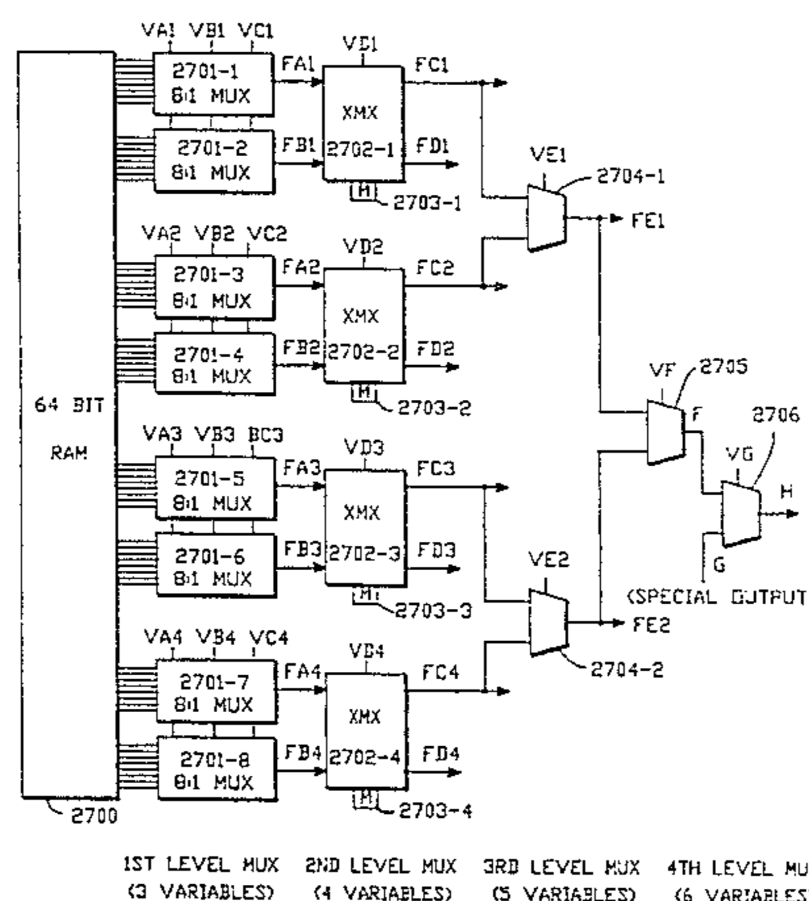
CLB CONFIGURATION
