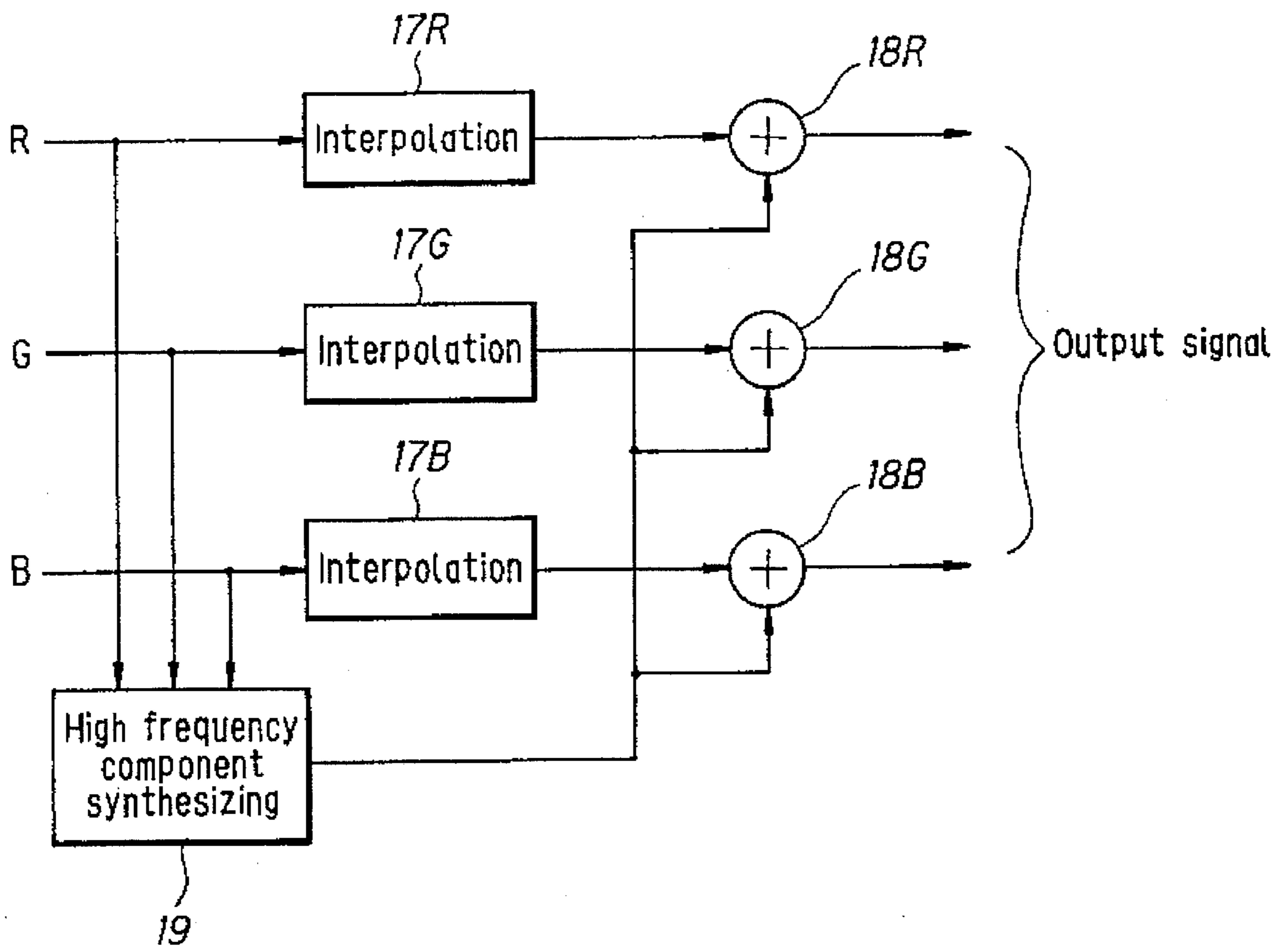
CONFIGURATION OF HD CIRCUIT
