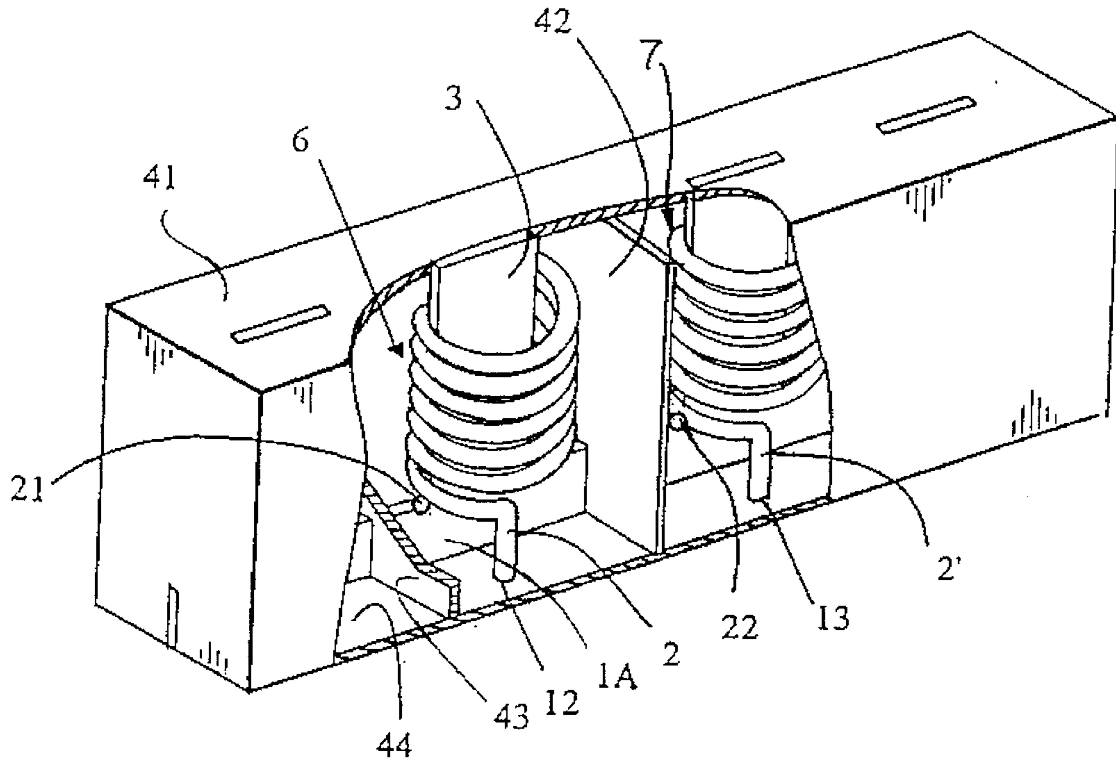
Fig. 4 PRIOR ART
