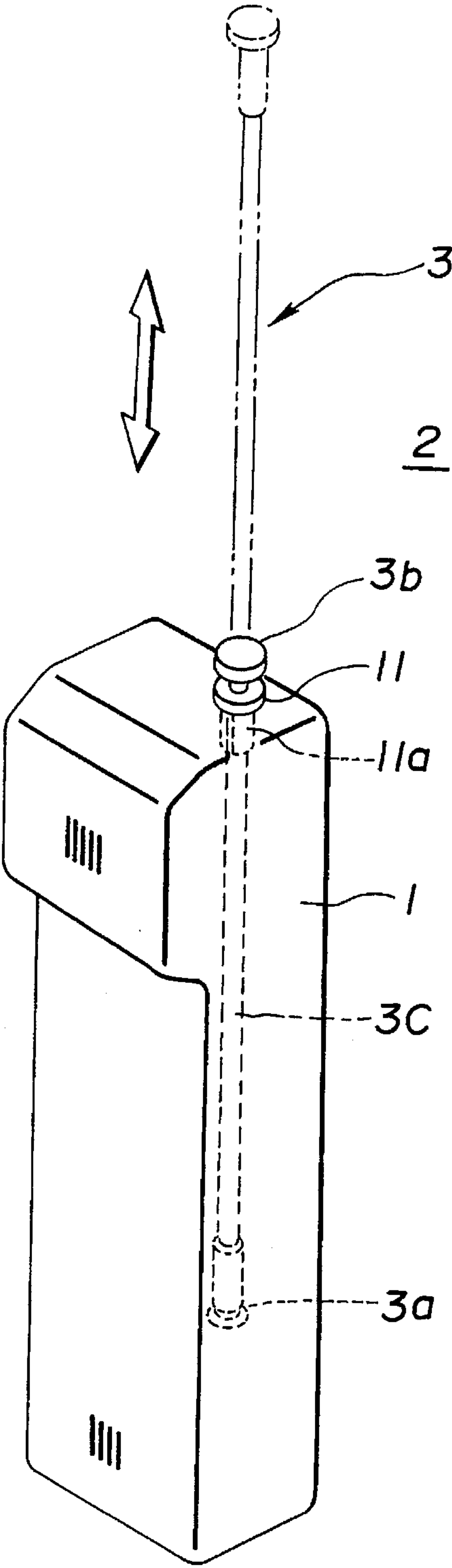
FIG.10 (PRIOR ART)
