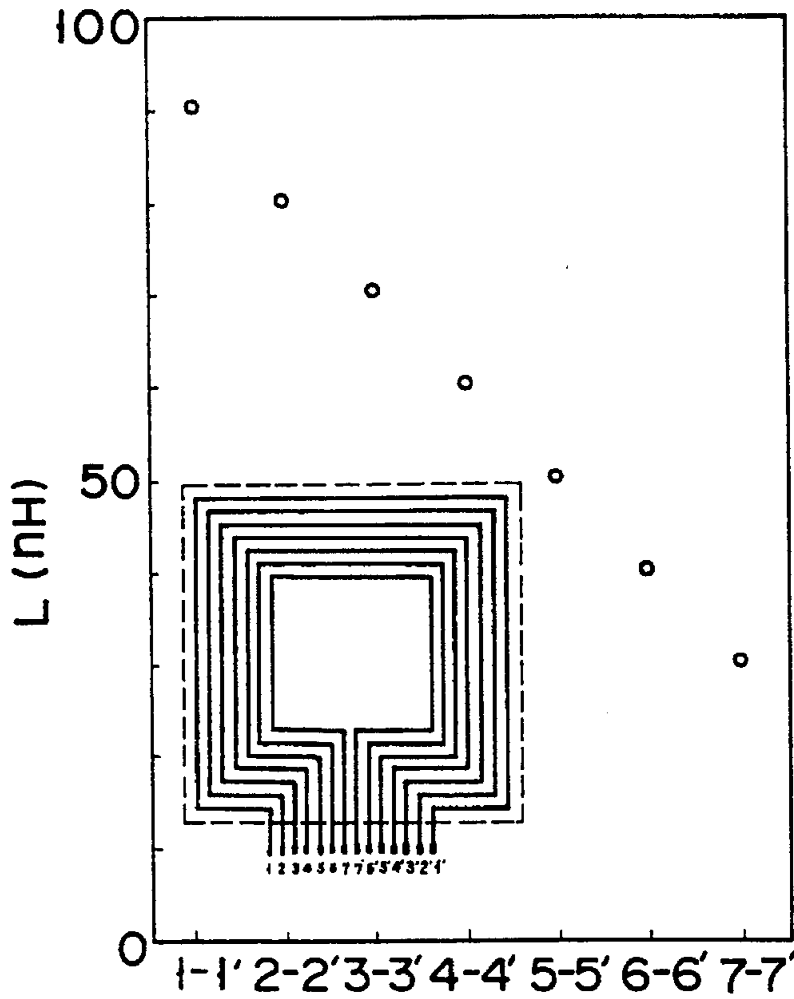
EXTERNAL TERMINAL OF 1 TURN PLANAR COIL
