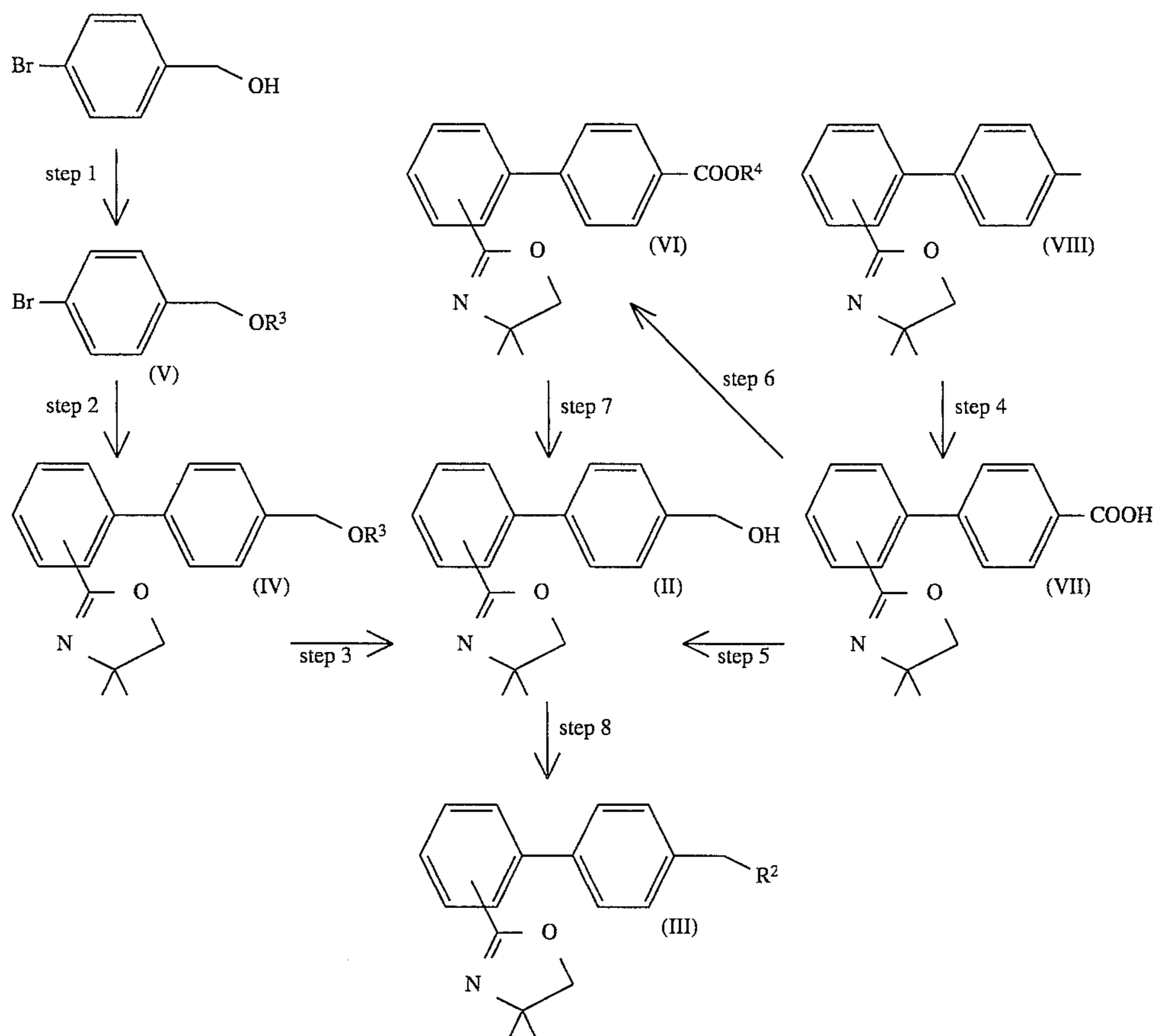
Reaction Scheme-6
