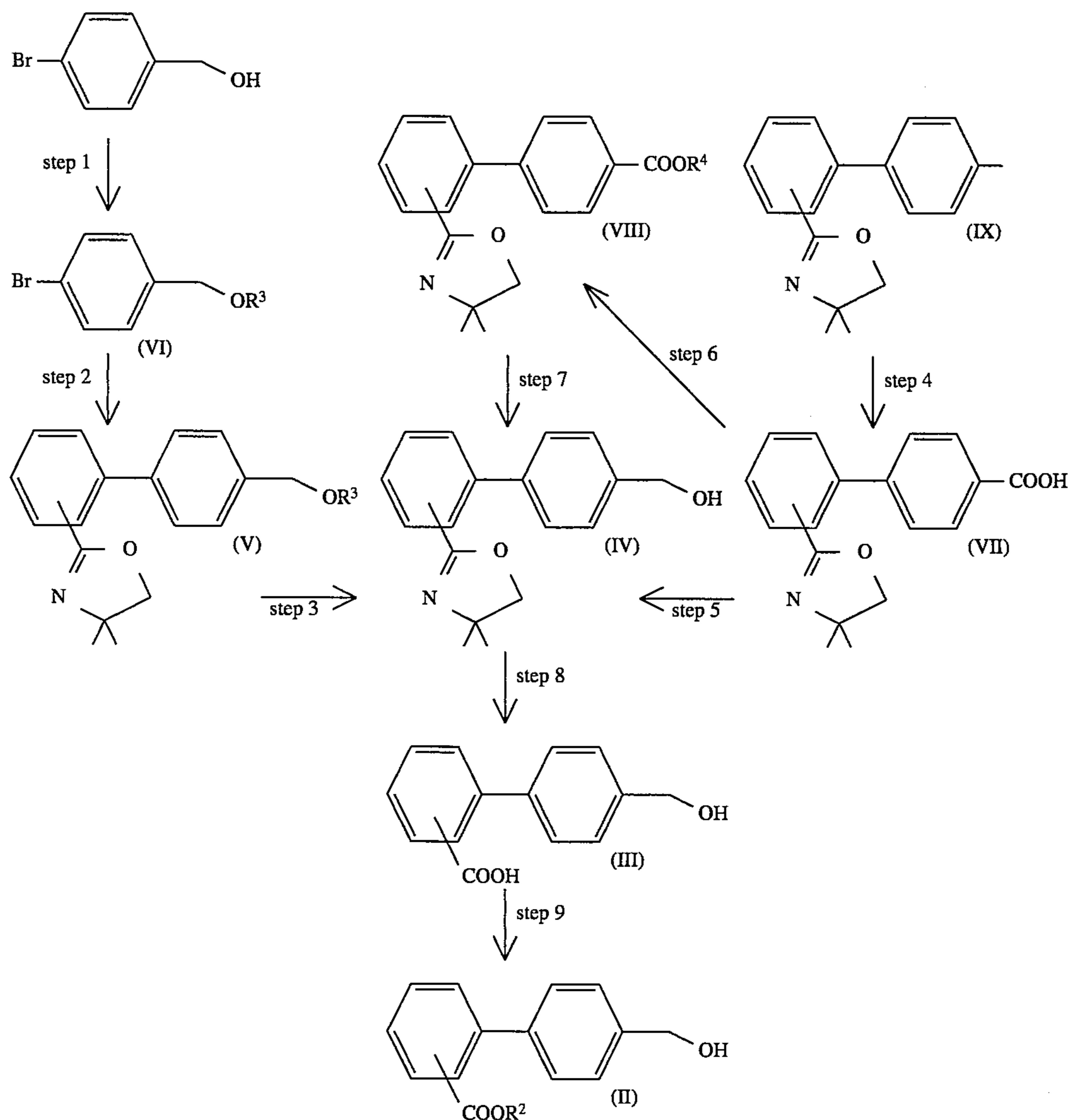
Reaction Scheme-7
