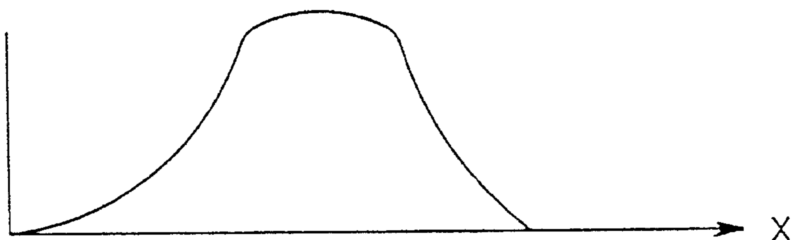
COATING DISTRIBUTION W/PRIMARY GAS DIRECTOR ONLY
