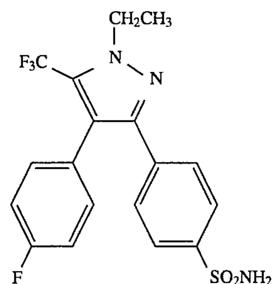
4-[1-Ethyl-4-(4-fluorophenyl)-5-(trifluoromethyl)-1H-pyrazol-3-yl]benzenesulfonamide
