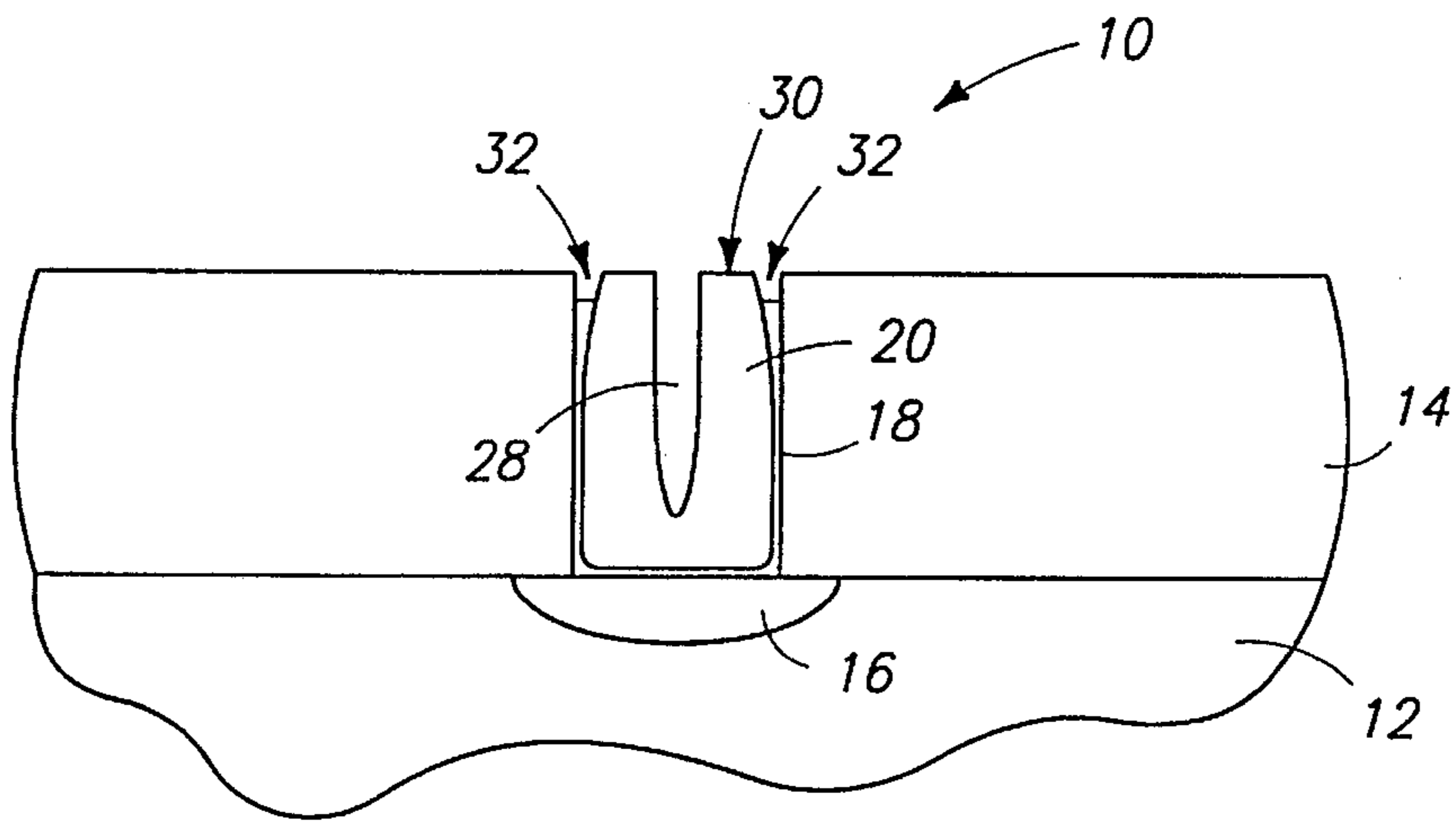
FIG. 2 PRIOR ART
