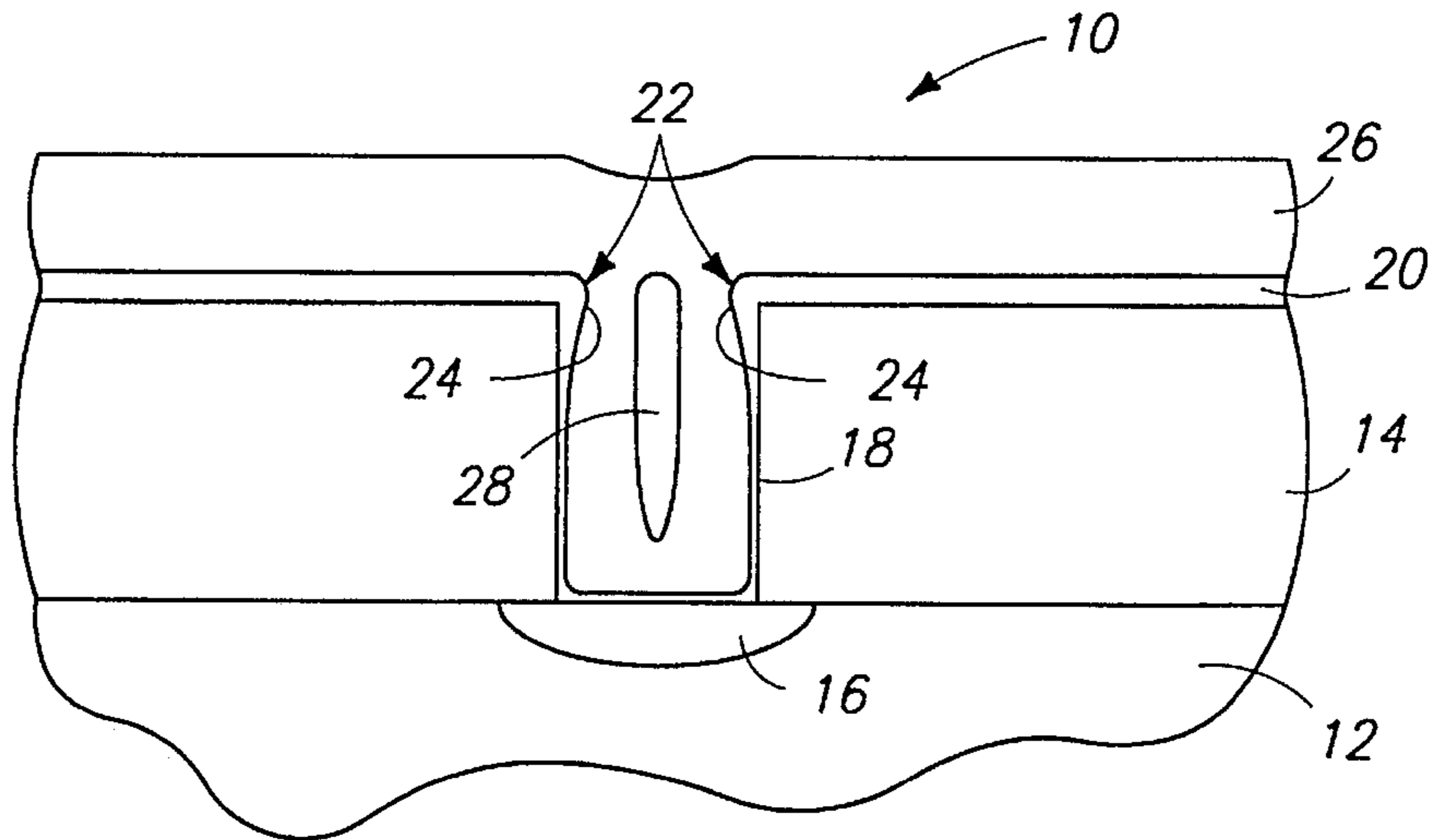
FIG. 1 PRIOR ART
