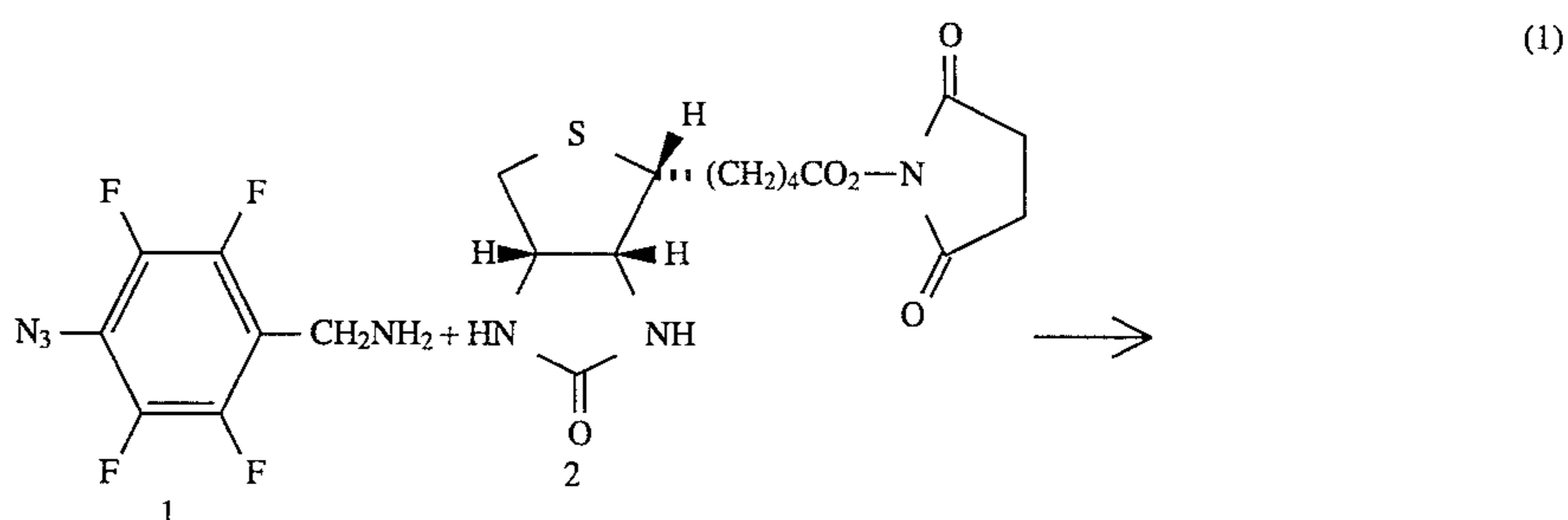
Scheme 11
