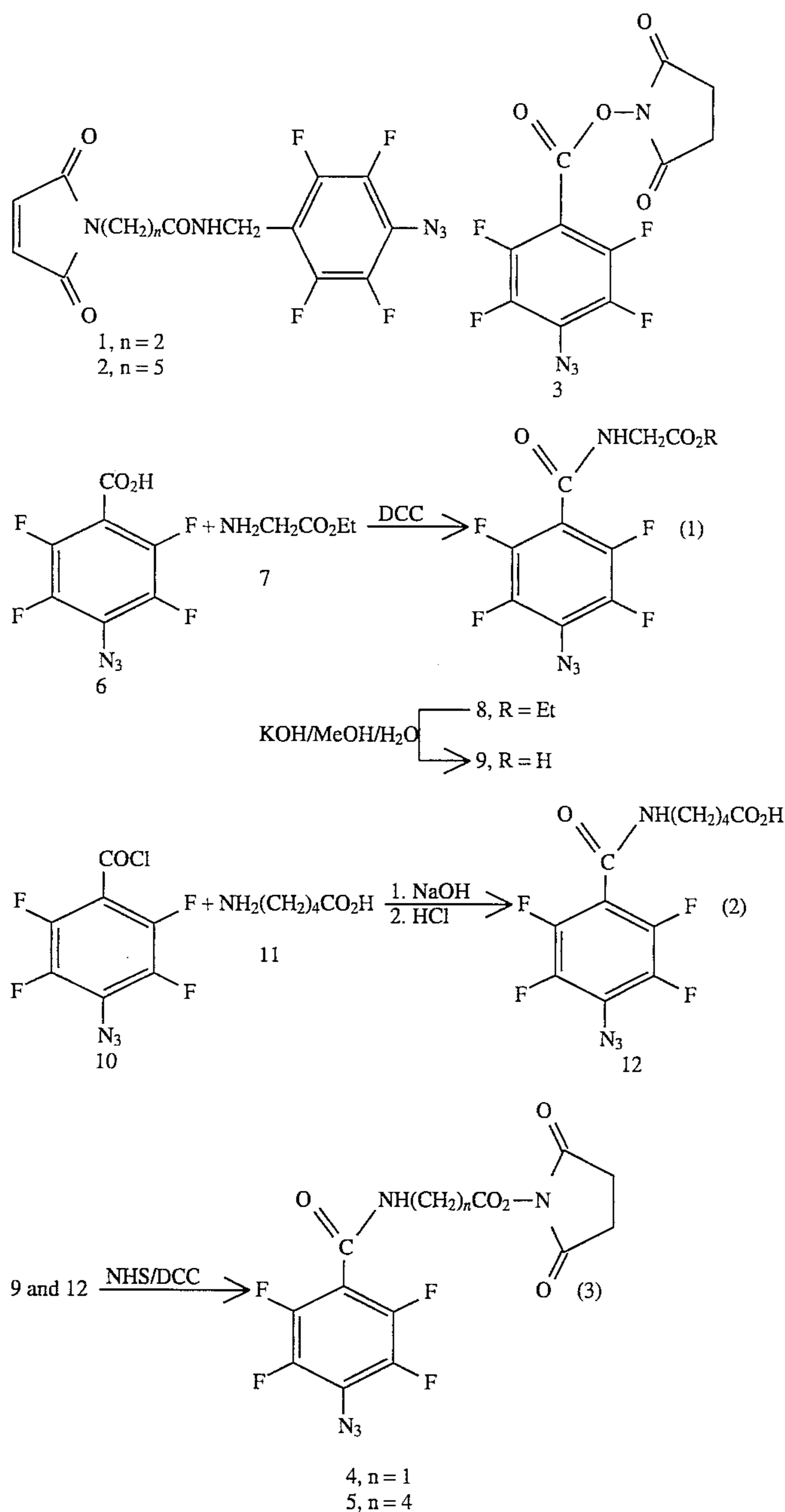
Scheme 12
