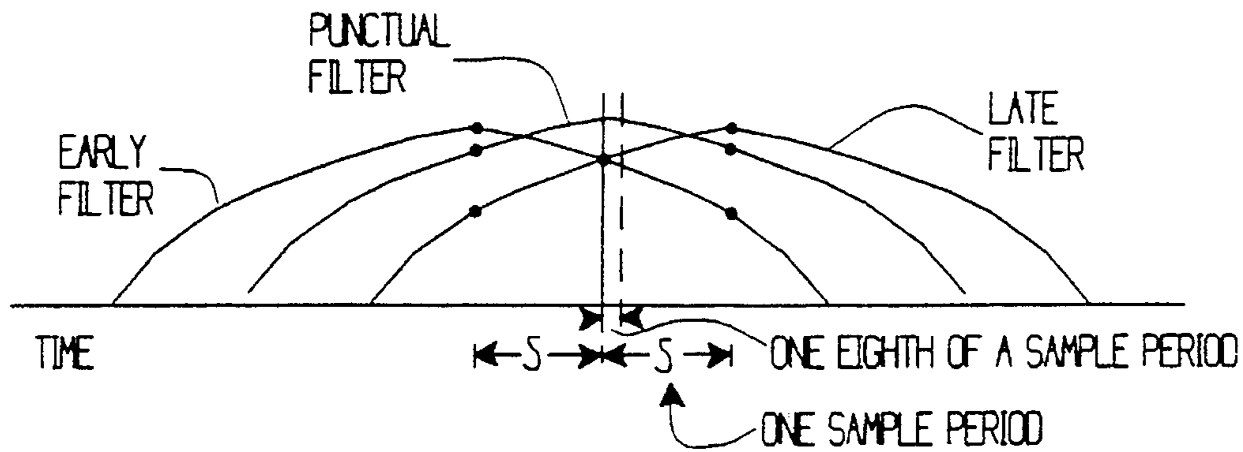
MATCHED FILTER SAMPLE TIMING
