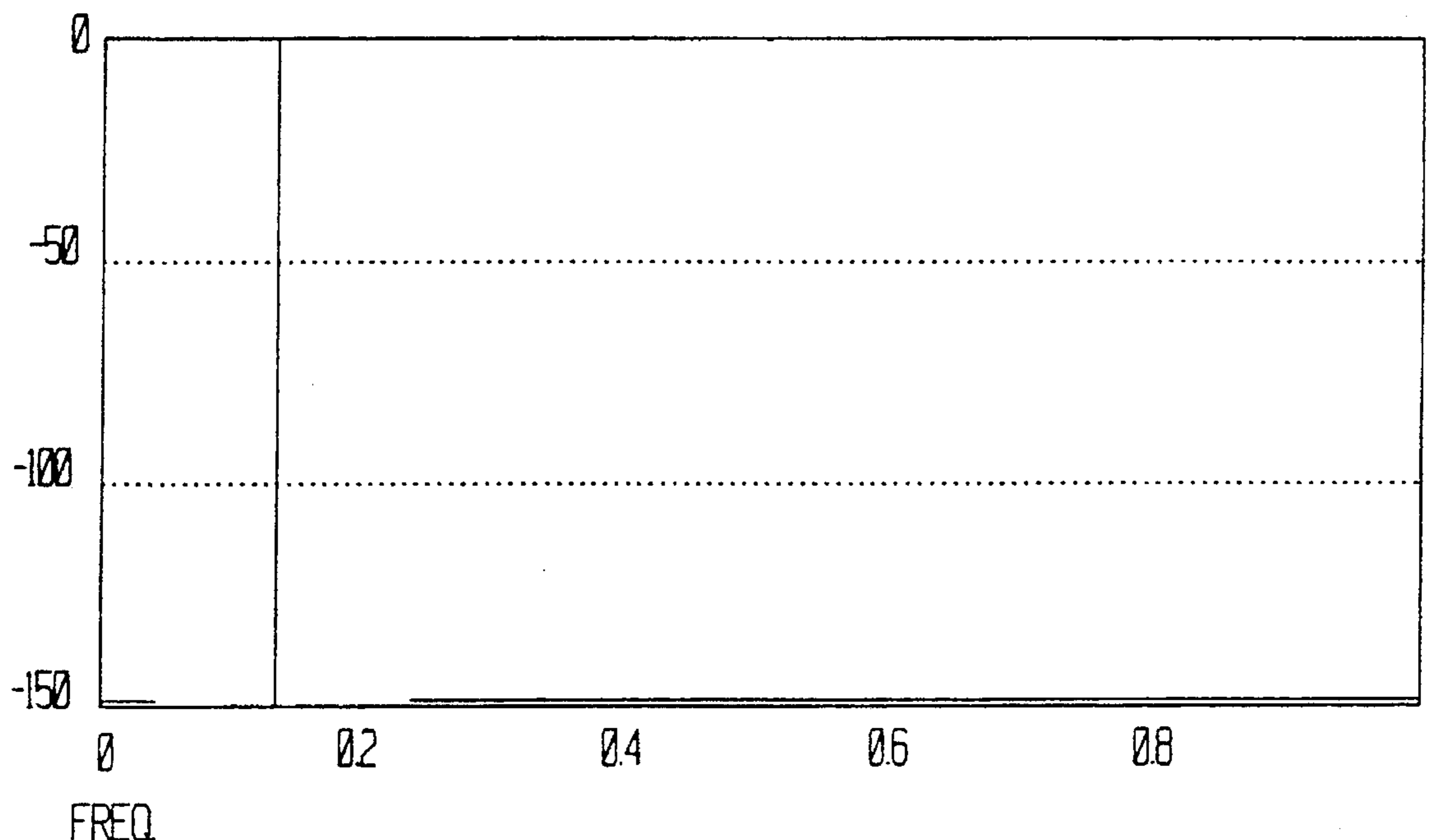
SPECTRUM OF NCO COMPLEX EXPONENTIAL VS. FREQUENCY NORMALIZED SAMPLE RATE SHOWS SPURIOUS IS -150 dB FROM SIGNAL
