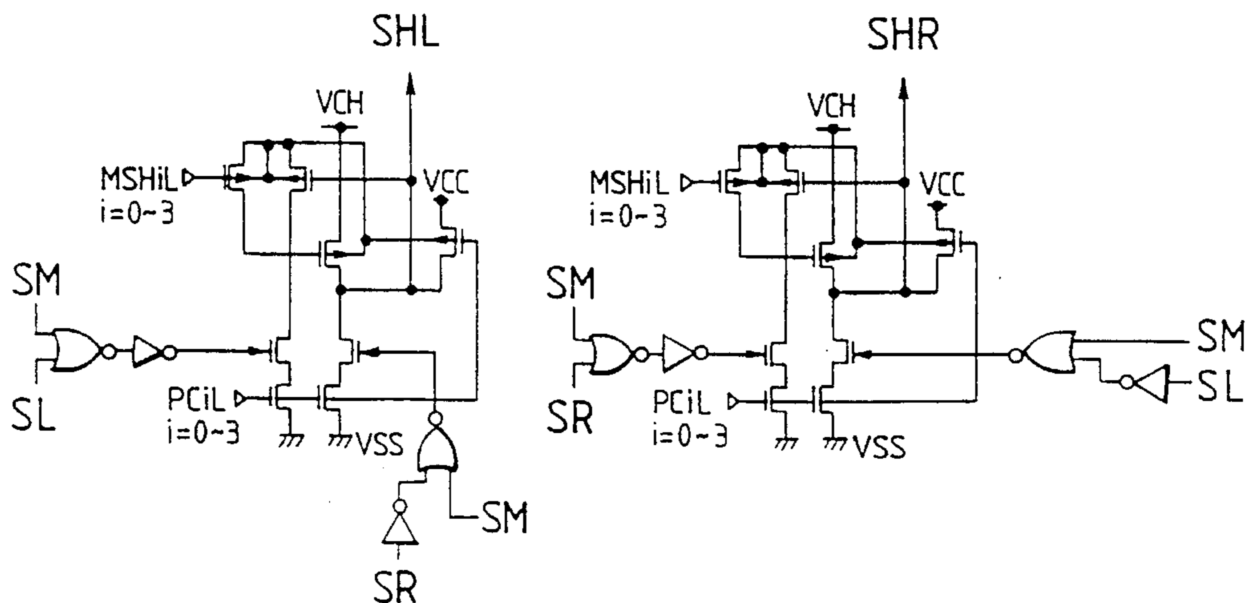
SHL/R GENERATOR
