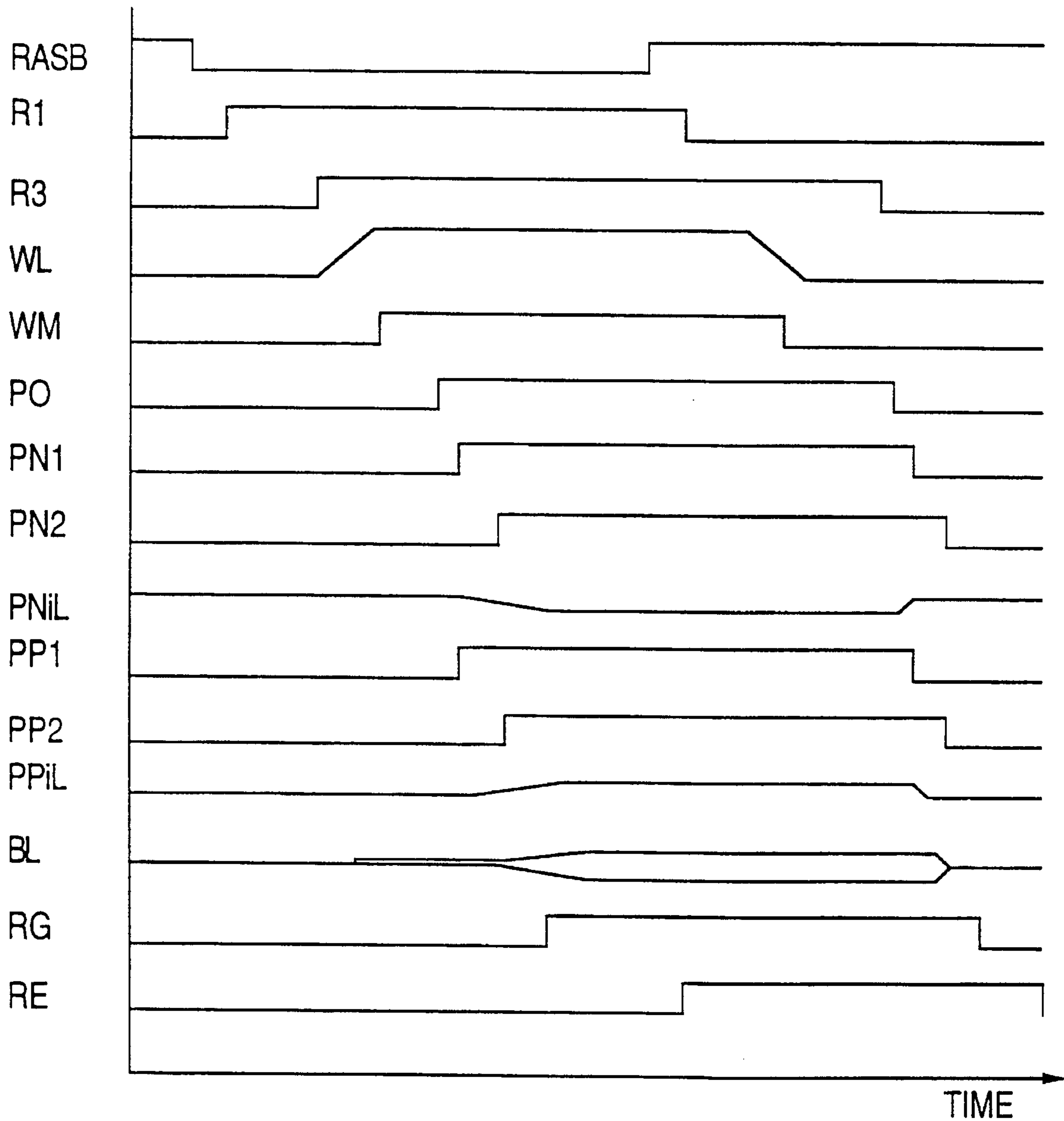
RAS SYSTEM (SENSE AMP-BL)
