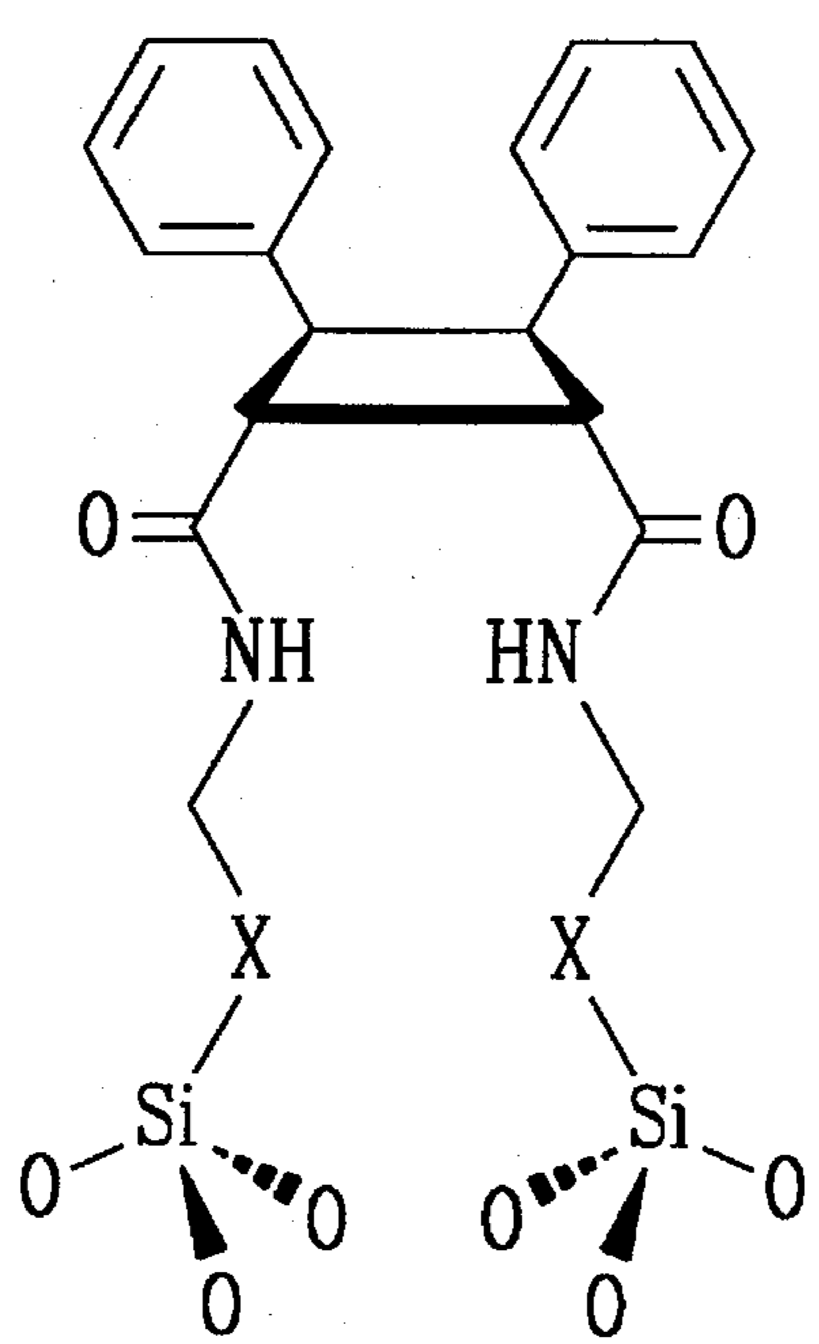
\beta -TRUXIAMIDE
