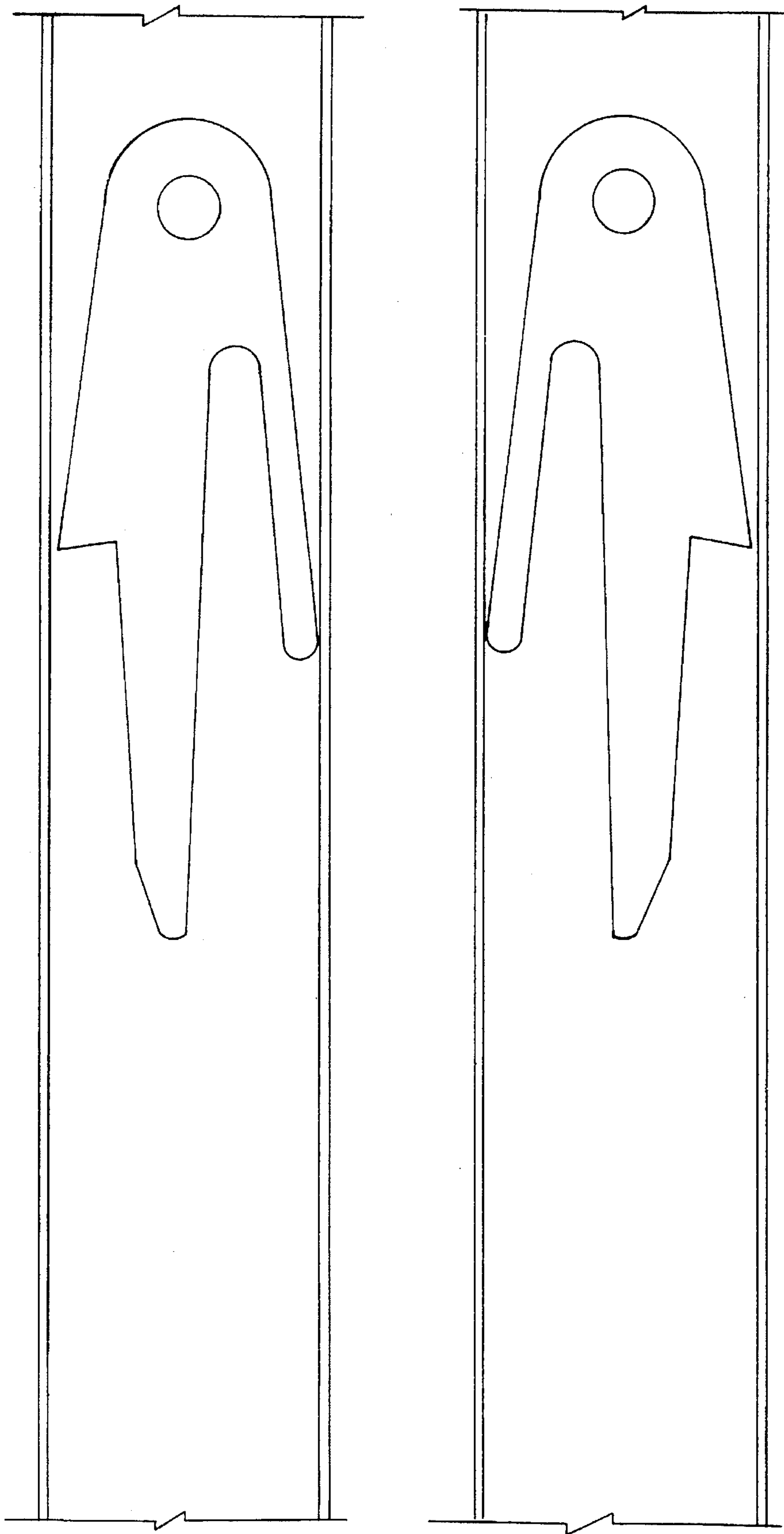
Fig. 2 PRIOR ART
