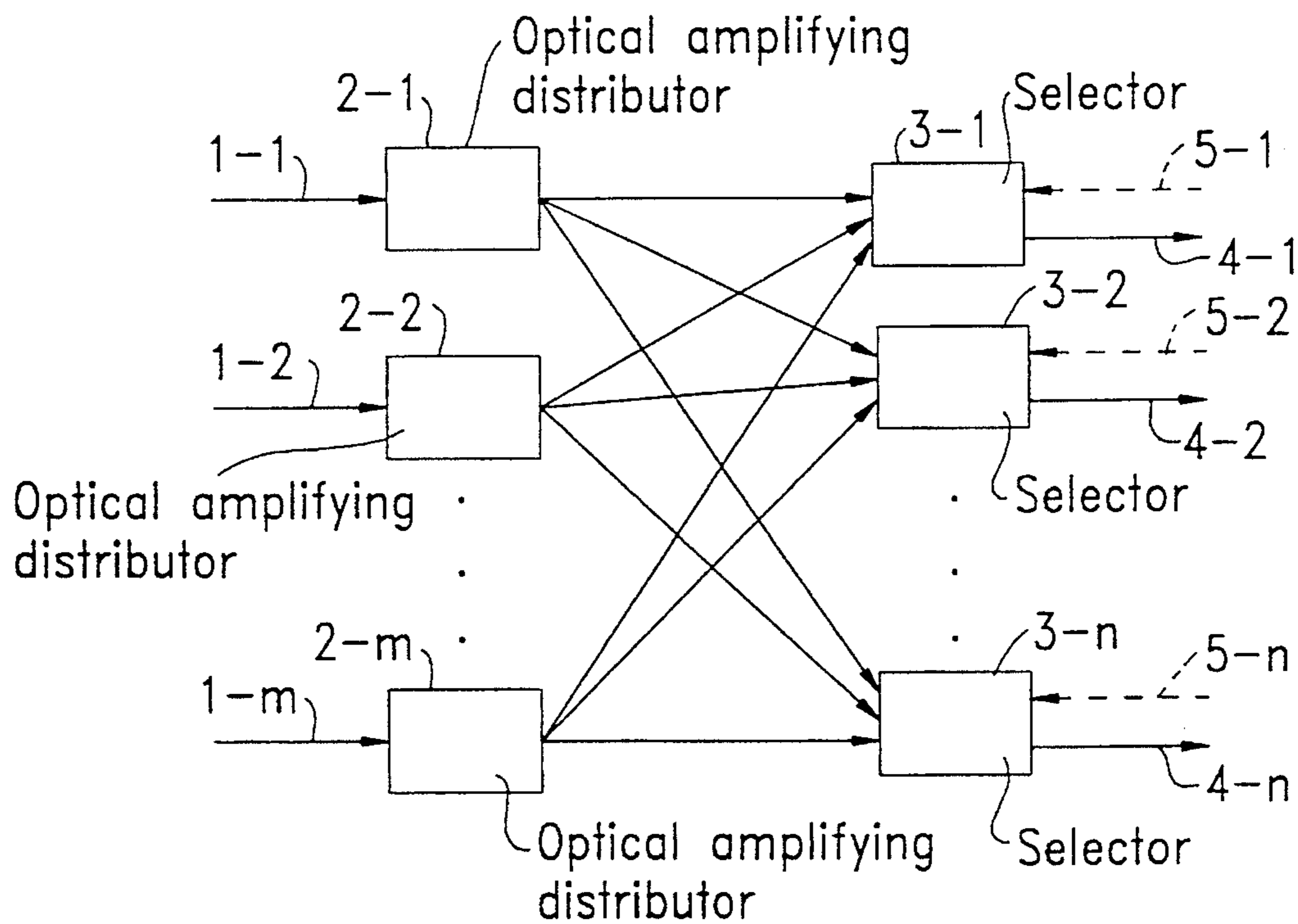
FIG. 2 Prior Art
