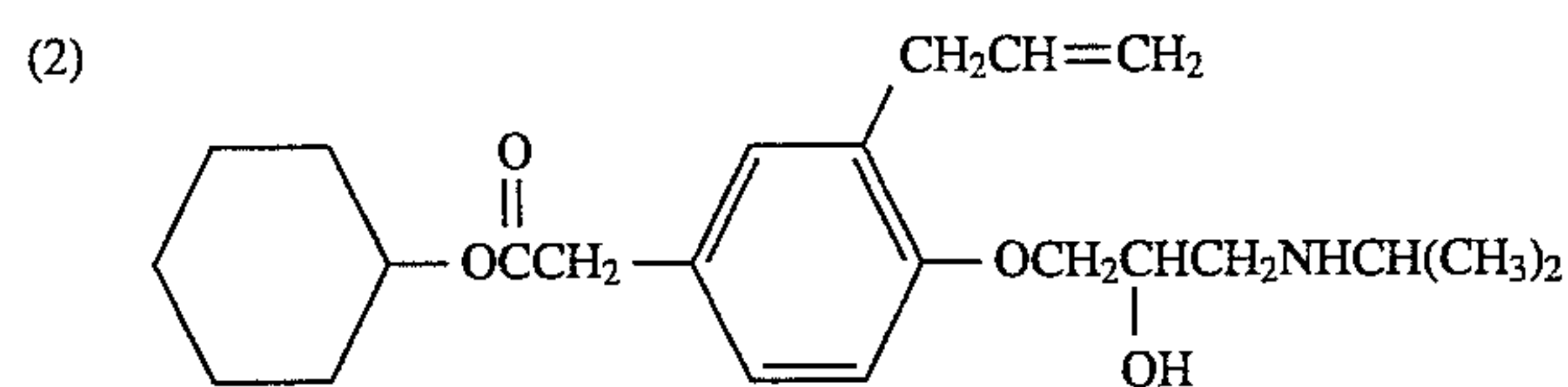
(AN ANALOGUE OF ALPRENOLOL)
