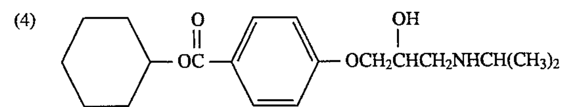
(AN ANALOGUE OF METOPROLOL)
