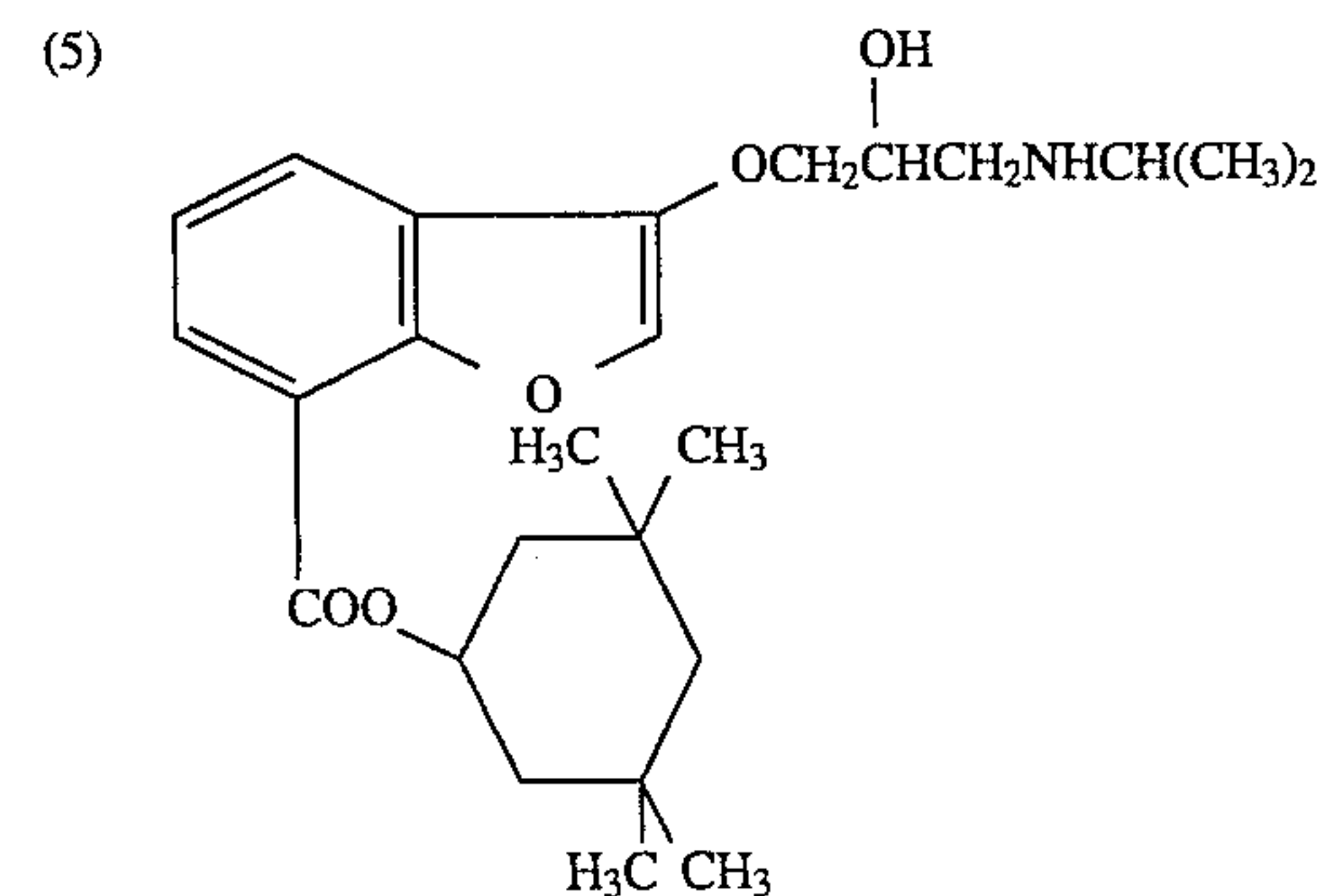
(AN ANALOGUE OF BUFUROLOL)
