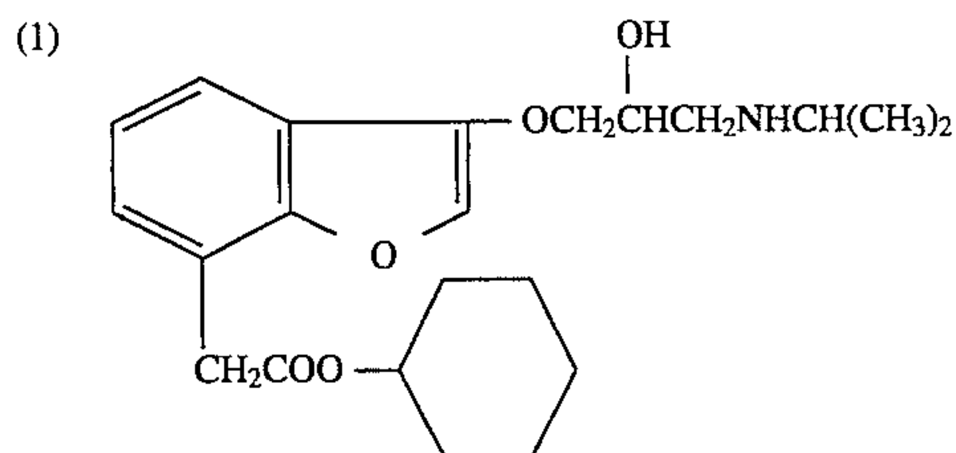
(AN ANALOGUE OF BUFUROLOL)
