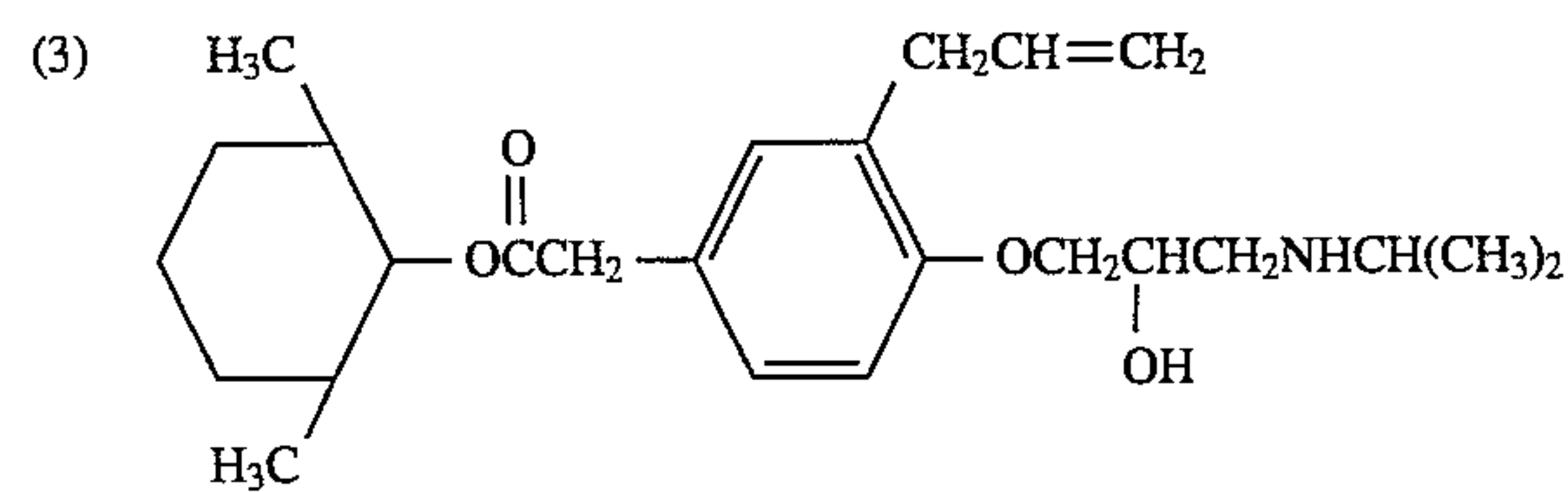
(AN ANALOGUE OF ALPRENOLOL)
