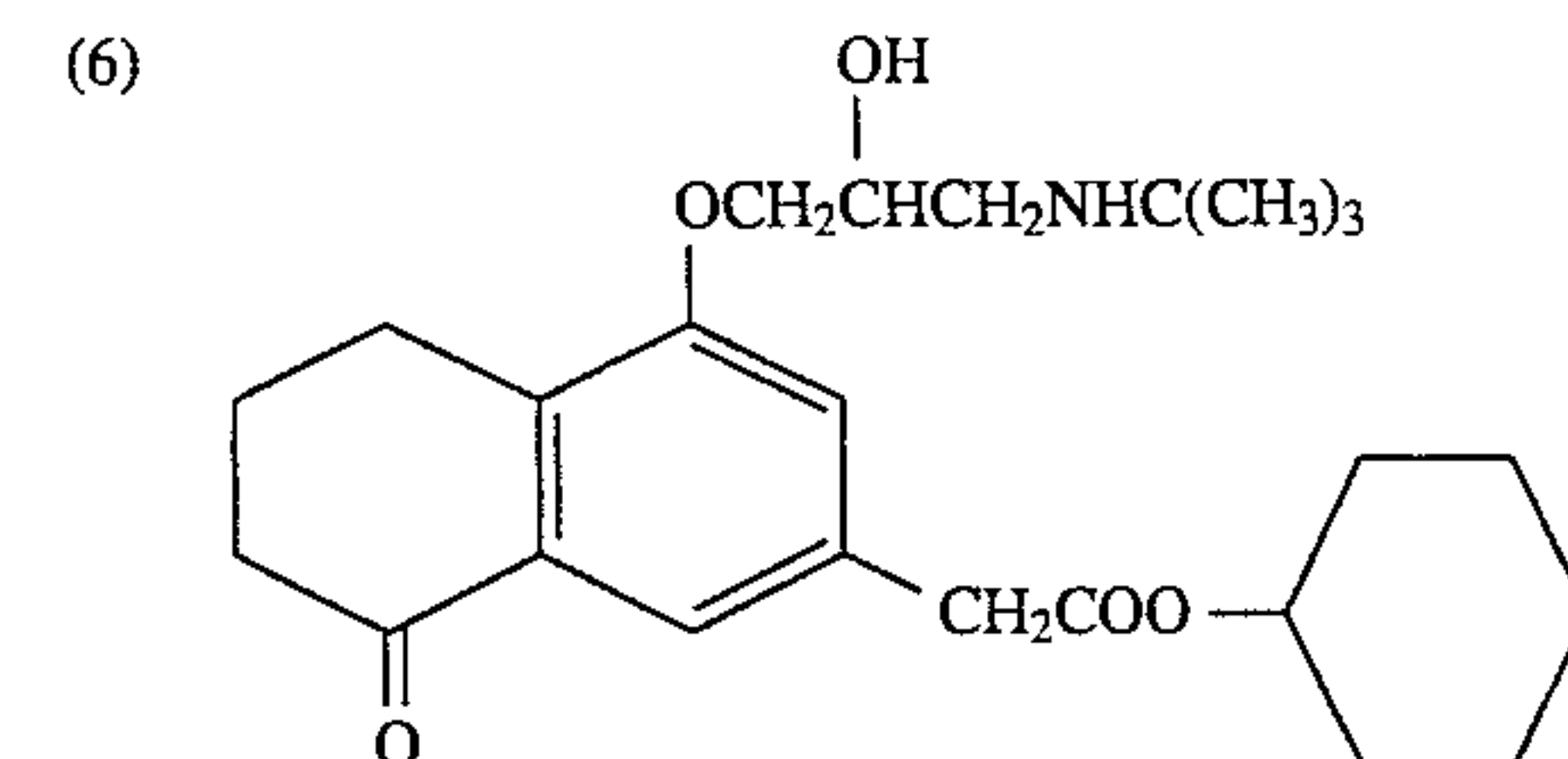
(AN ANALOGUE OF BUNOLOL)
