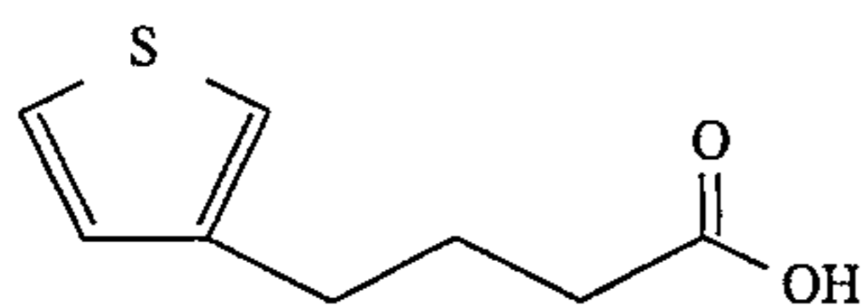
3-thiophenebutanoic acid (32)
