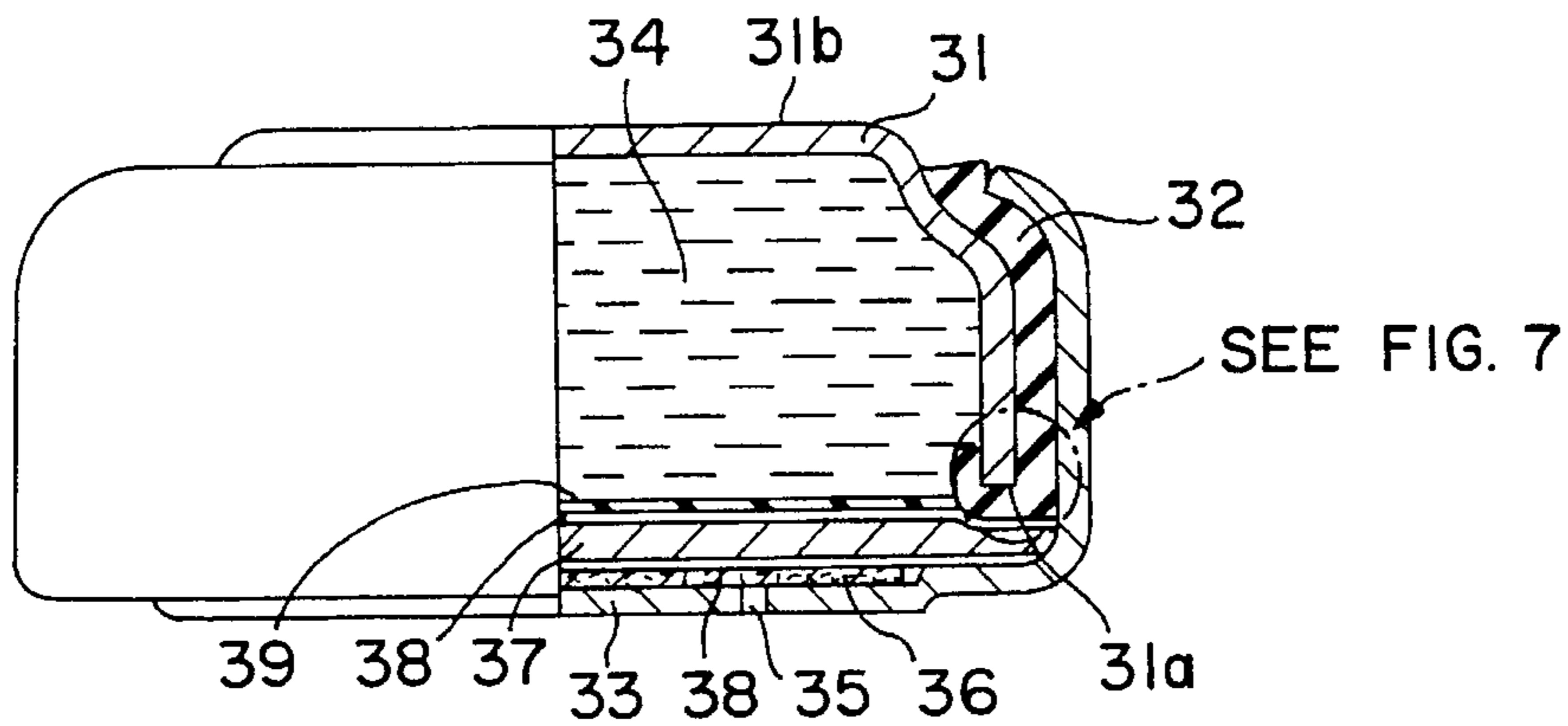
FIG. 6 (PRIOR ART)
