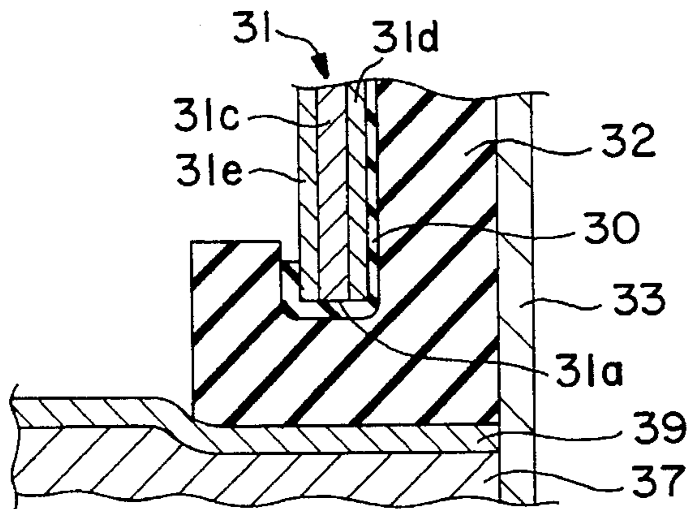
FIG. 7 (PRIOR ART)
