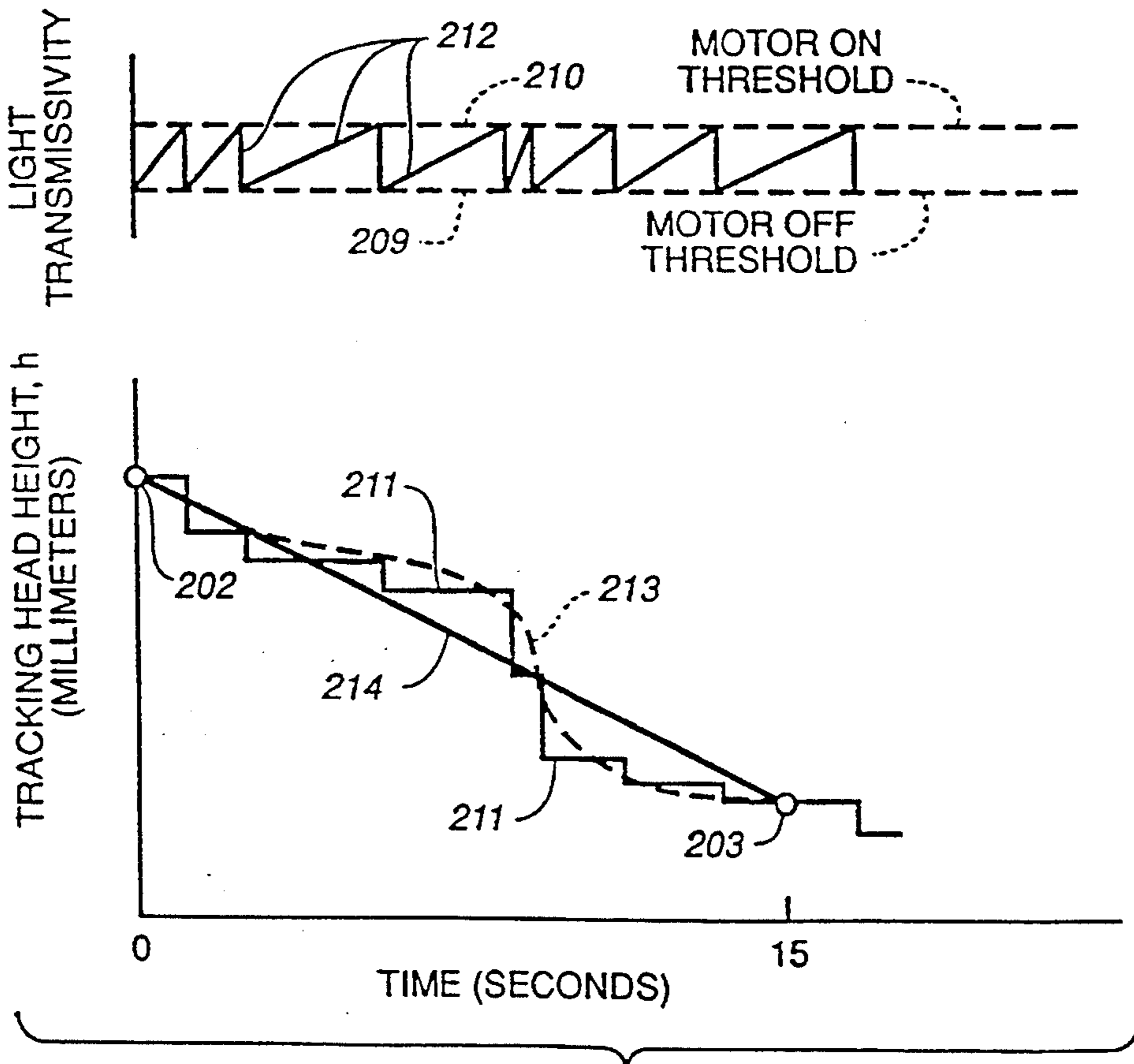
FIG. 2 (PRIOR ART)
