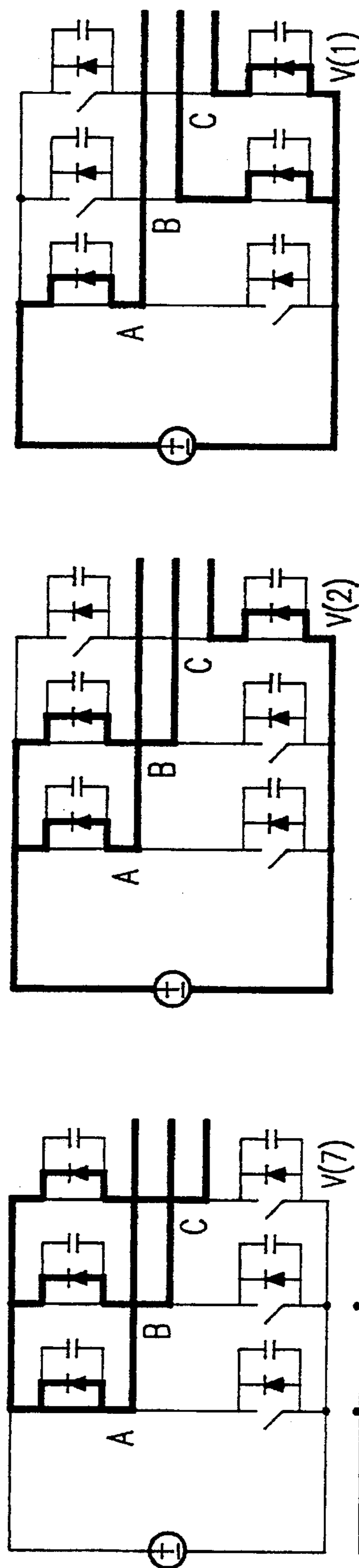
FIG. 7 Switching Sequence: V(7)-V(1)-V(2)-V(7)-
