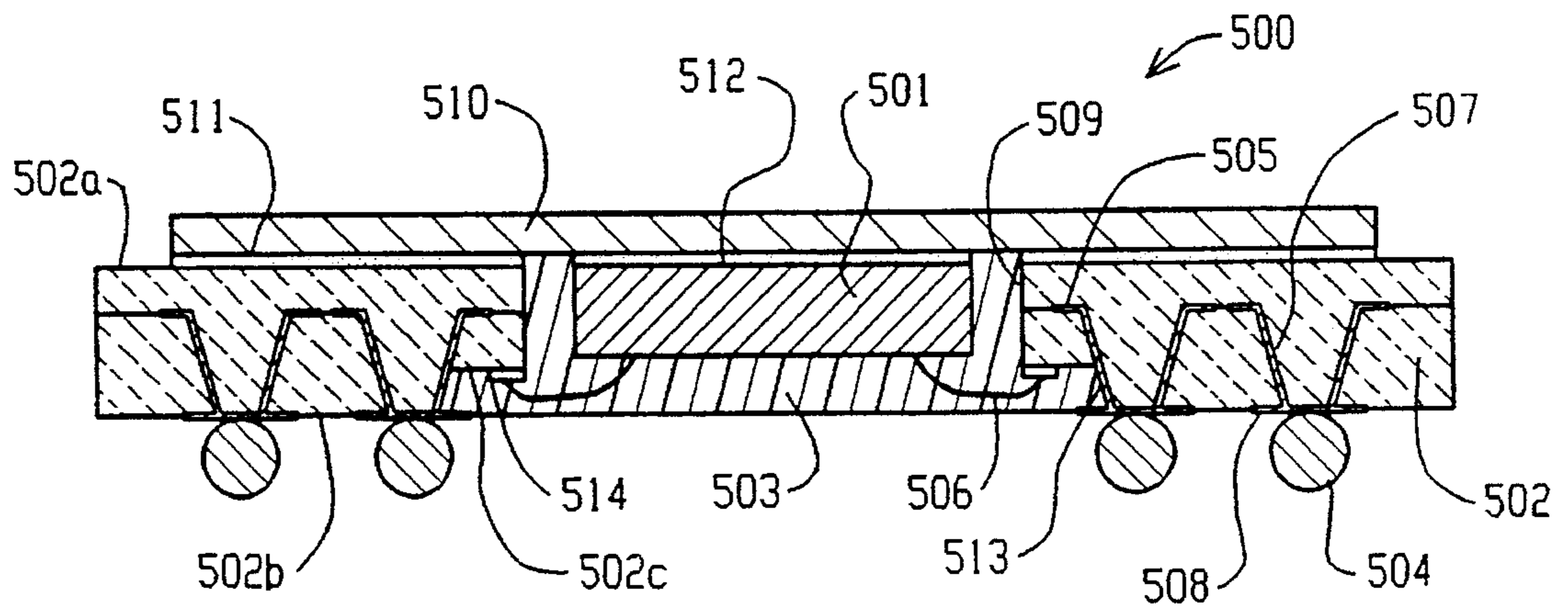
FIG. 3 (PRIOR ART)
