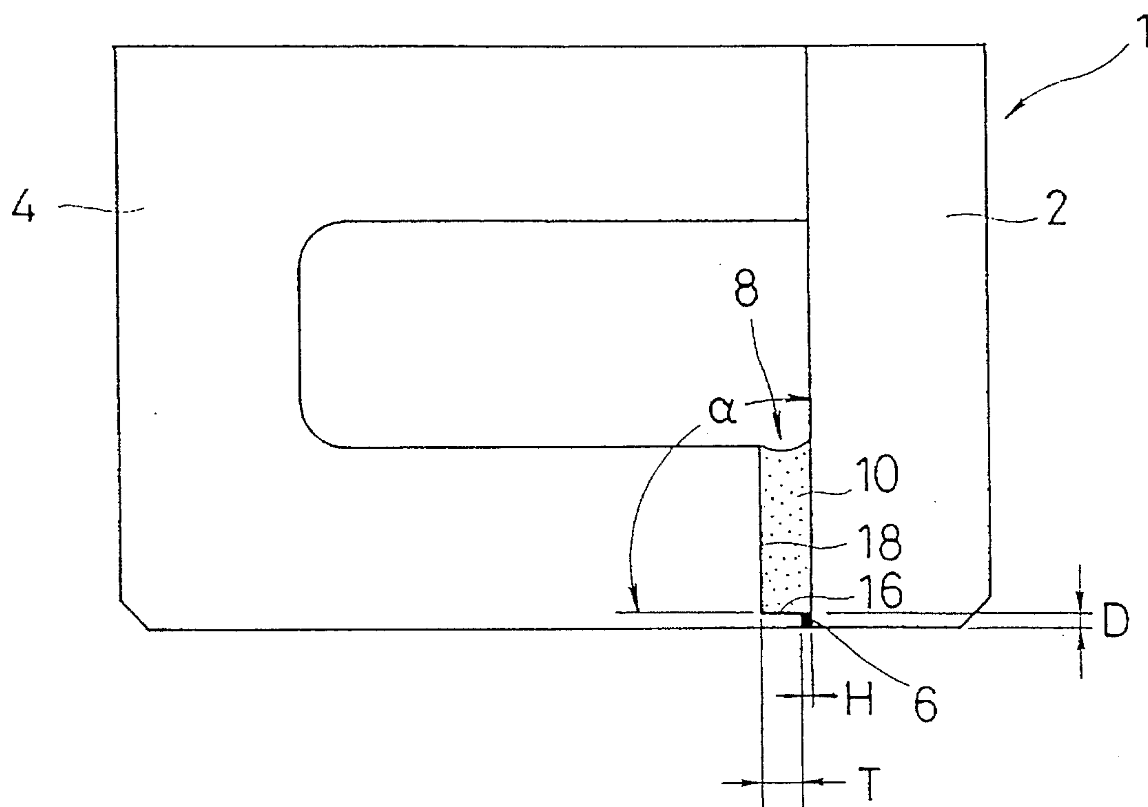
FIG. 8 PRIOR ART
