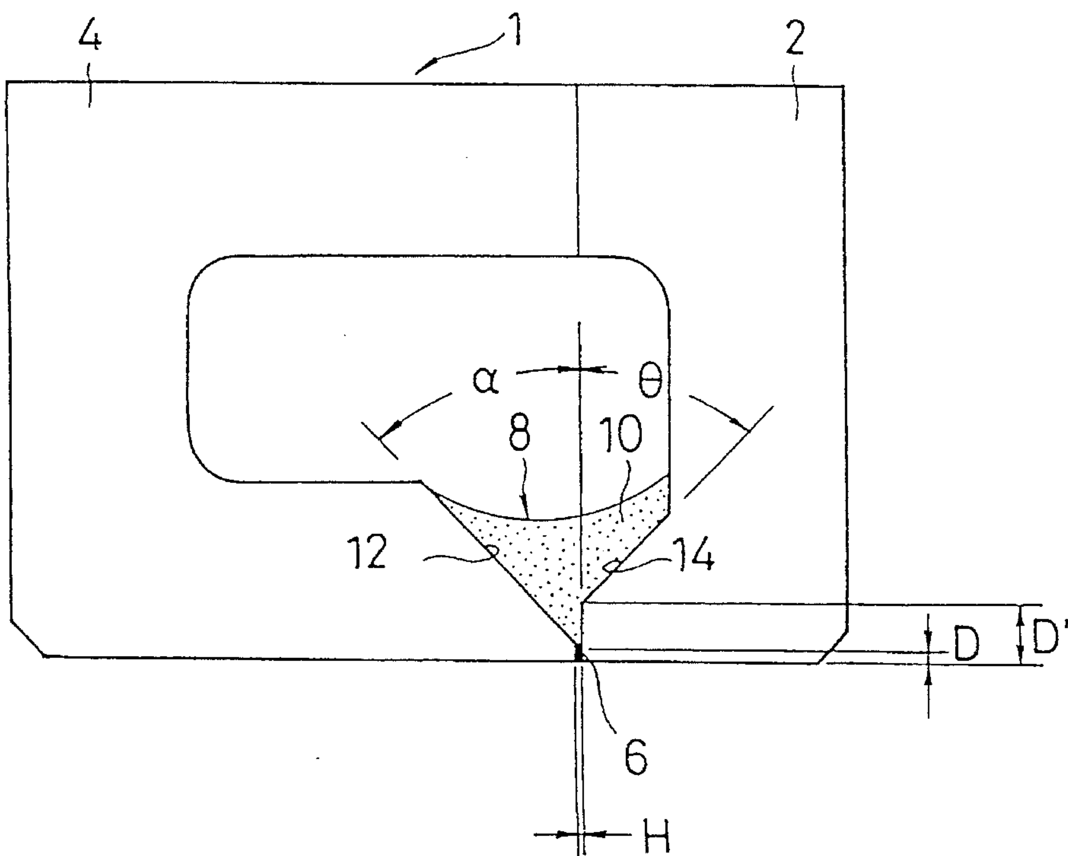
FIG. 7 PRIOR ART
