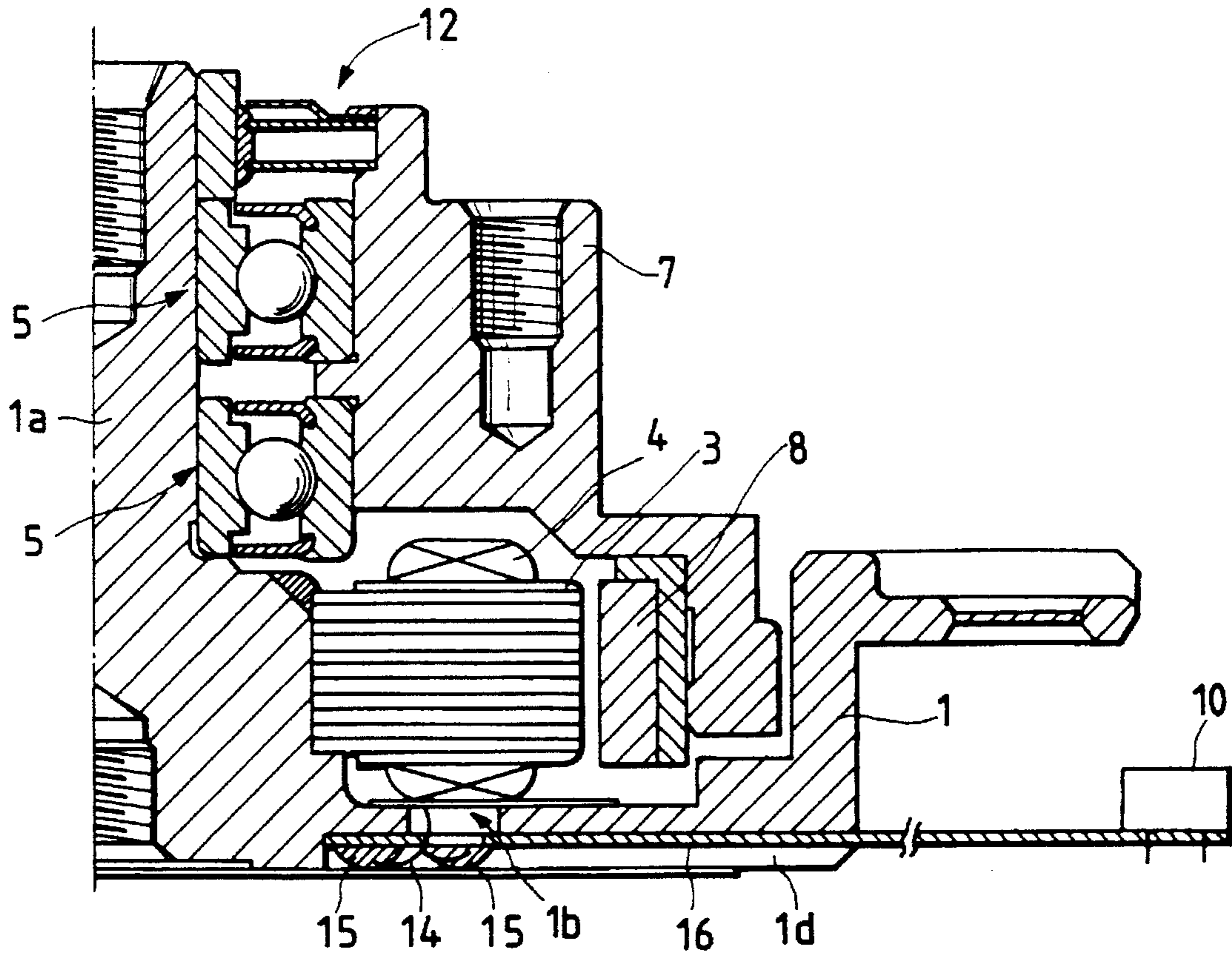
FIG. 8 PRIOR ART
