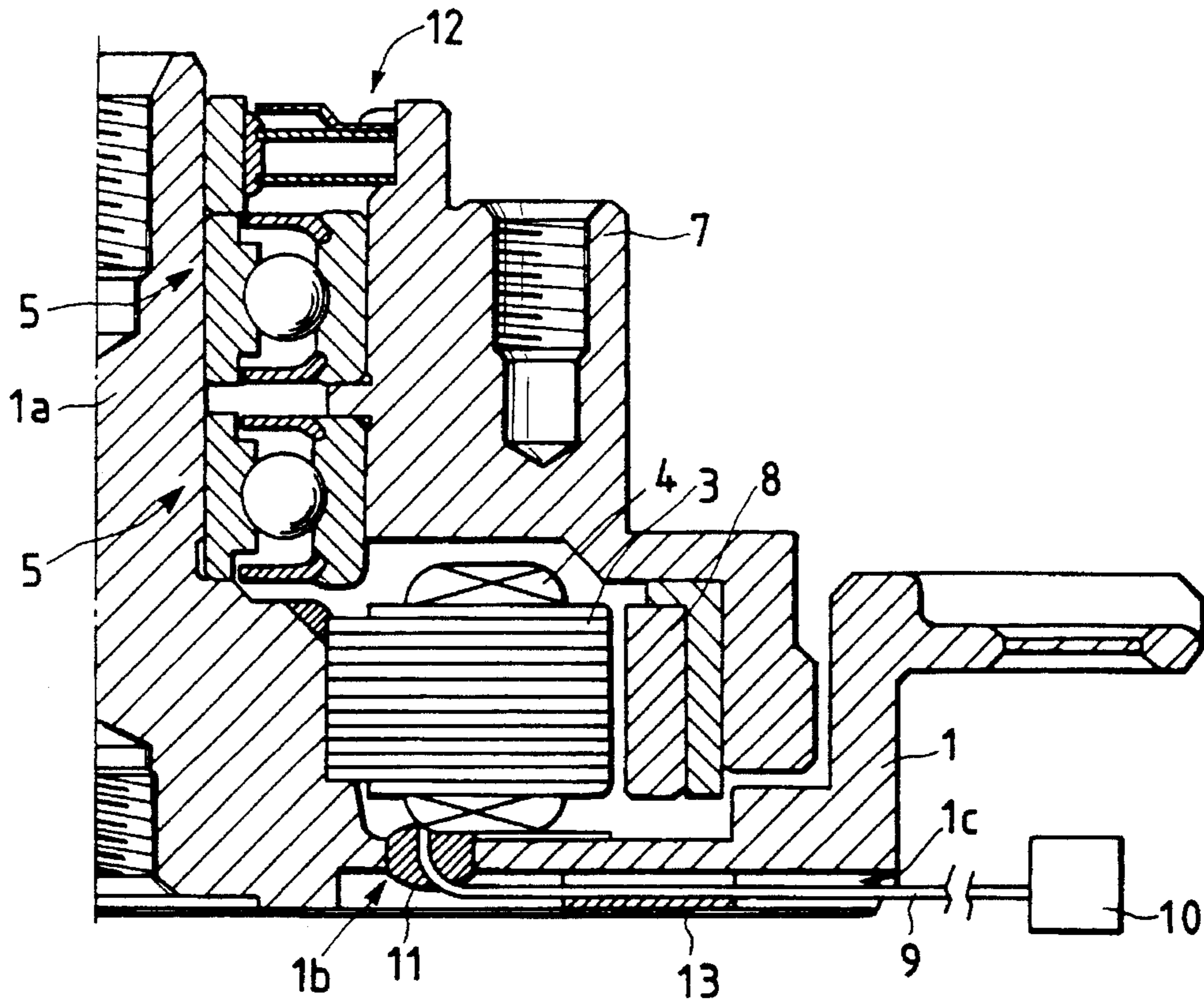
FIG. 6 PRIOR ART
