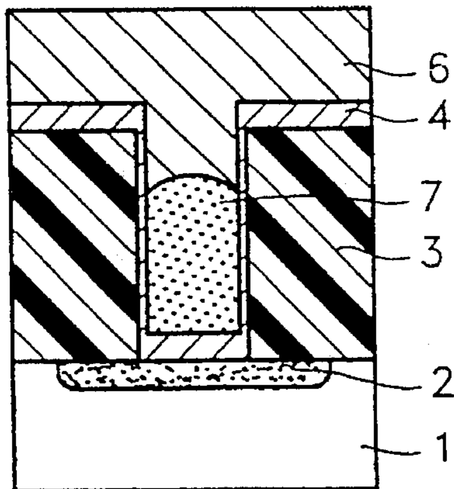
FIG. 3 (PRIOR ART)
